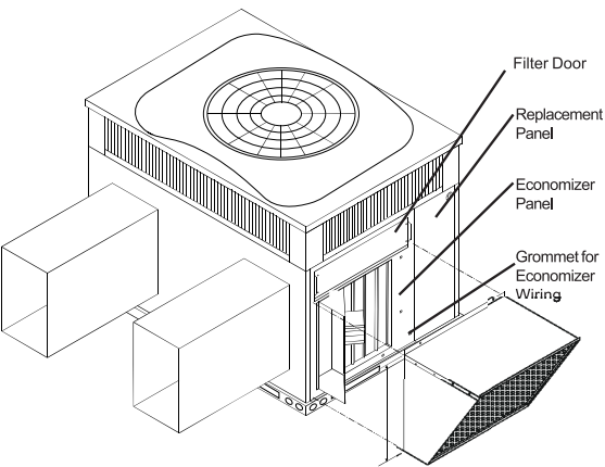
Horizontal Economizer
