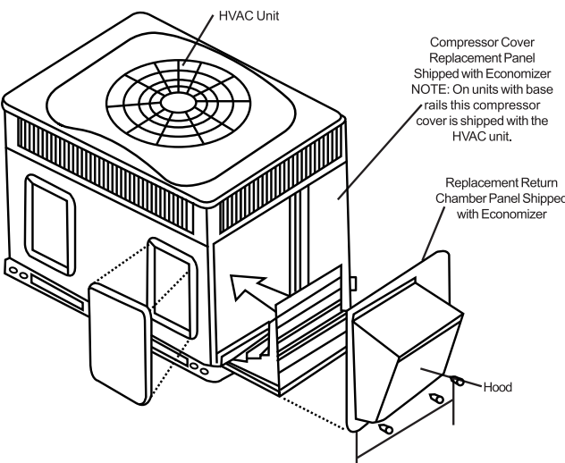
Vertical Economizer
