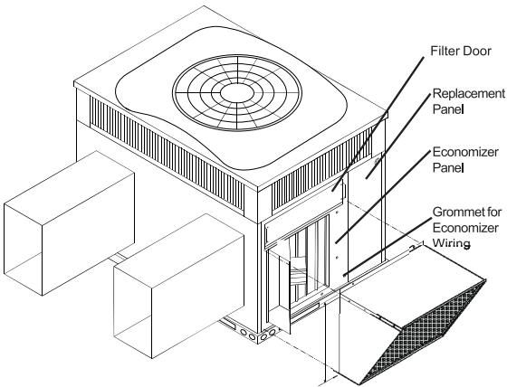
Horizontal Economizer
