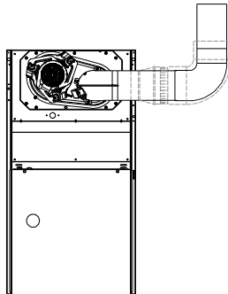
Upflow Application-Vent Elbow Up
