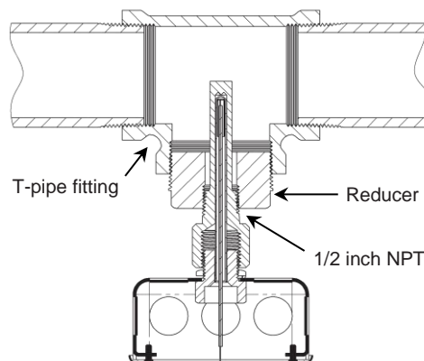
Figure 7: Typical T-Mount
