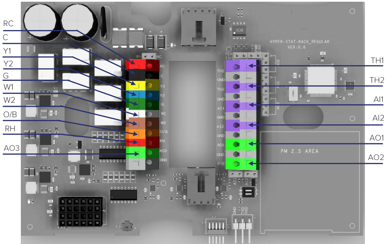
INTERFACE PCB
