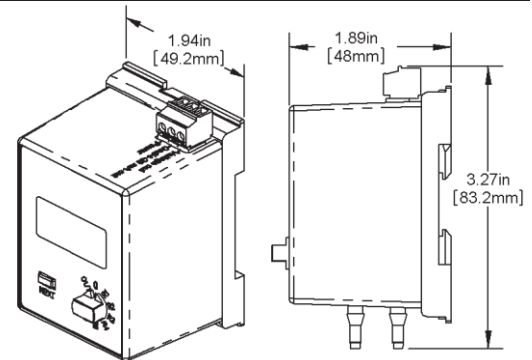
Figure 1: Pressure Sensor
