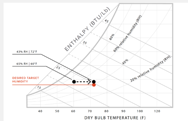
This psychrometric chart indicates that air which is 60°F with 65% humidity will end up with 43% humidity when heated to 72°F.
