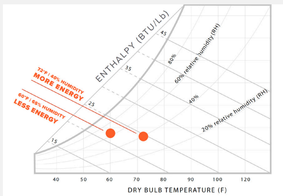
This psychrometric chart indicates that air which is 72°F with 40% humidity has more energy than air which is 60°F with 65% humidity.
