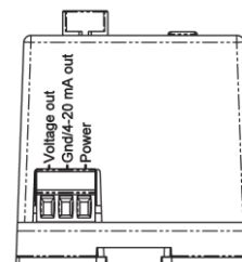
Figure 7: Wiring terminations
