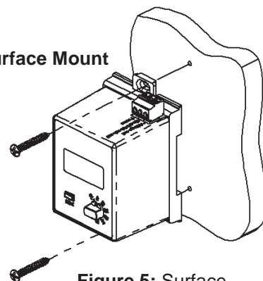
Figure 5: Surface mounting with the tabs out.
