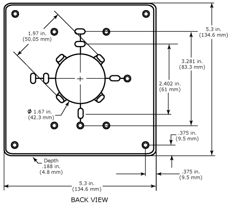
Figure 5: Part #NSB-ADP-53-53
