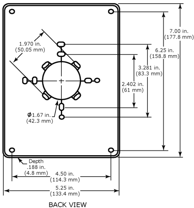
Figure 4: Part #NSB-ADP-525-7
