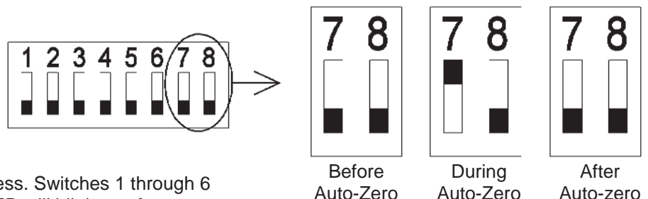
Figure 6: Auto-Zero Switch 7
