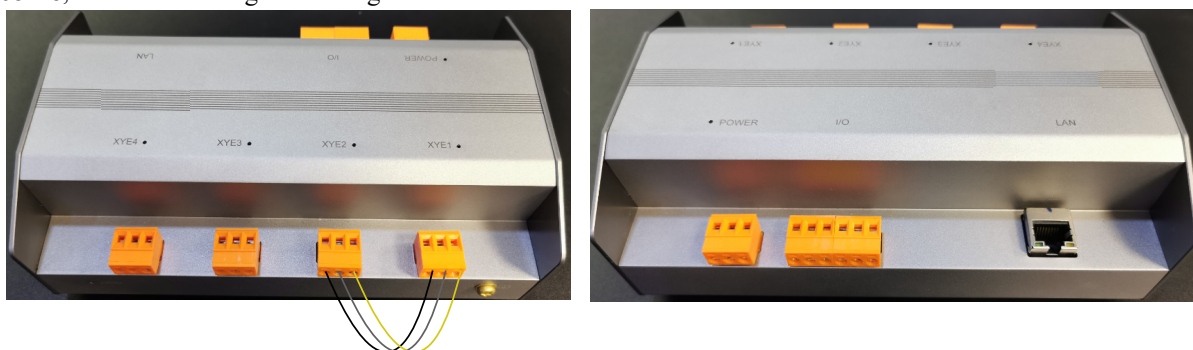
Fig. 17 —Connect XYE Port 0 and Port 1
