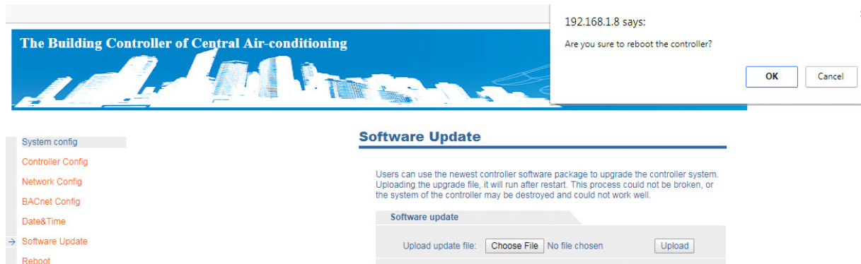
Fig. 16 —Reboot Confirmation
