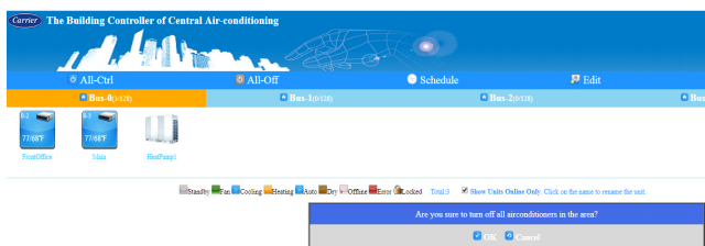
Fig. 28 —All-Off
