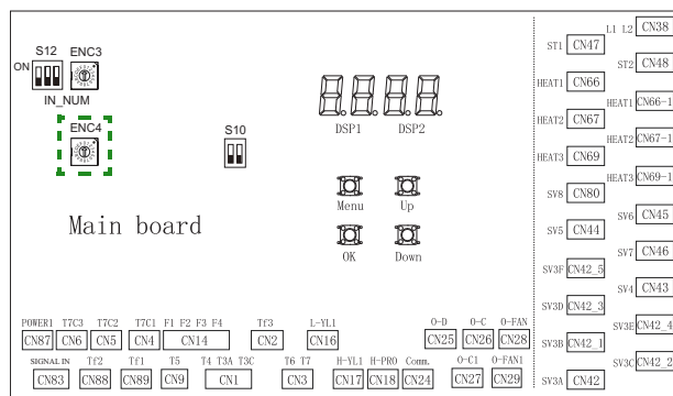
Fig. 5 —Heat Recovery ENC4
