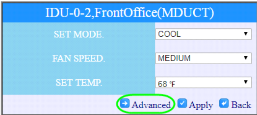
Fig. 22 —Click Advanced
