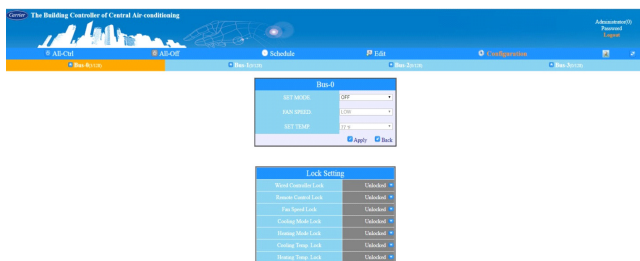
Fig. 27 —All-Ctrl
