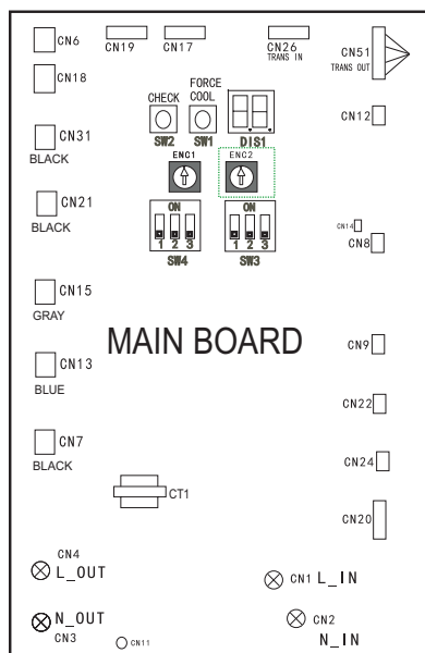
Fig. 6 —Single Phase Heat Pump ENC2
