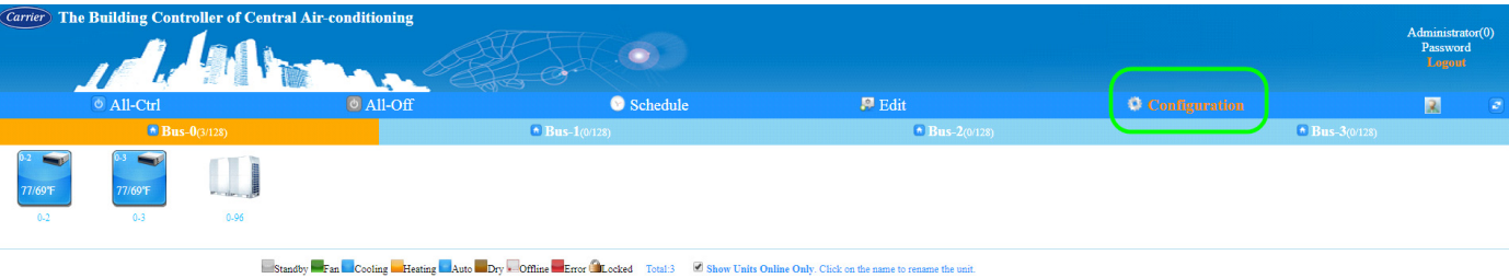
Fig. 10 —Configuration Icon
