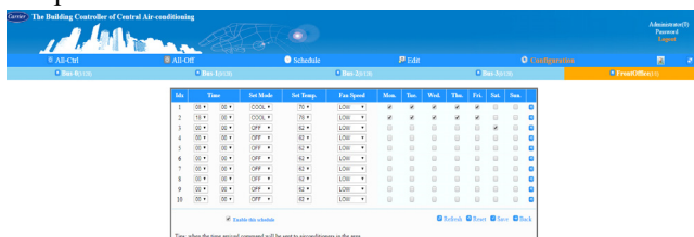
Fig. 29 —Schedule
