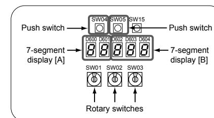
Interface PC board
