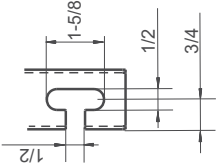
Detail of Z section
