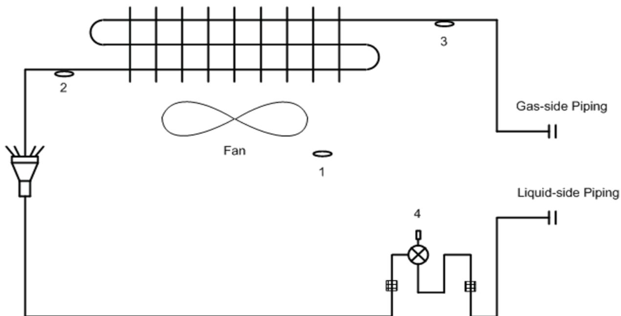
Fig. 1 —Piping
