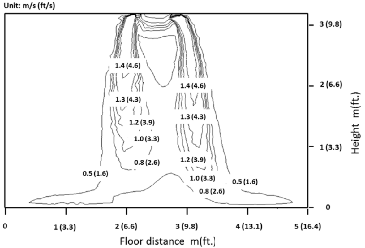
Fig. 4 —Cooling Velocity
