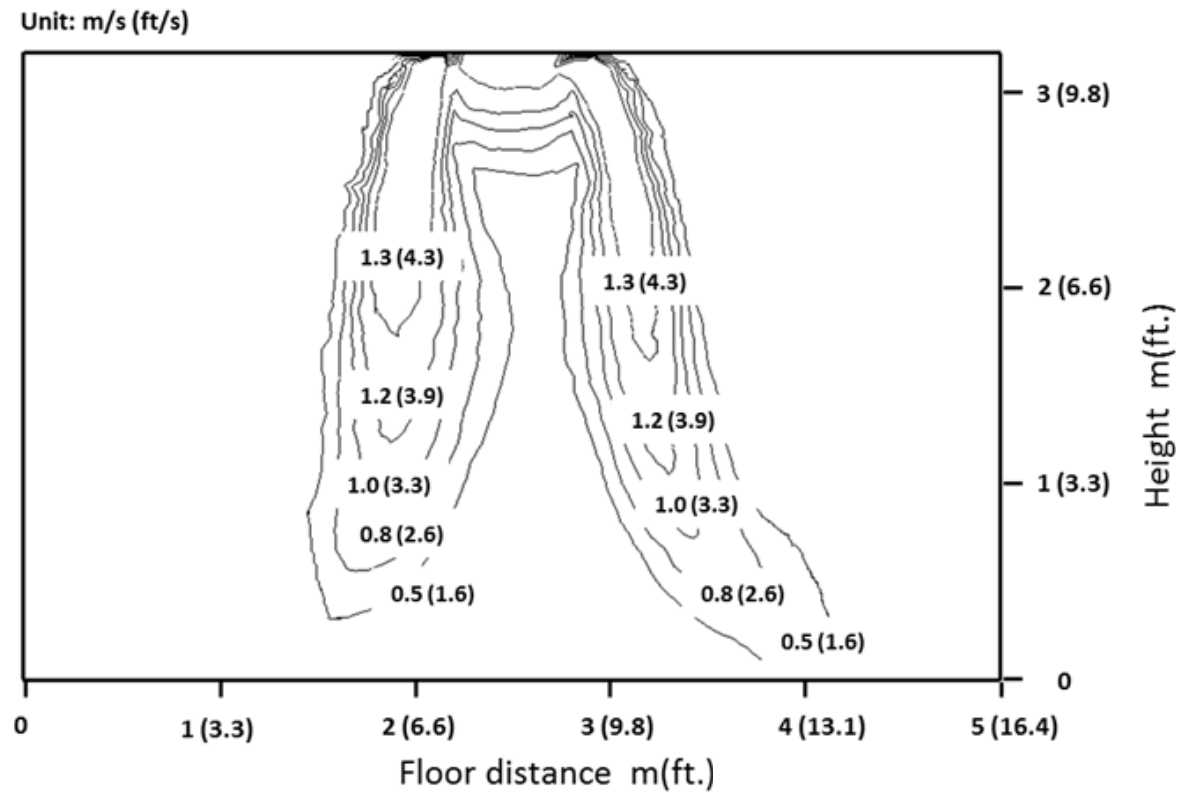
Fig. 5 —Heating Velocity
