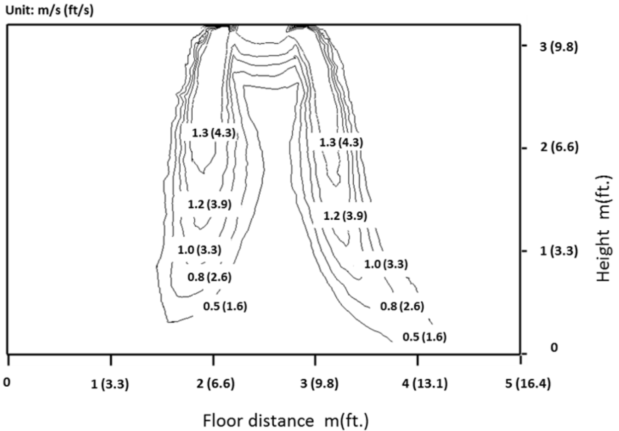
Fig. 9 —Heating mode with 60°swing
