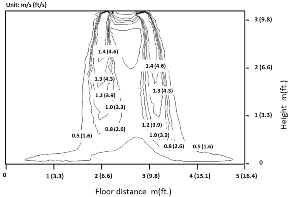
Fig. 8 —Cooling mode with 60°swing
