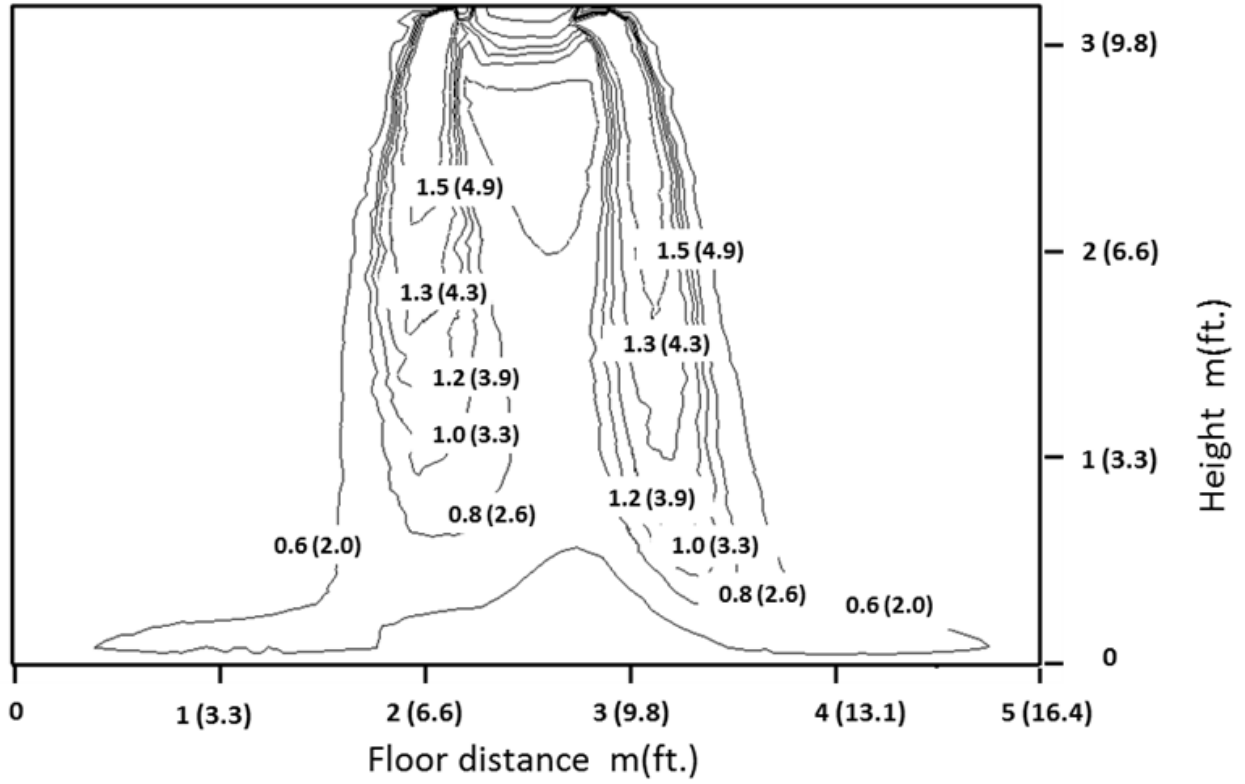
Fig. 12 —Cooling mode with 60°swing
