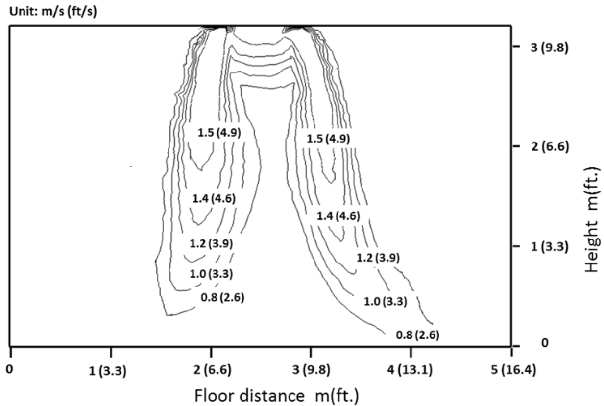
Fig. 19 —Heating mode with 60°swing
