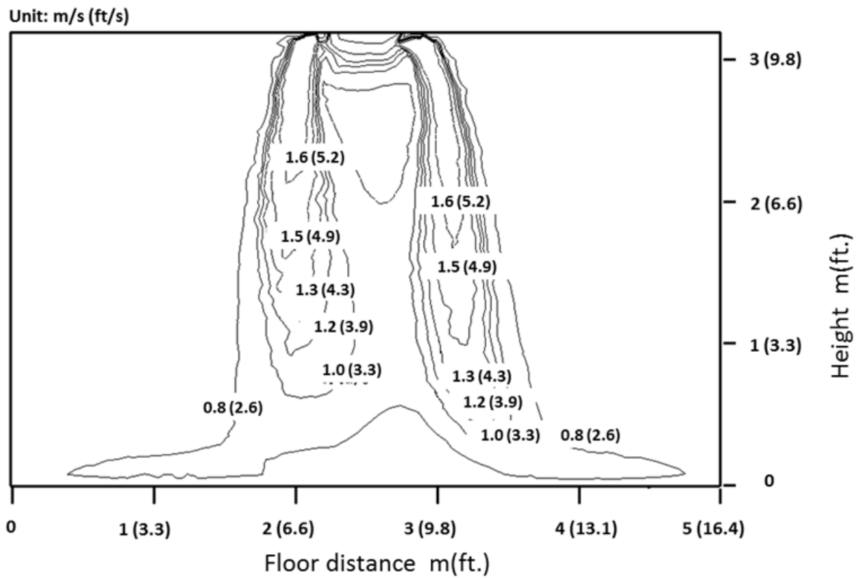
Fig. 18 —Cooling mode with 60°swing
