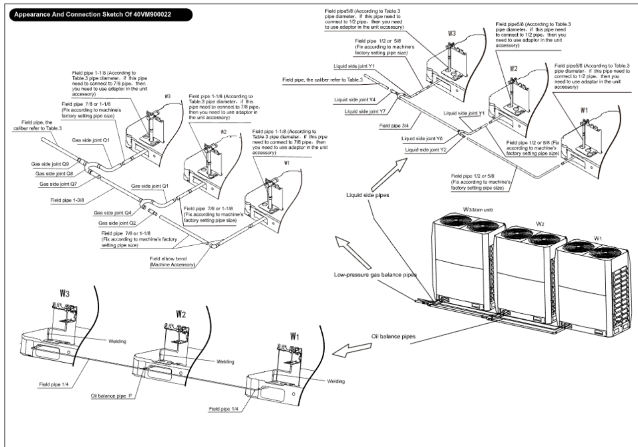
Figure 29 - Appearance and Connection Sketch of 40VM900022
