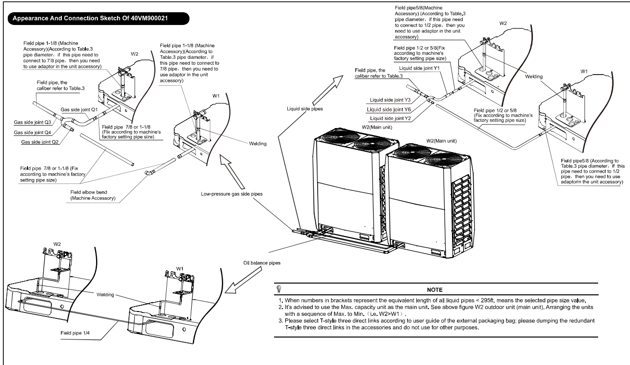
Figure 28 - Appearance and Connection Sketch of 40VM900021
