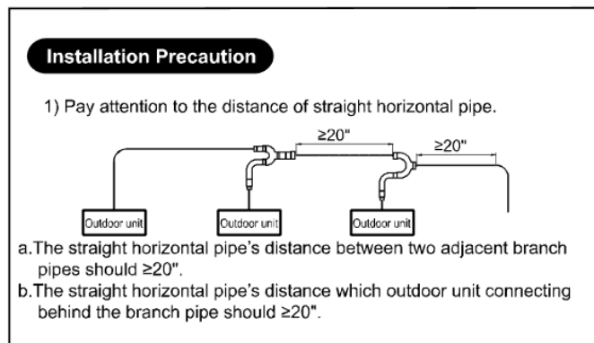
Figure 26 - Installation Precautions (ODU)
