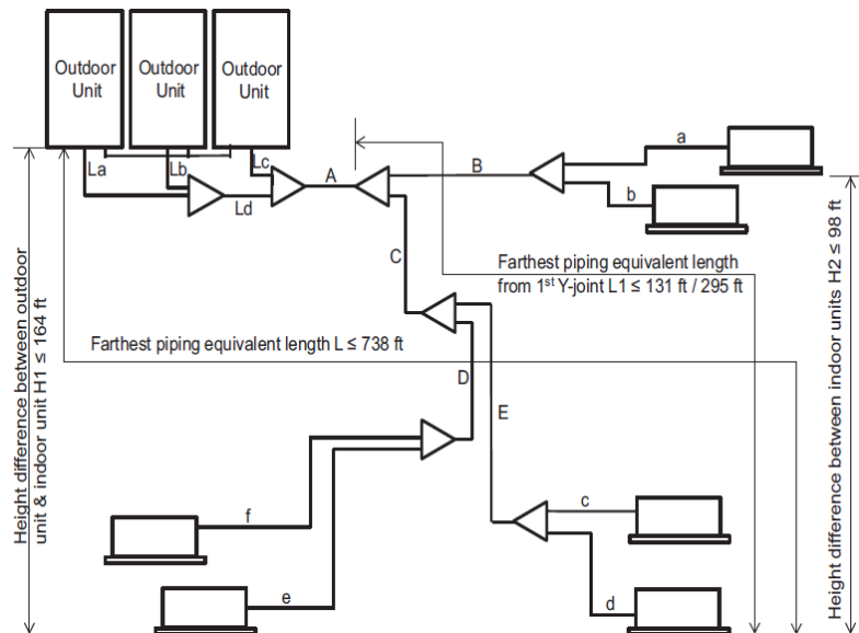
Figure 22 - Piping Lengths and Drop Height
