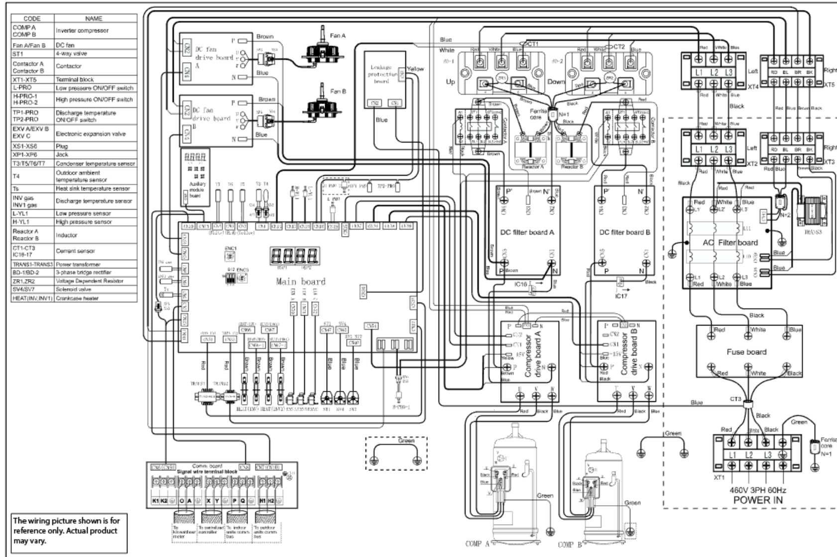
Figure 8 - 38VMA144HDS6-1
