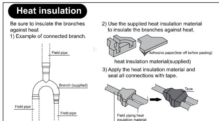
Figure 25 - Heat Insulation (IDU)
