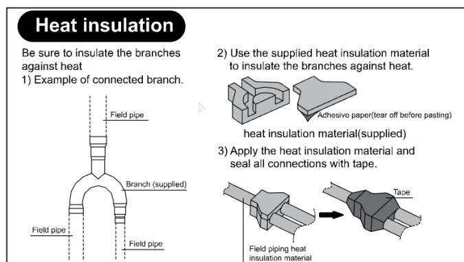
Figure 27 - Heat Insulation (ODU)
