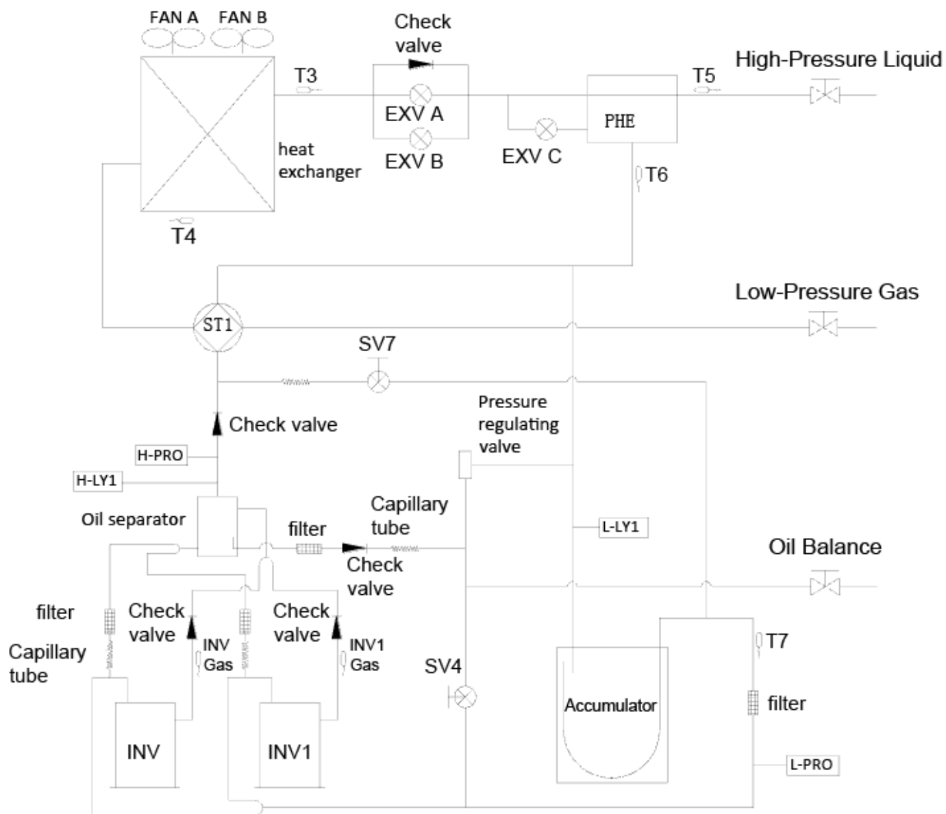
Figure 4 - Refrigerant Circuit Diagram (38VMA144HDS*-1)
