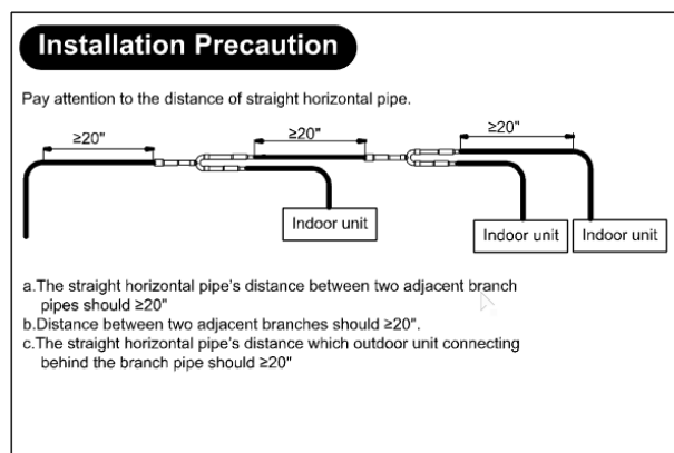
Figure 24 - Installation Precautions (IDU)
