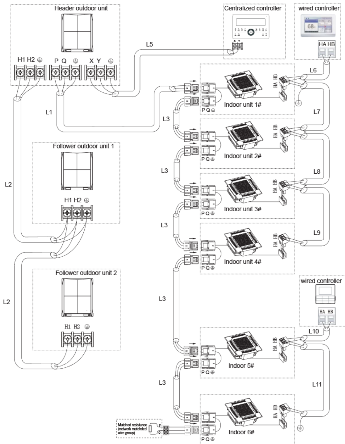
Figure 9 - Field Wiring
