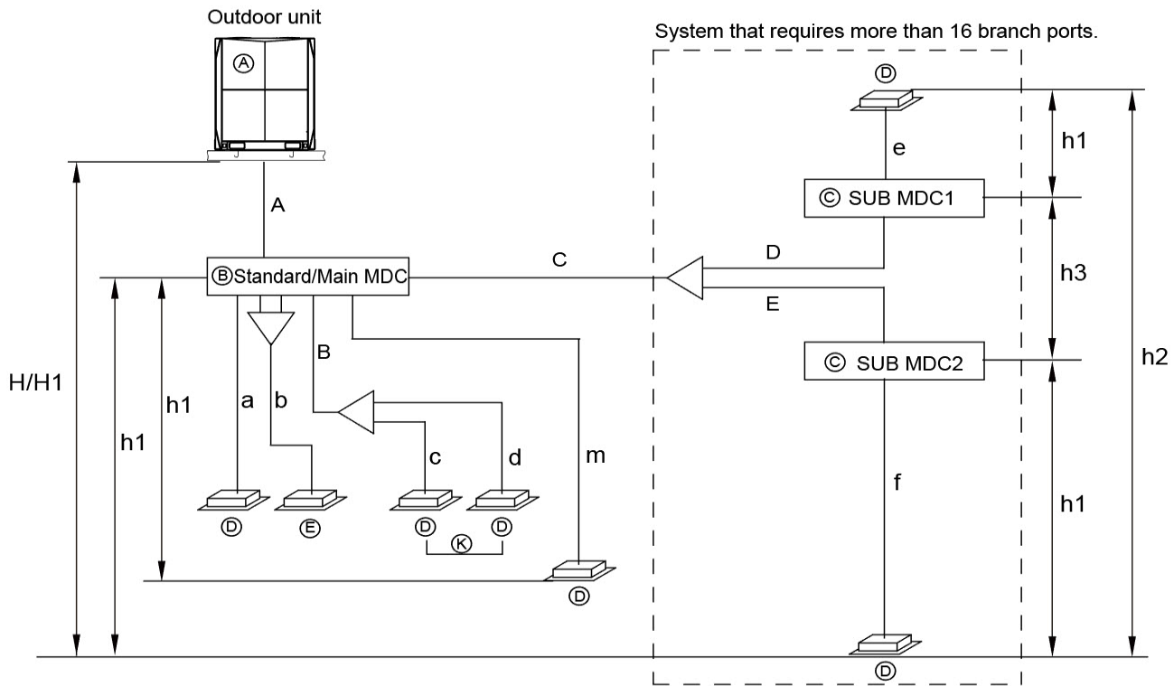
Fig. 46 —Piping Lengths and Drop Heights
