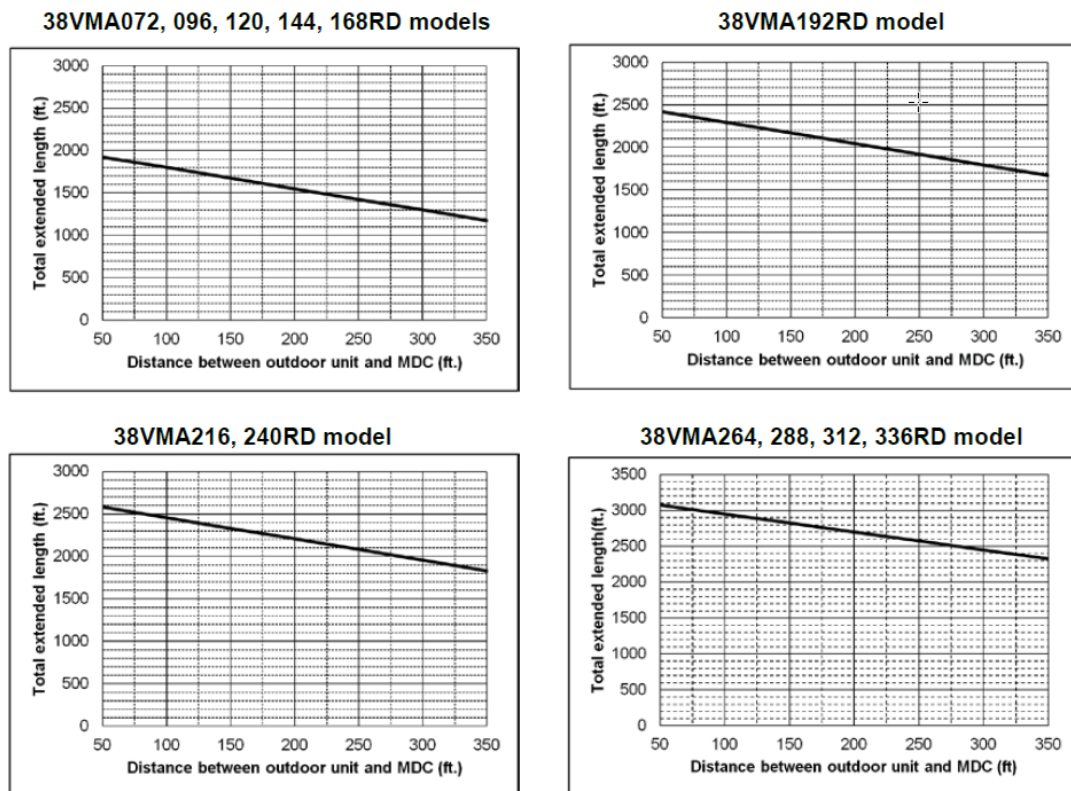
Fig. 49 —Total Piping Length Restrictions
