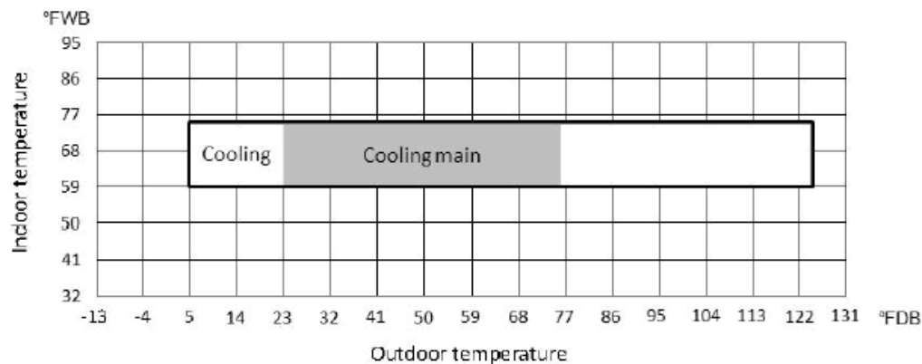
Fig. 52 —Temperature Operation Limits – Cooling
