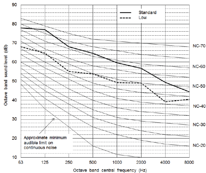
Fig. 43 —38VMA312RDS6-1
