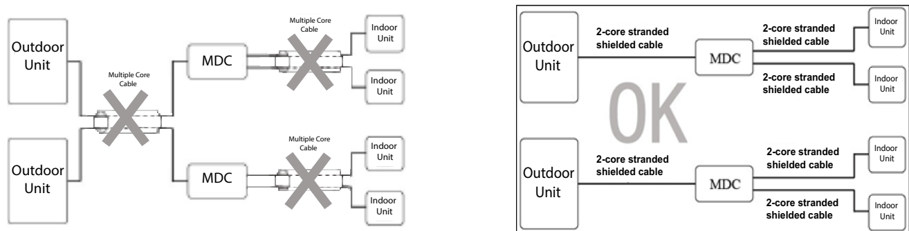
Fig. 14 —2-Core Stranded Shielded Cables
