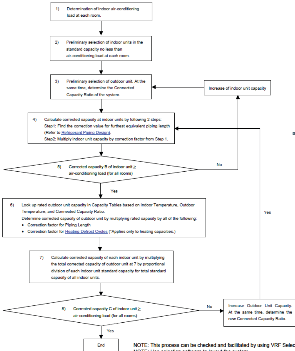
Fig. 50 —Selection Flow Chart
