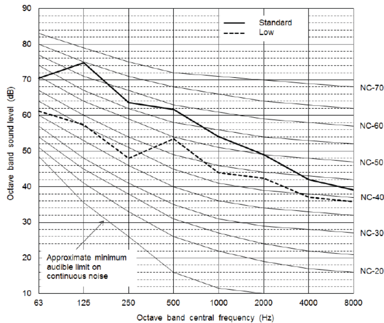
Fig. 31 —38VMA192RDS6-1
