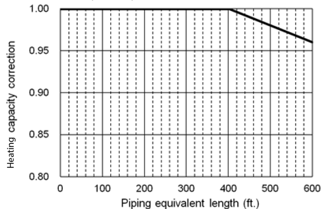
38VMA312RDS5-1(RDS6-1)
