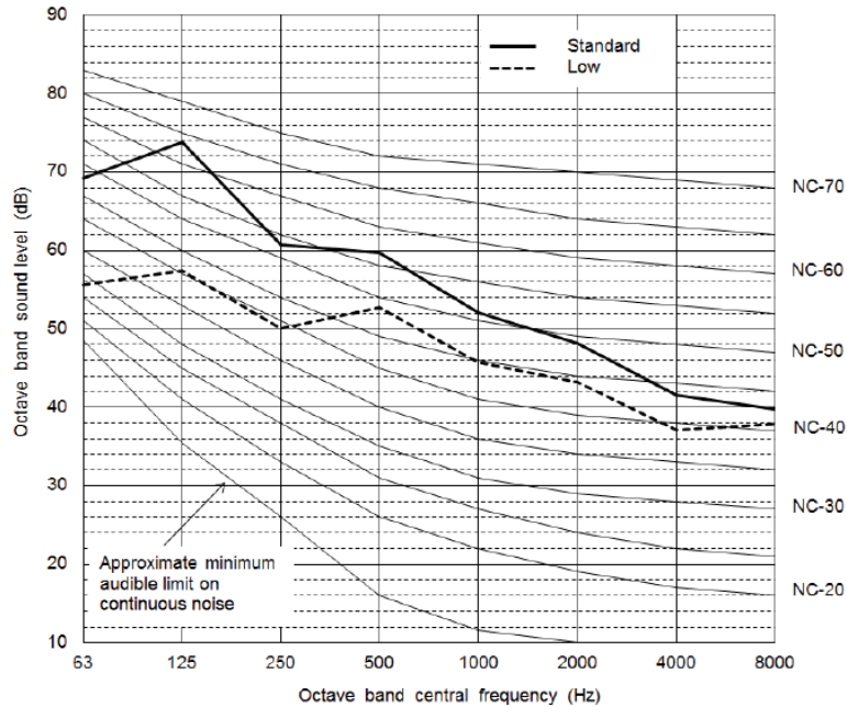
Fig. 29 —38VMA168RDS6-1
