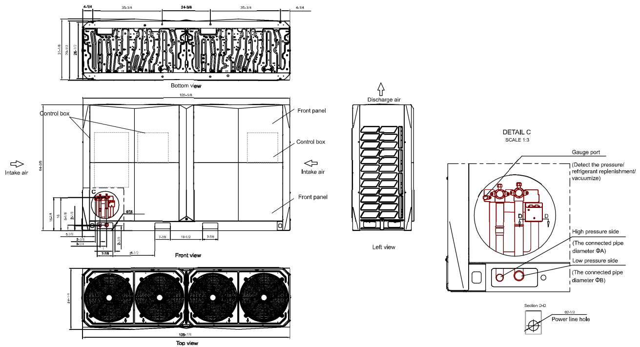
Fig. 6 —38VMA240RDL, 38VMA264, 288, 312, 336RDS Models
