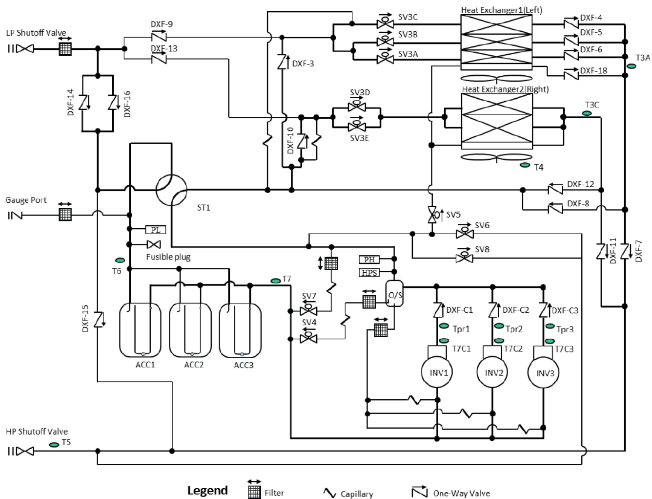
Fig. 9 —38VMA240RDL, 264, 288, 312, 336RDS models
