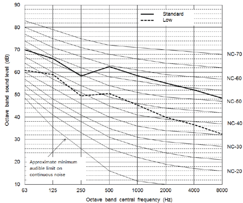
Fig. 25 —38VMA120RDS6-1
