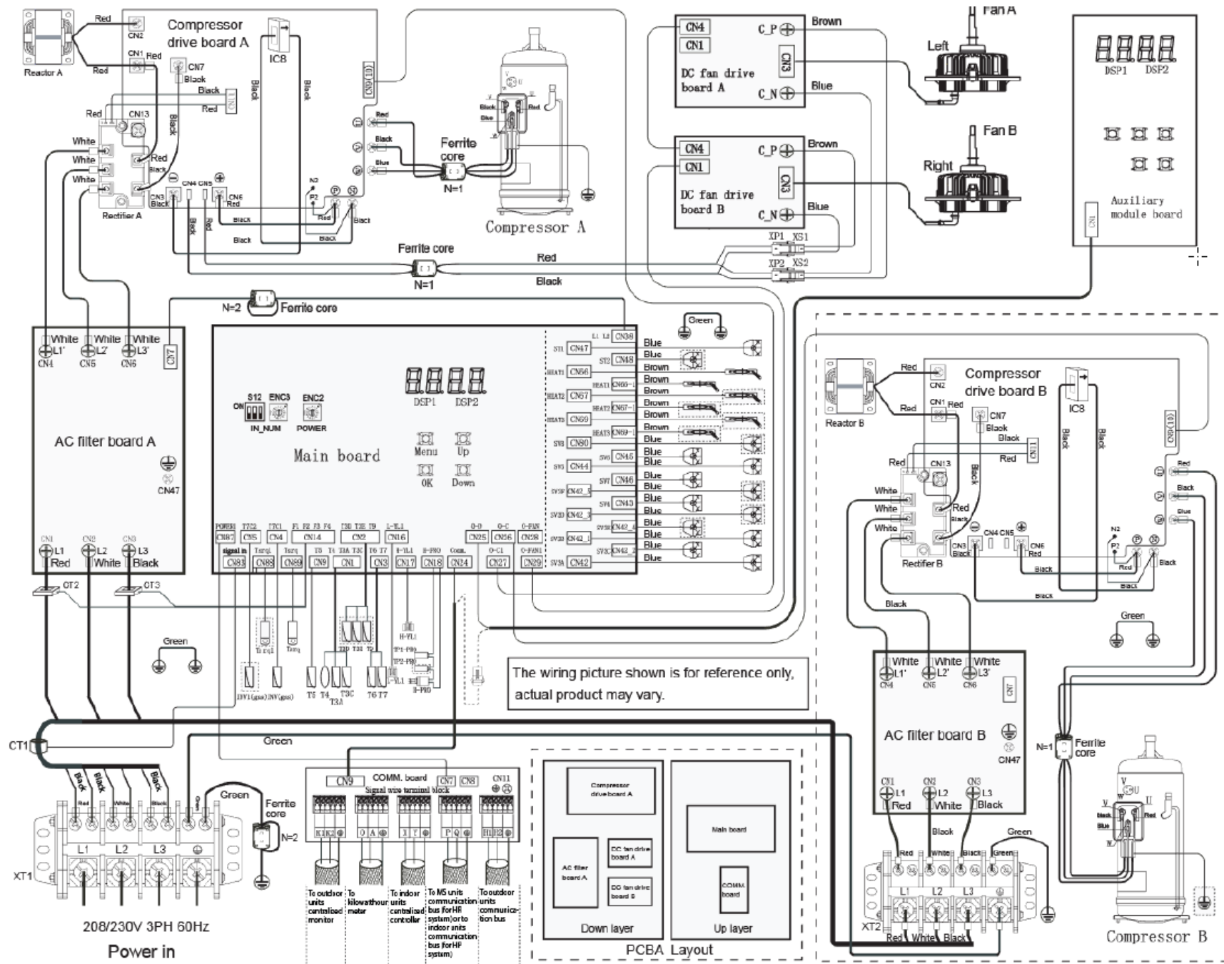
Fig. 12 —38VMA072, 096, 120RDS6-1, 38VMA144RDL6-1, 38VMA168, 192, 216, 240RDS6-1
