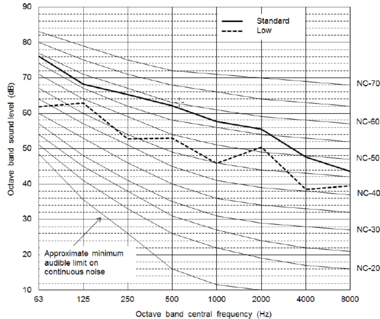
Fig. 37 —38VMA240RDL6-1
