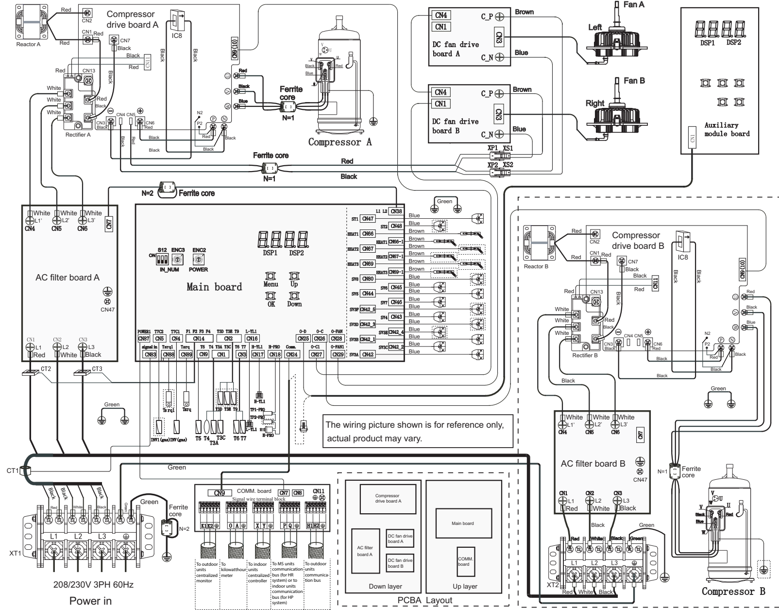
Fig. 10 —38VMA072, 096, 120RDS5-1, 38VMA144RDL5-1, 38VMA168, 192, 216, 240RDS5-1
