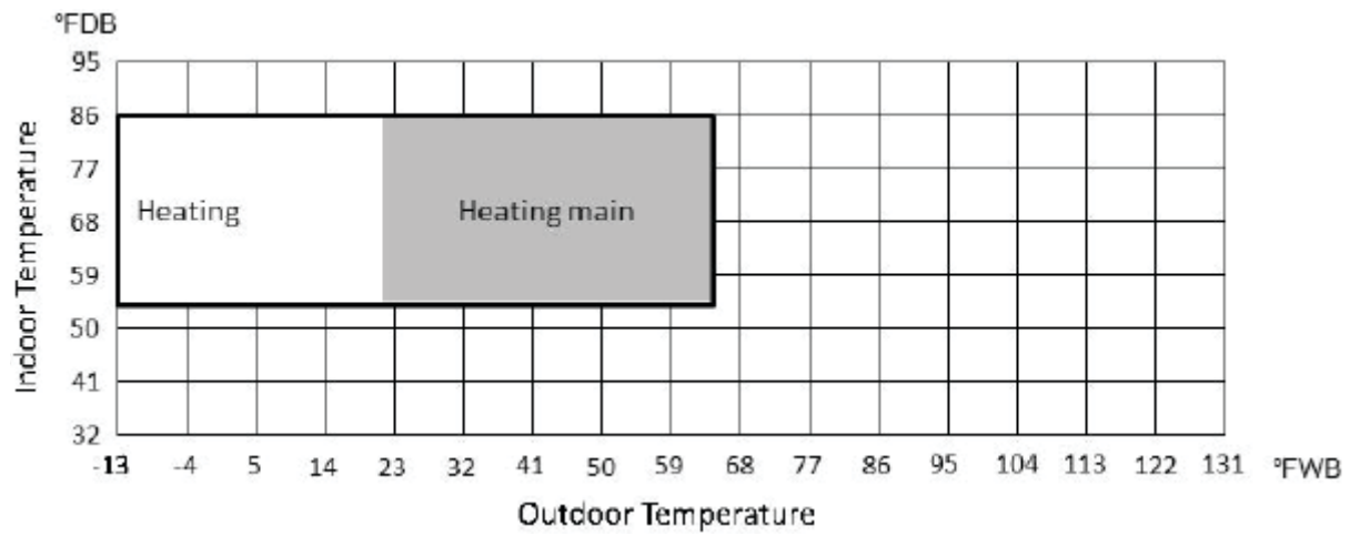
Fig. 53 —Temperature Operation Limits – Heating
