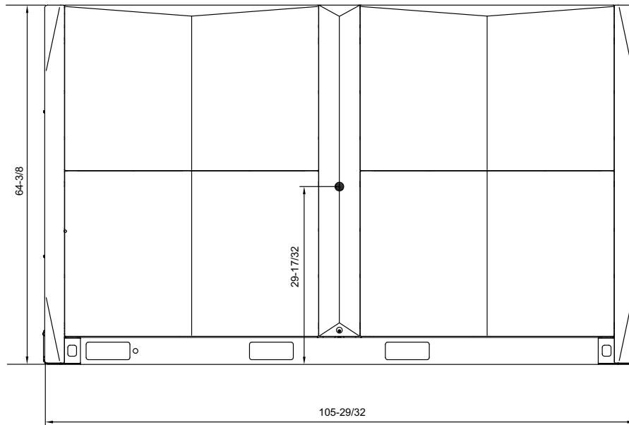
Fig. 2 —38VMA144RDL, 38VMA168, 192, 216, 240RDS Models
