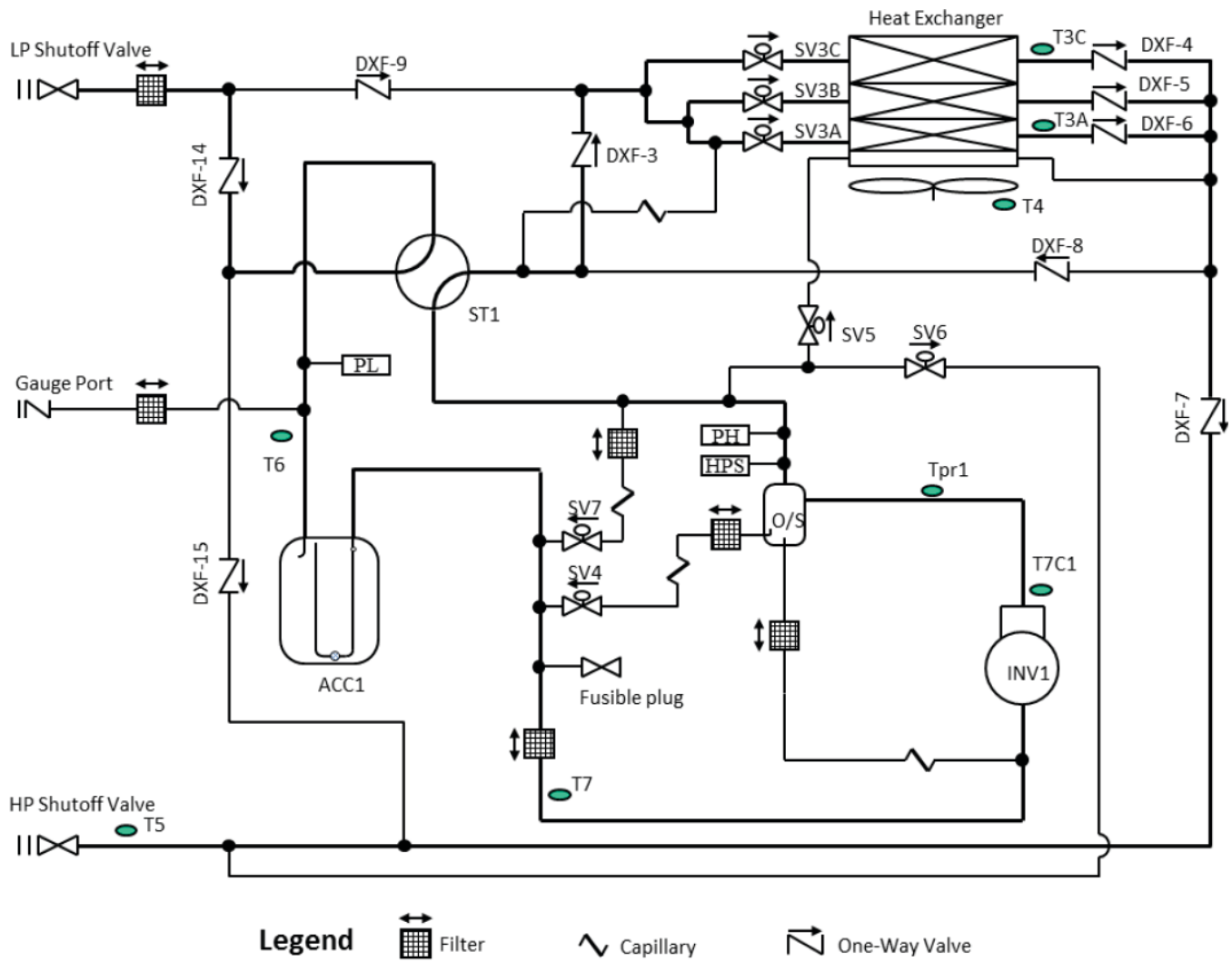
Fig. 7 —38VMA072, 096, 120RDS Models
