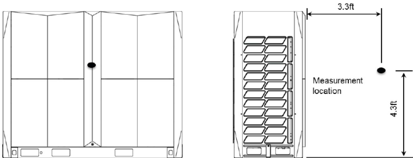
Fig. 18 —38VMA144RDL, 38VMA168, 192, 216, 240RDS Models
