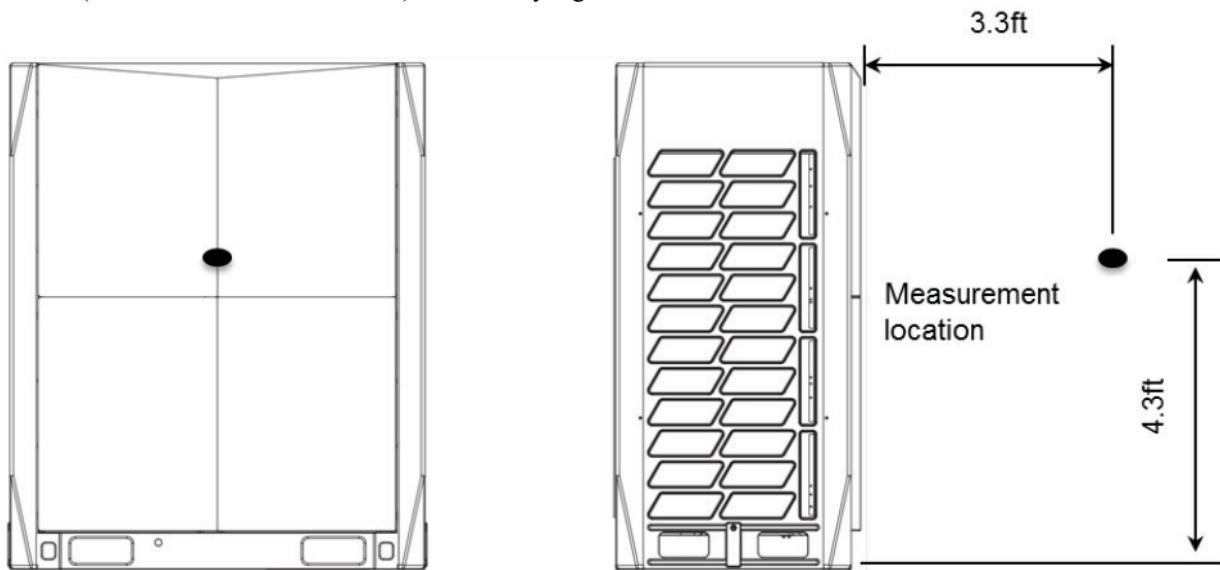
Fig. 17 —38VMA072, 096, 120RDS Models
