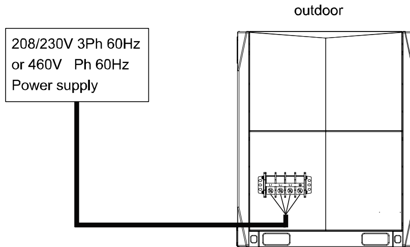
Fig. 15 —Main Power Wiring for Outdoor Unit
