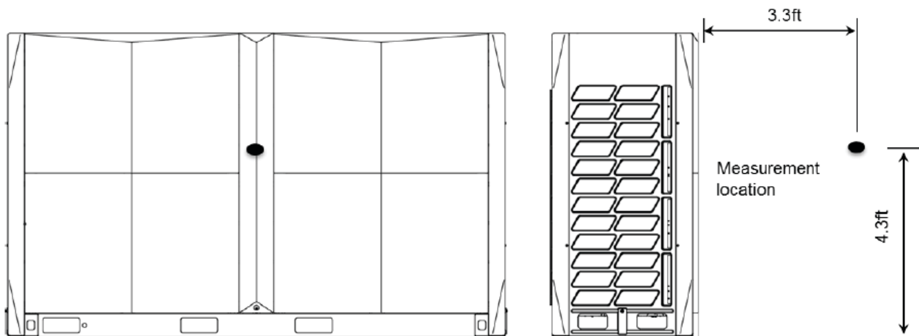
Fig. 19 —38VMA240RDL, 38VMA264, 288, 312, 336RDS Models
