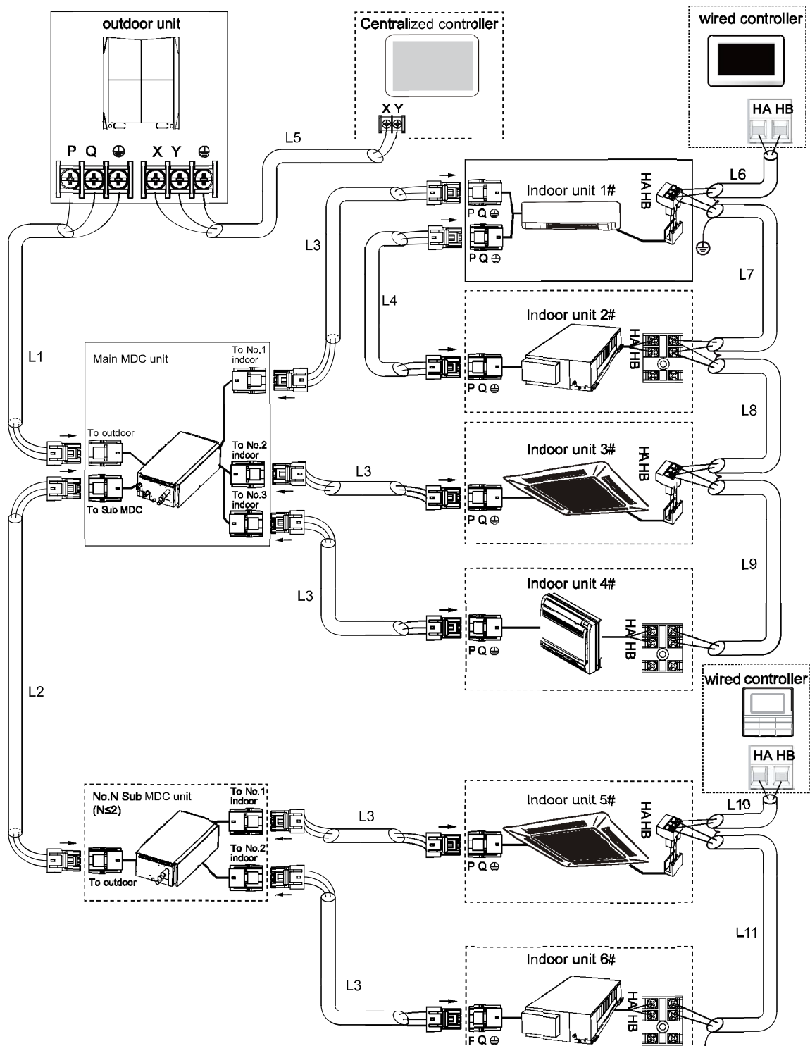
Fig. 16 —Controls Wiring
