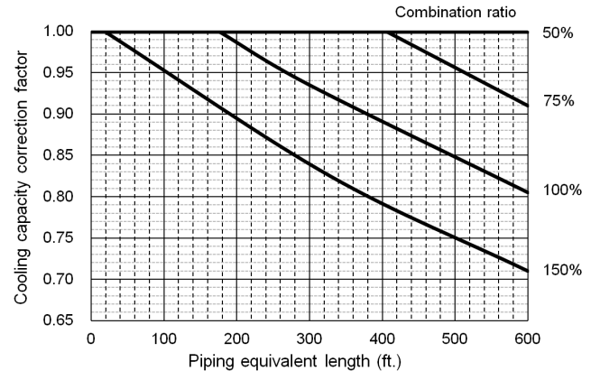
38VMA264RDS5-1(RDS6-1)
