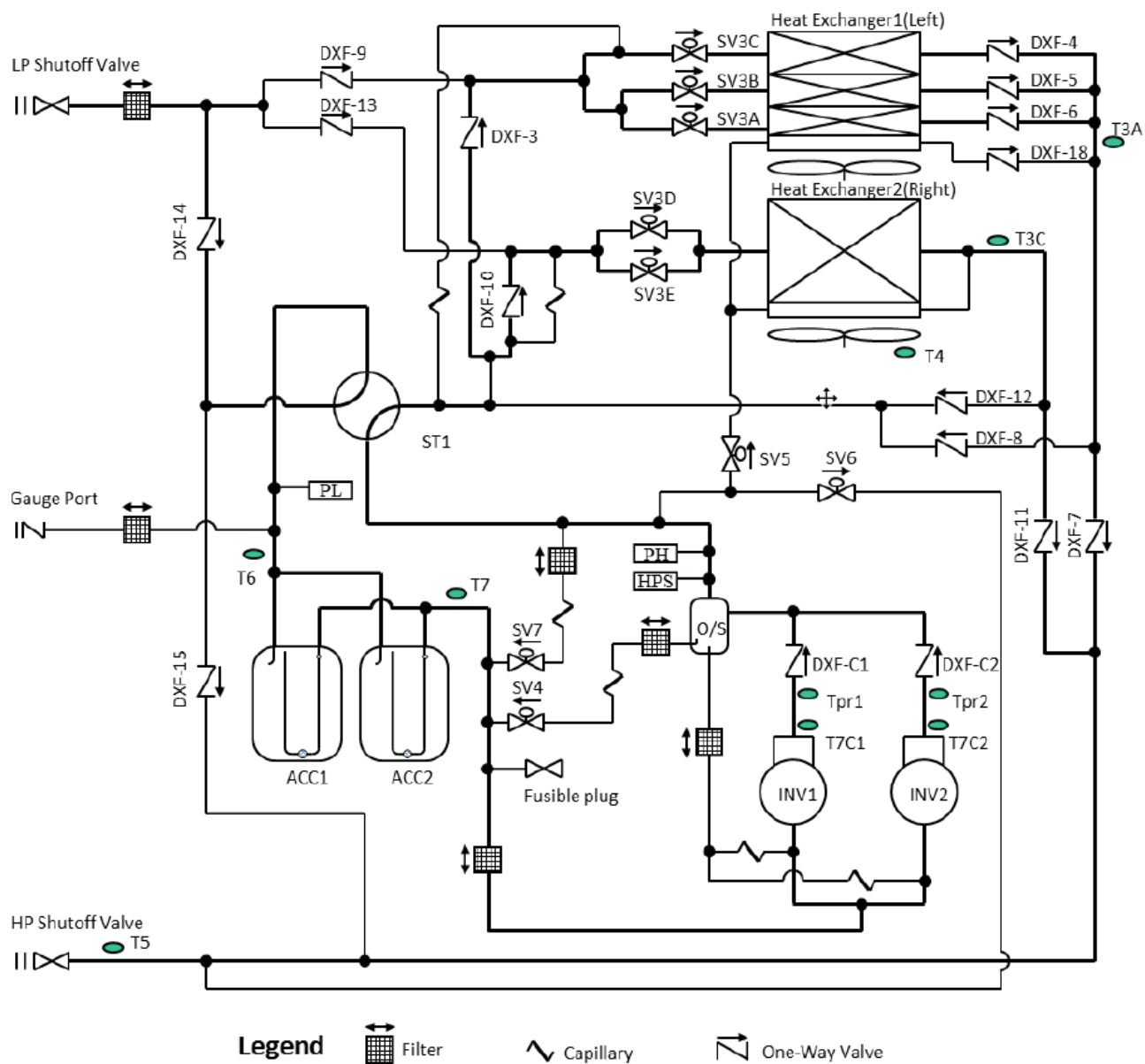
Fig. 8 —38VMA144RDL, 168, 196, 216, 240RDS Models
