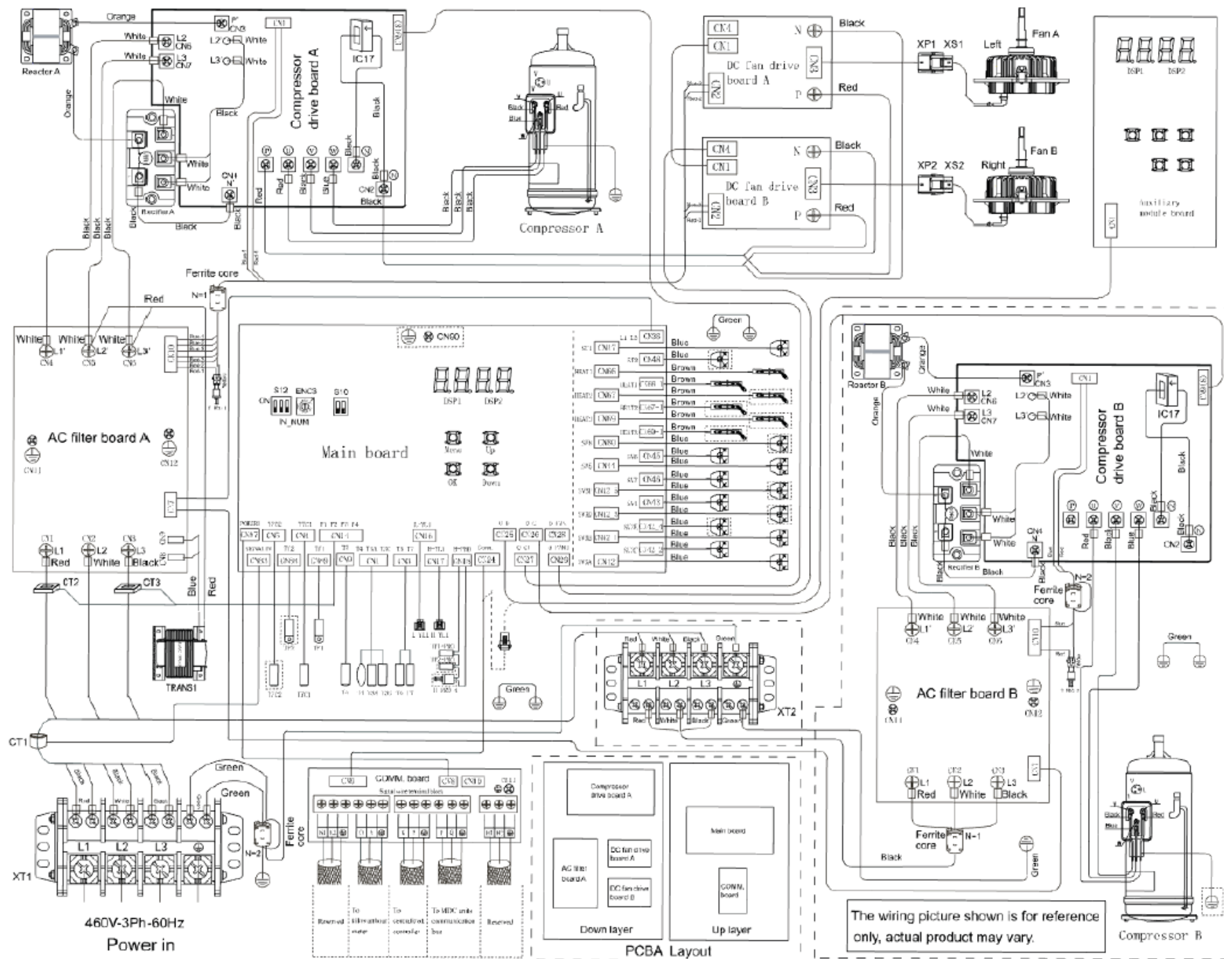
Fig. 13 —38VMA240RDL6-1, 38VMA264, 288, 312, 336RDS6-1
