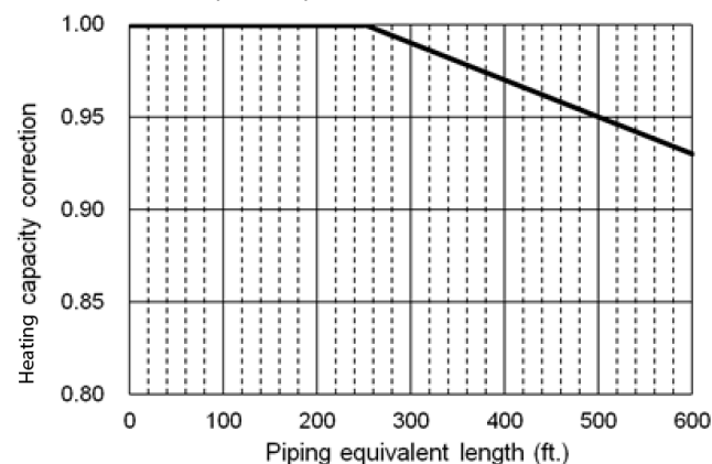
38VMA336RDS5-1(RDS6-1)
