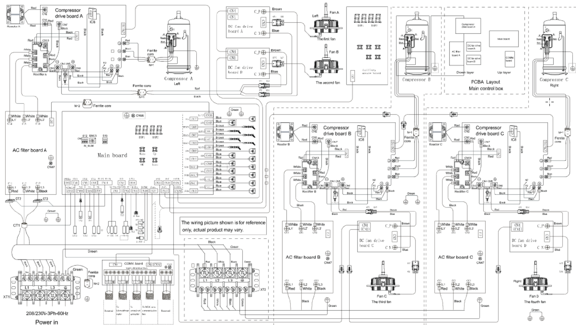
Fig. 11 —38VMA240RDL5-1, 38VMA264, 288, 312, 336RDS5-1
