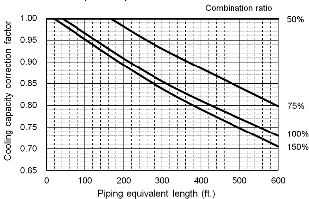
38VMA336RDS5-1(RDS6-1)
