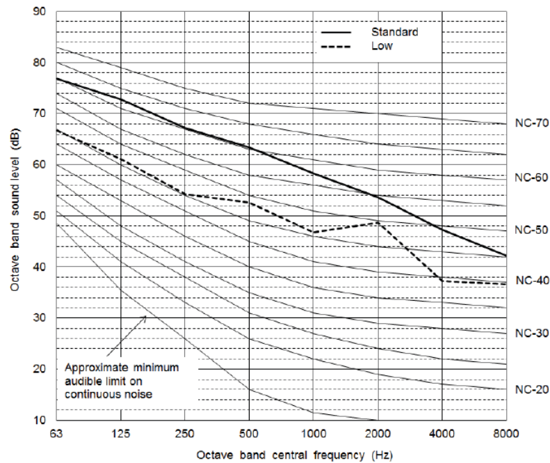
Fig. 40 —38VMA288RDS5-1
