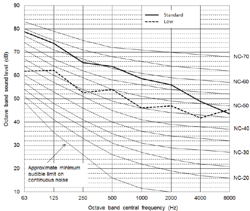
Fig. 41 —38VMA288RDS6-1
