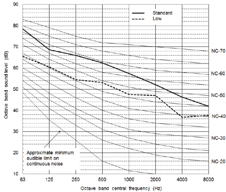
Fig. 36 —38VMA240RDL5-1
