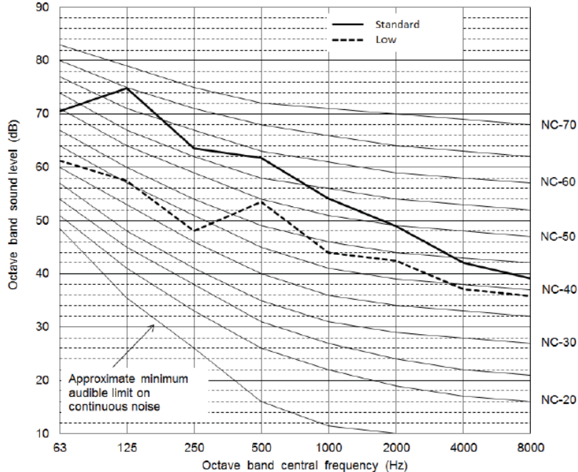
Fig. 27 —38VMA144RDL6-1
