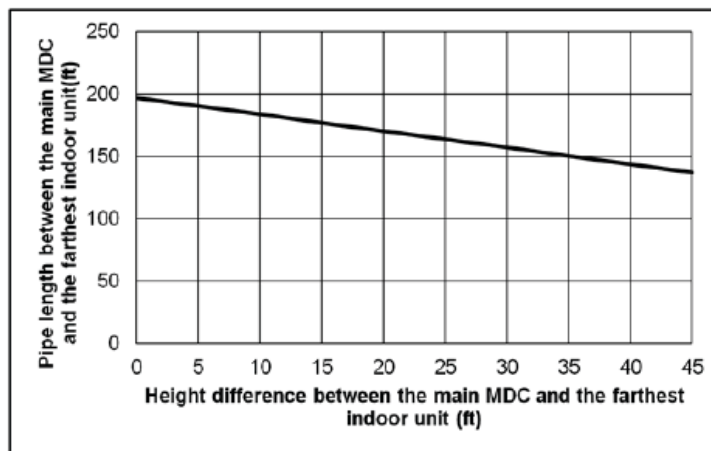
Fig. 48 —Piping Length and Height between Indoor Unit and MDC
