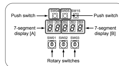
Interface PC board
