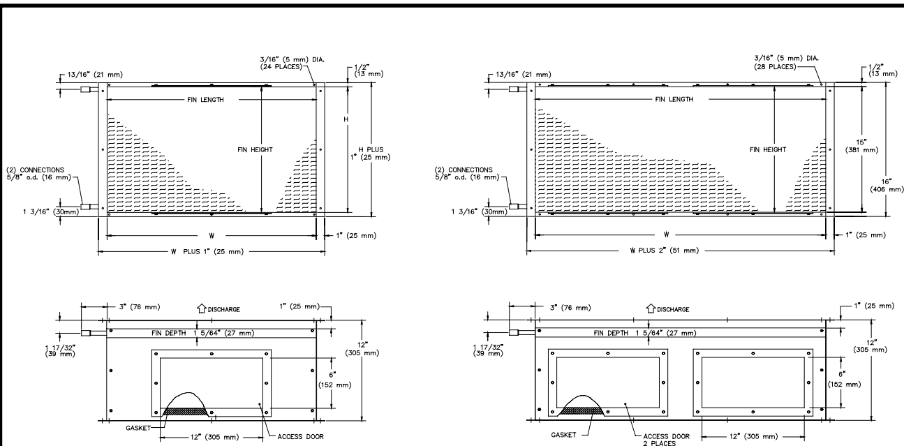
CONSTRUCTION TYPICAL OF UNIT SIZES 2 - 6
