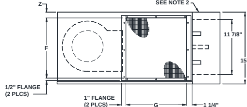
DISCHARGE VIEW
