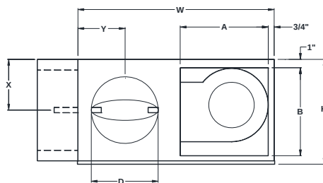
INLET VIEW
