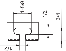
Detail of Z section
