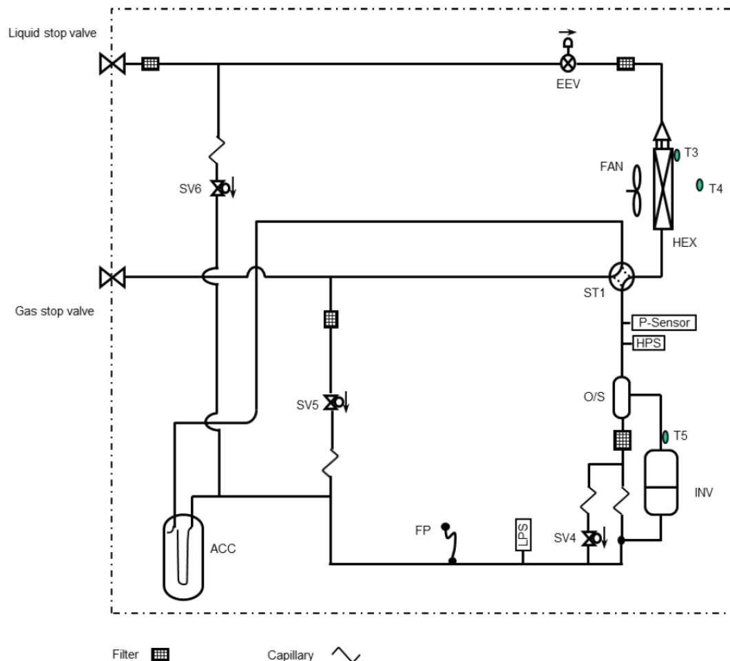
Fig. 8 —Refrigerant Circuit Diagram
