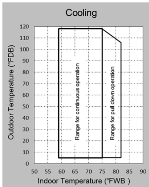
Fig. 11 —Operation Limits (Cooling)
