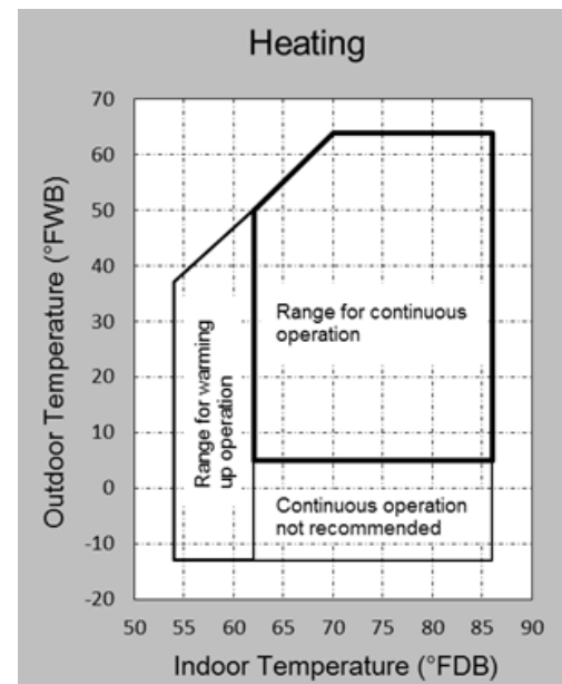
Fig. 12 —Operation Limits (Heating)
