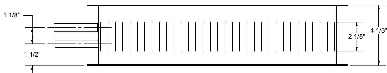
2 ROW HOT WATER COIL TOP VIEW
