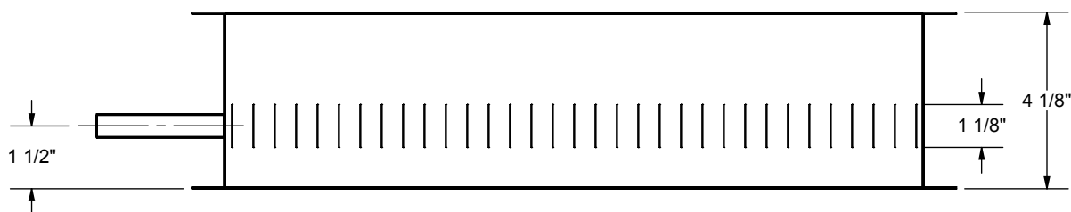
1 ROW HOT WATER COIL TOP VIEW
