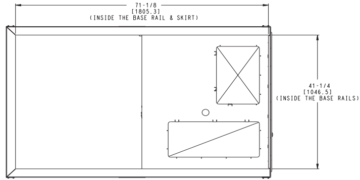
INSIDE BASERAIL DIMENSIONS
