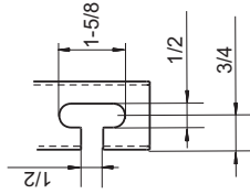
Detail of Z section
