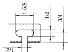
Detail of Z section
