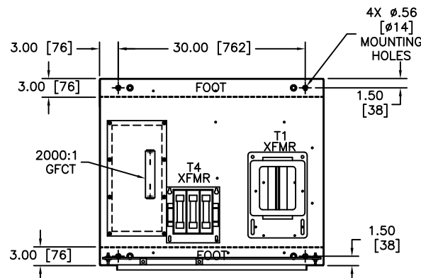
FRONT OF ENCLOSURE PLAN VIEW
