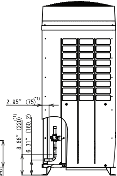
(*1)Cutting position of L-shape pipe
