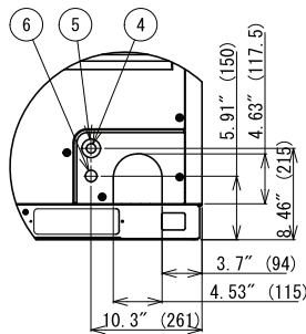
Holes for piping/wiring
