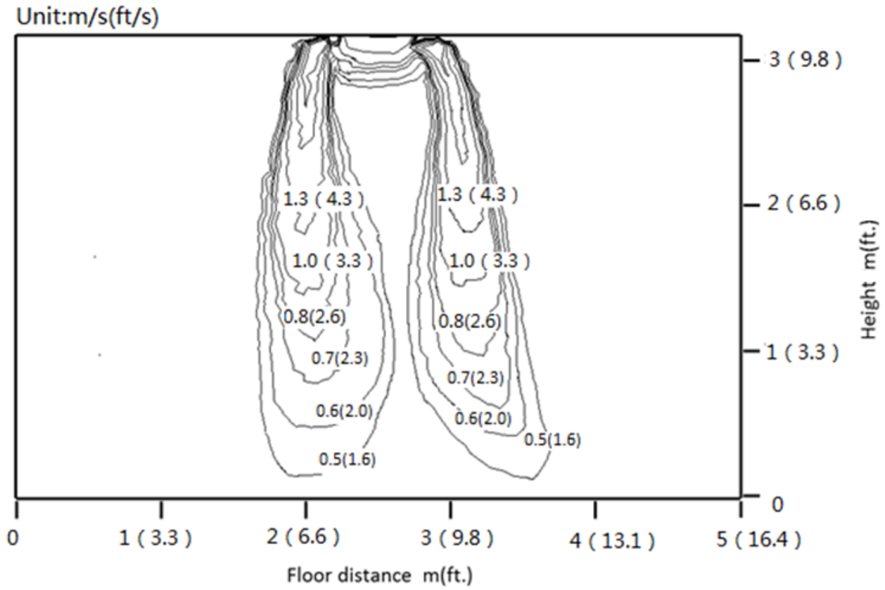
Fig. 13 —Cooling Mode with 60° Swing
