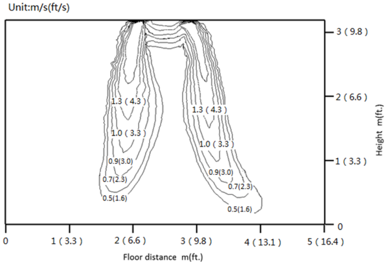
Fig. 14 —Heating Mode with 60° Swing
