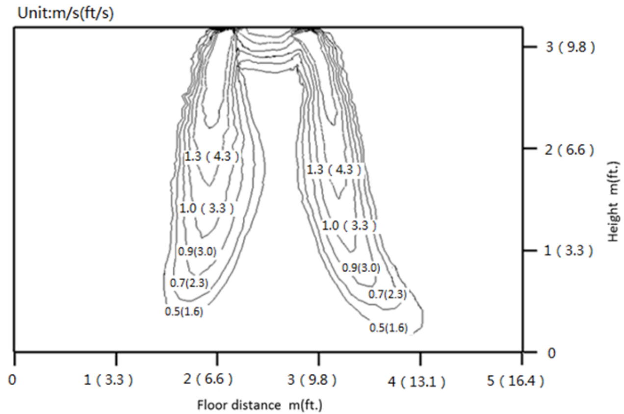
Fig. 10 —Heating Mode with 60° Swing
