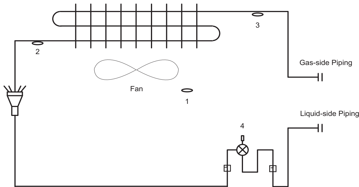
Fig. 1 —Piping
