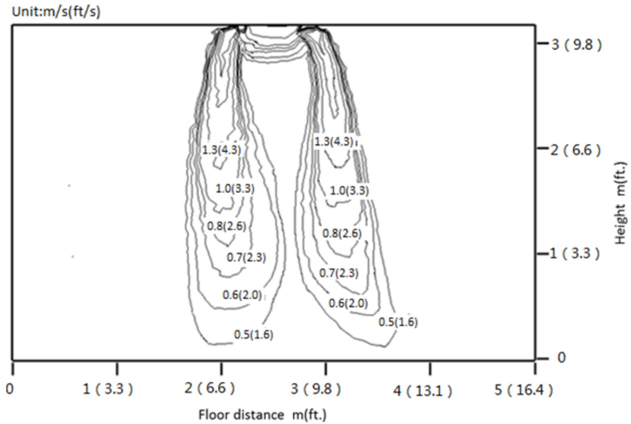
Fig. 9 —Cooling Mode with 60° Swing
