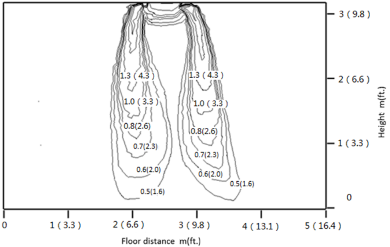
Fig. 7 —Cooling Mode with 60° Swing
