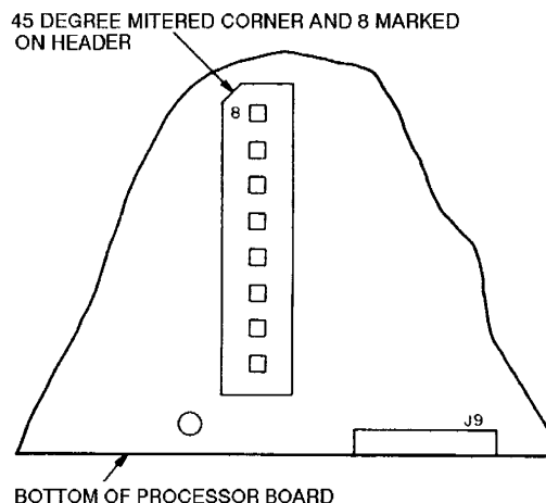
Fig. 27 — Configuration Header
