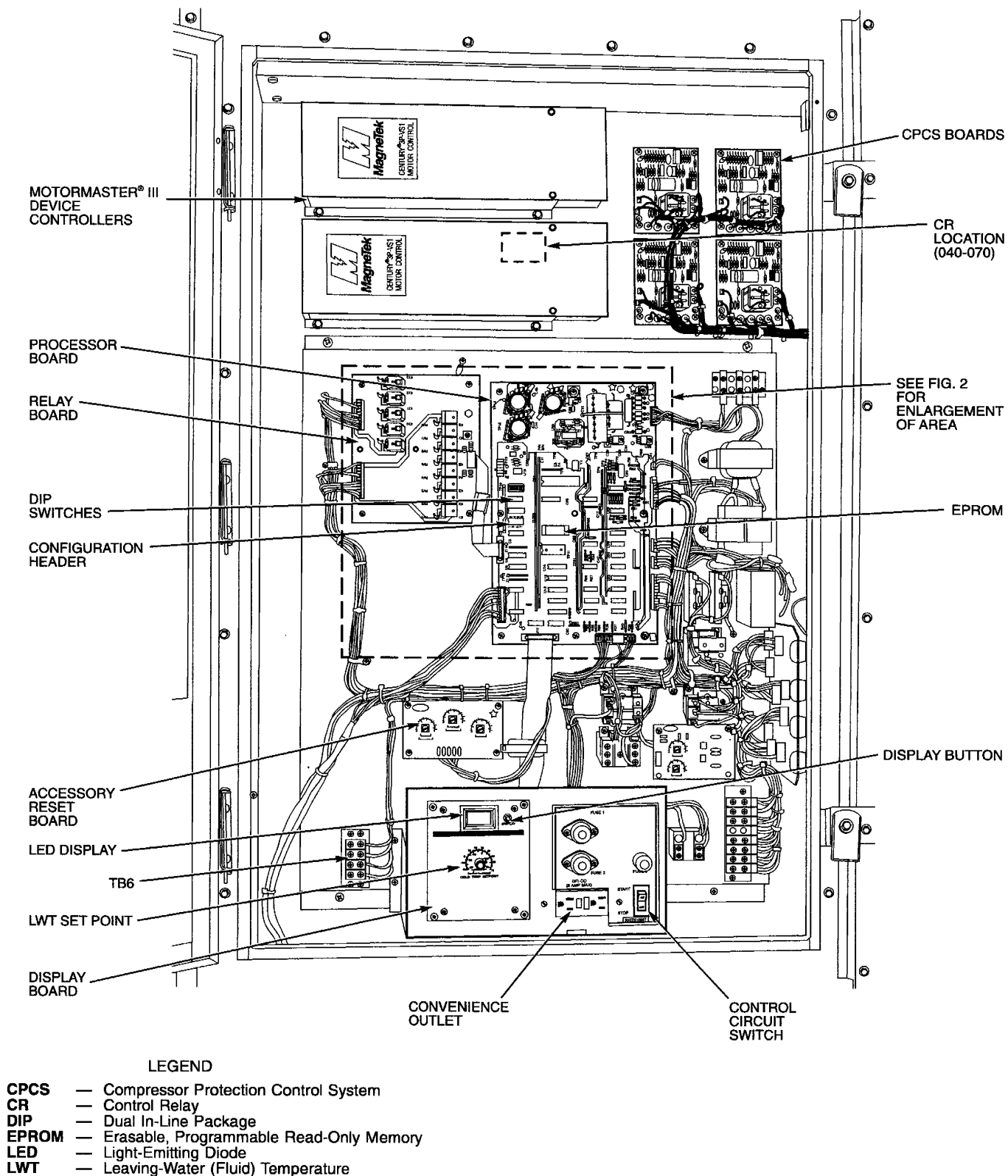
Fig. 1 — Typical Control Box (080-110 and Associated Modular Units Shown)
