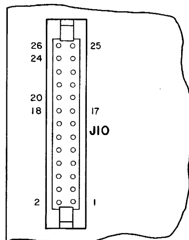
Fig. 26 — Display Board Connector
