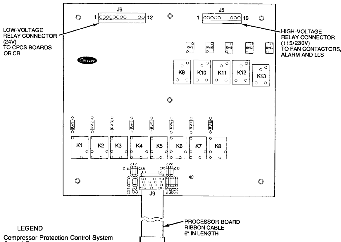
Fig. 6 — Relay Board
