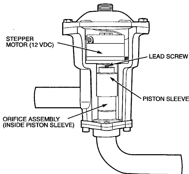
Fig. 15 — Electronic Expansion Valve (EXV)
