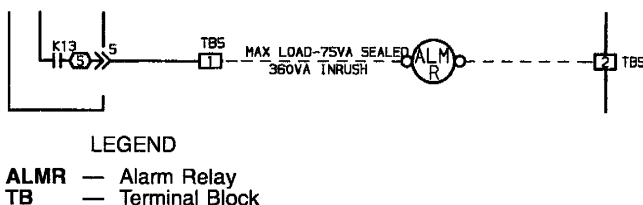
Fig. 21 — Remote Alarm Wiring
