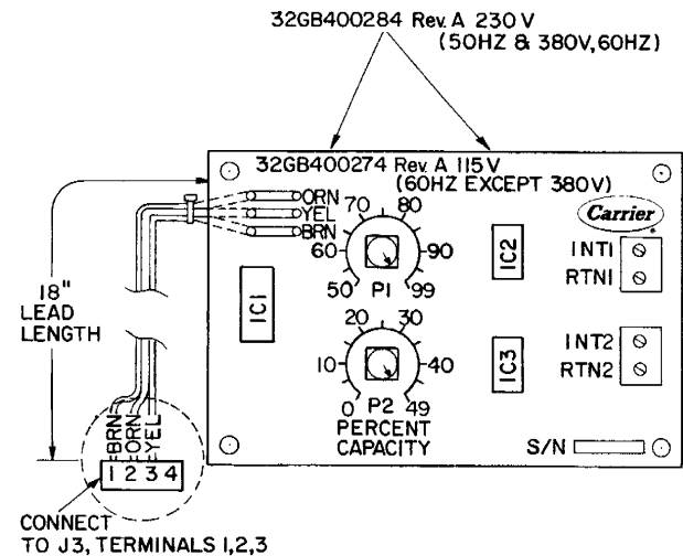
Fig. 12 — Accessory Reset Board
