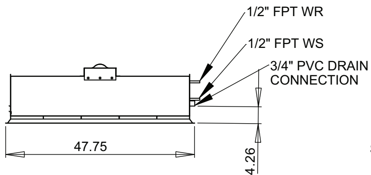
REAR VIEW
