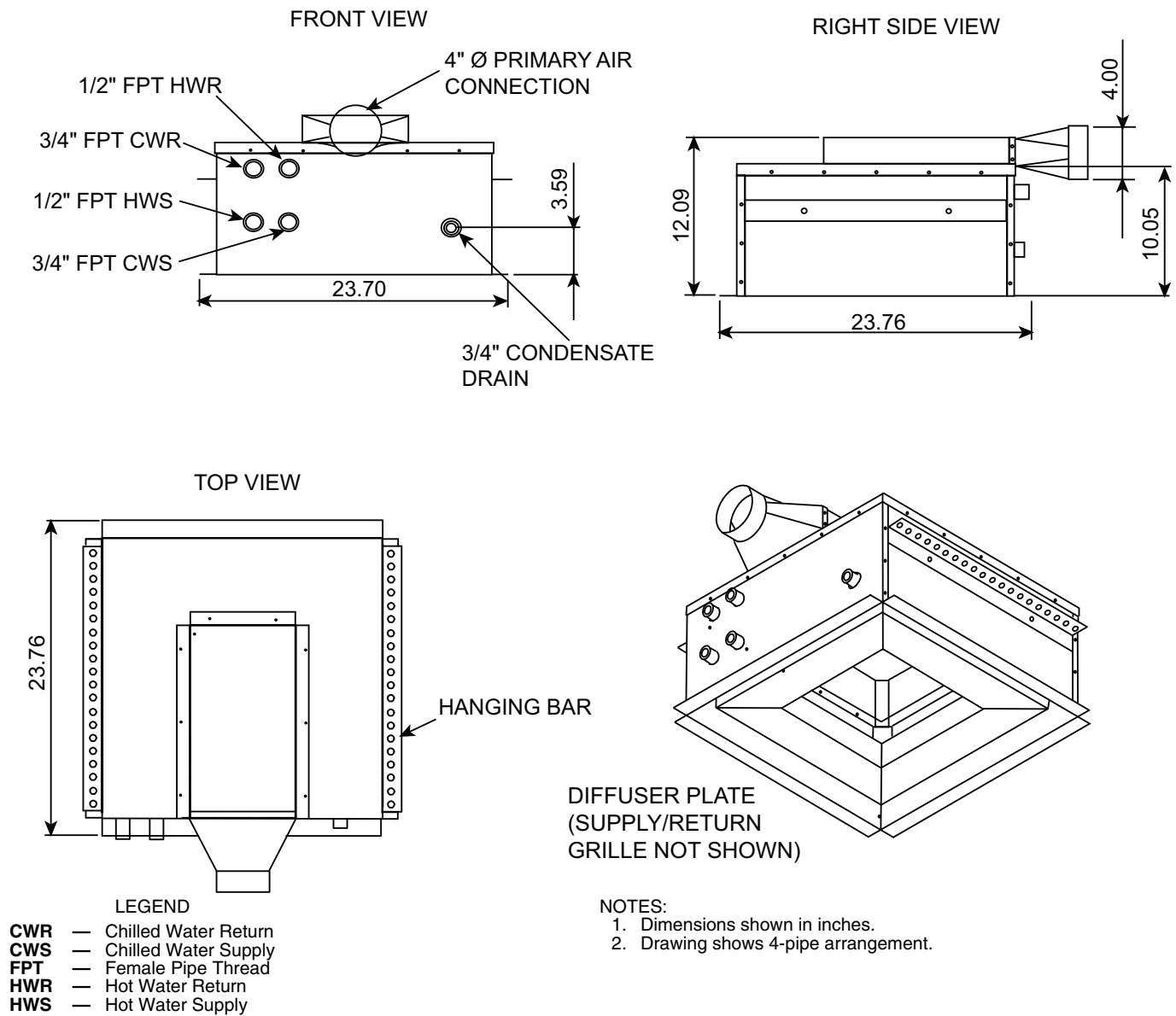
Fig. 3 — 36IBAC 2 x 2, All-Way Blow, 4-Pipe Unit Dimensions
