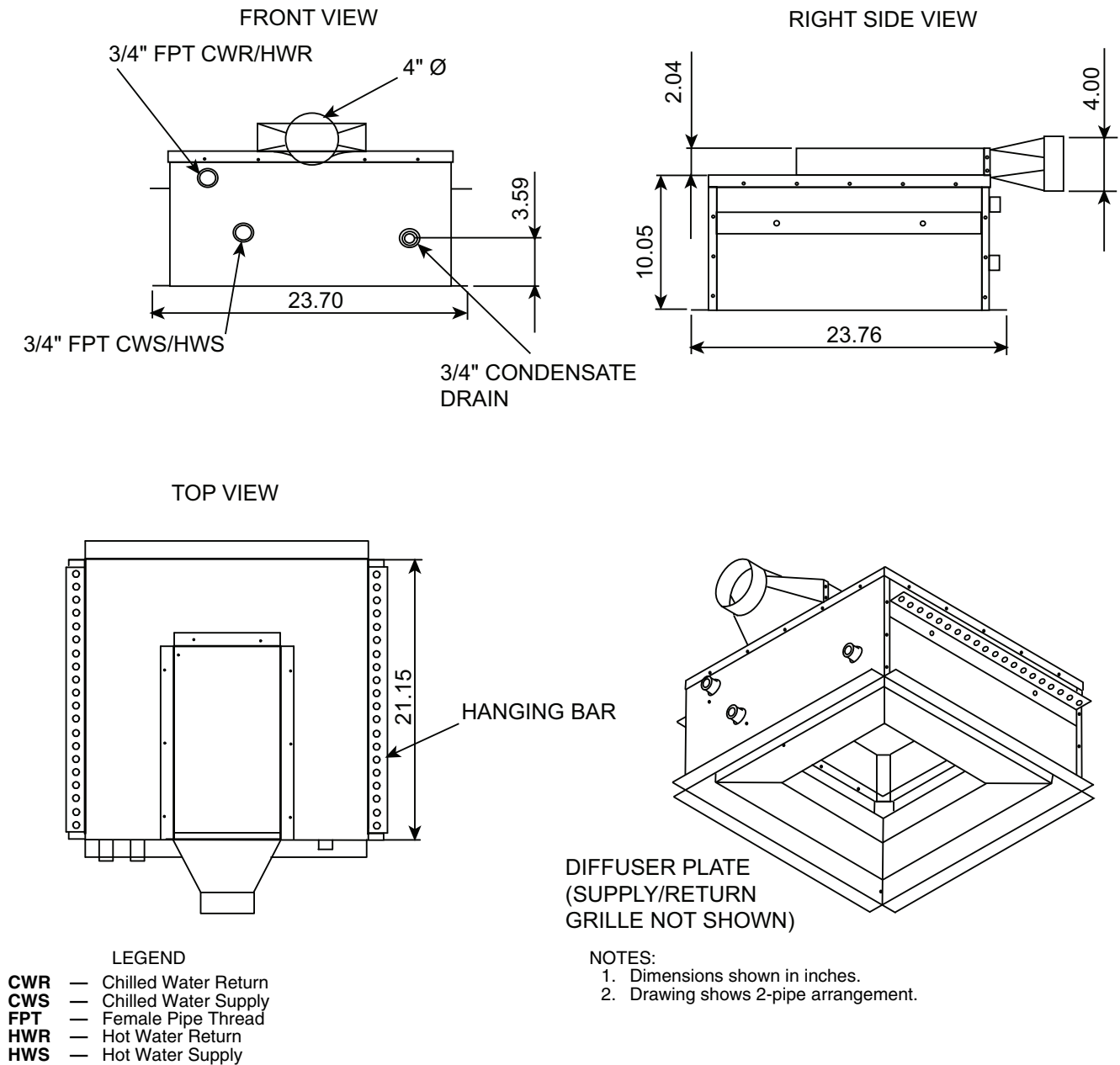
Fig. 2 — 36IBAC 2 x 2, All-Way Blow, 2-Pipe Unit Dimensions
