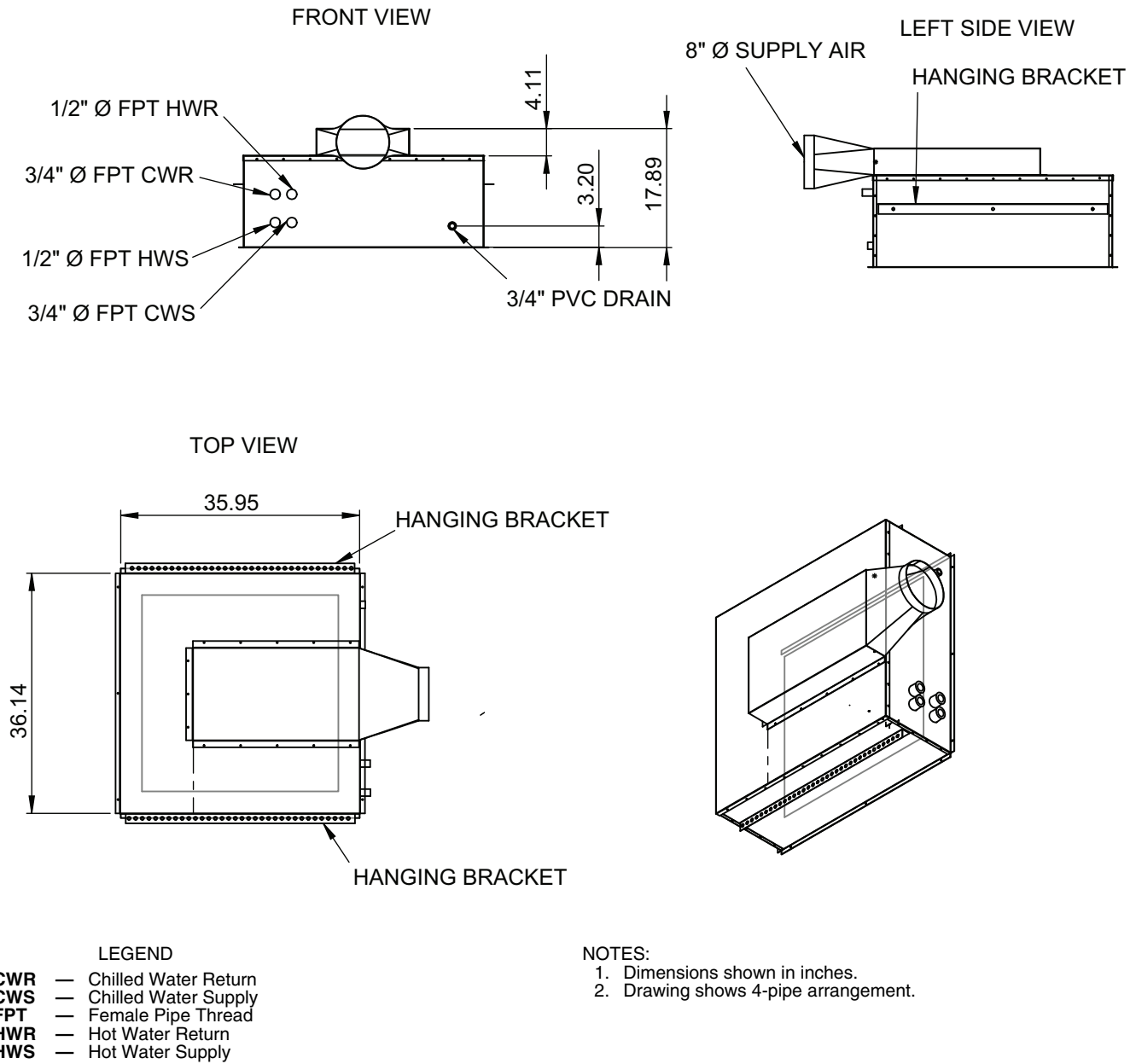
Fig. 5 — 36IBAC 4 x 4, All-Way Blow, 4-Pipe Unit Dimensions
