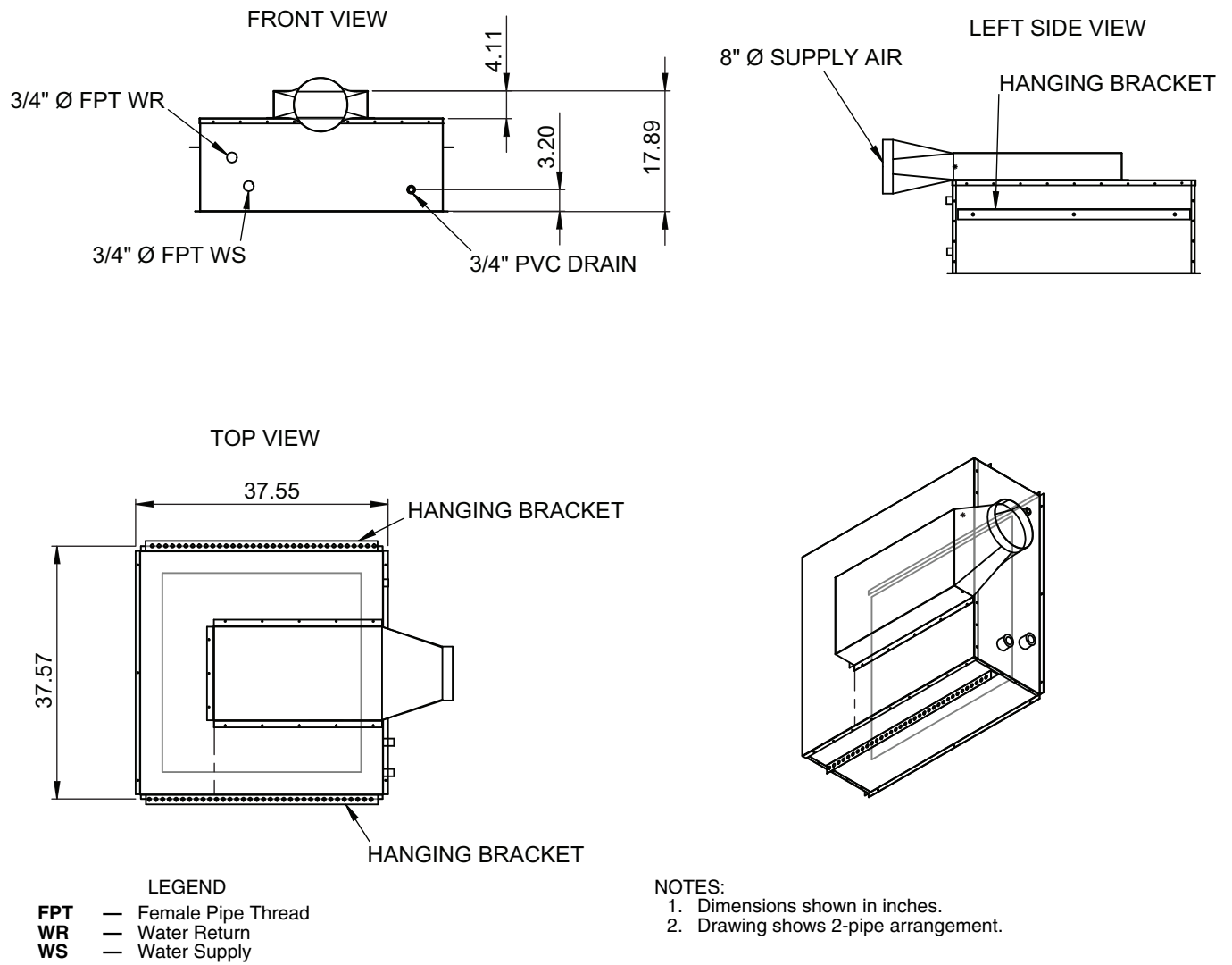
Fig. 4 — 36IBAC 4 x 4, All-Way Blow, 2-Pipe Unit Dimensions
