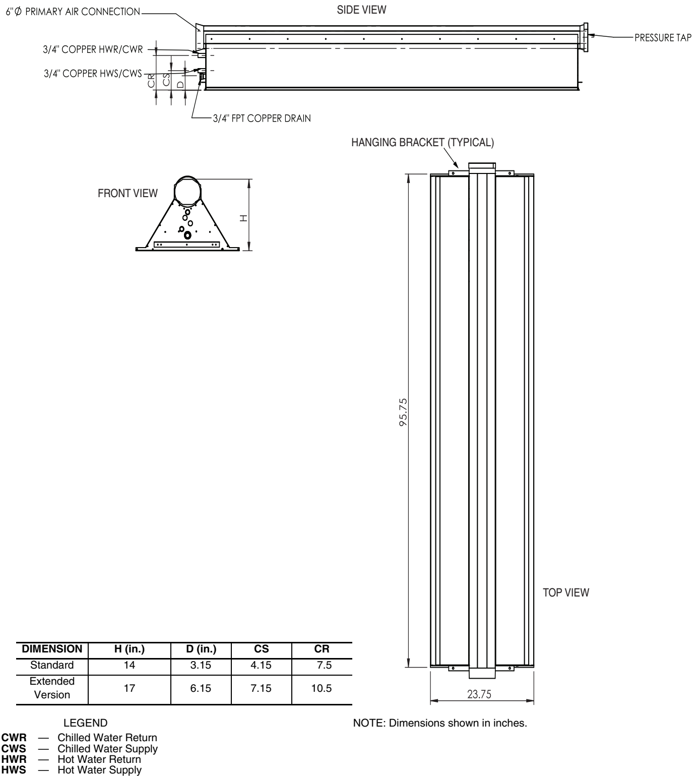
Fig. 19 — 36IBAL 8 x 2, 2-Way Blow, 2-Pipe Unit Dimensions
