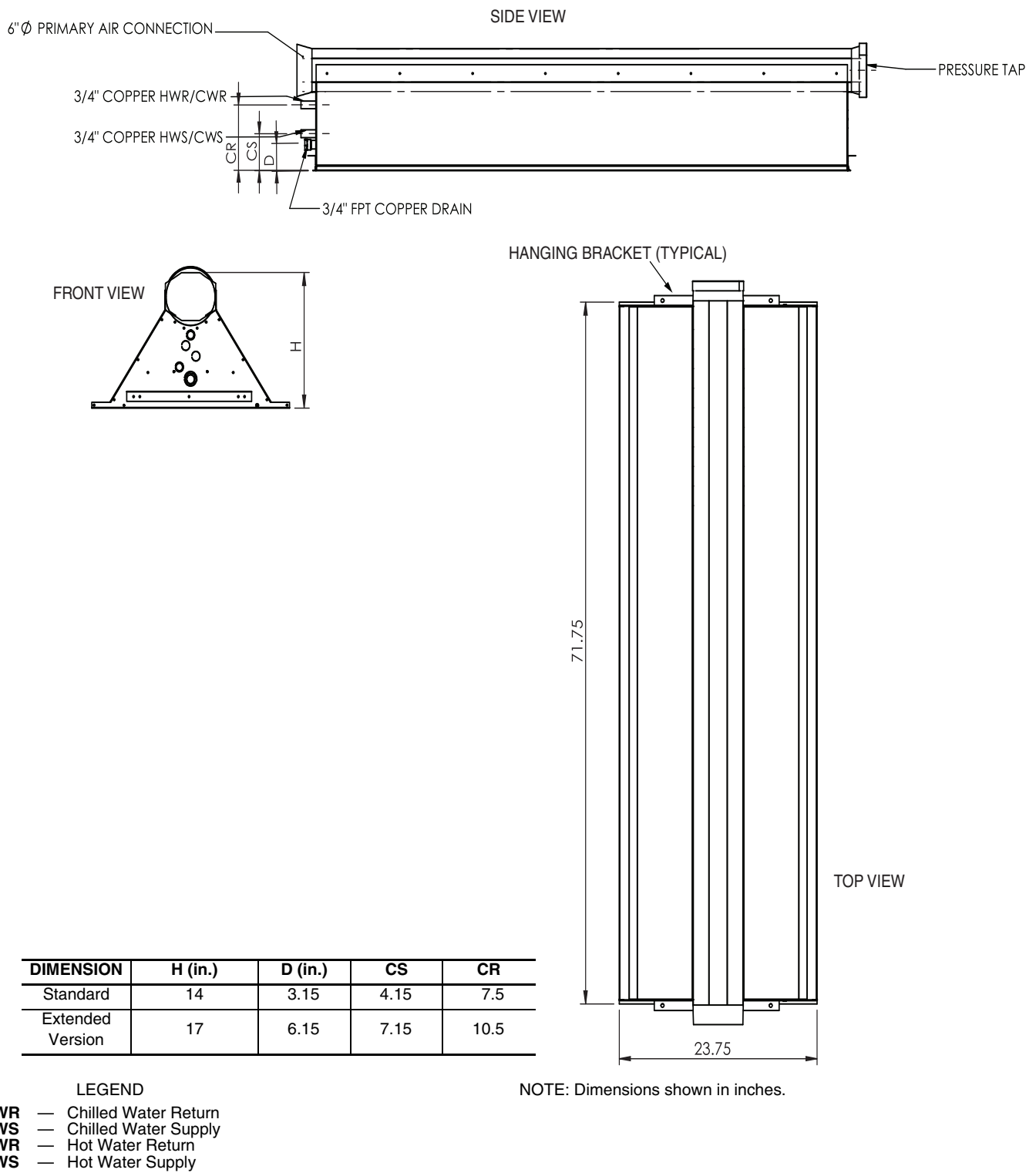
Fig. 18 — 36IBAL 6 x 2, 2-Way Blow, 2-Pipe Unit Dimensions
