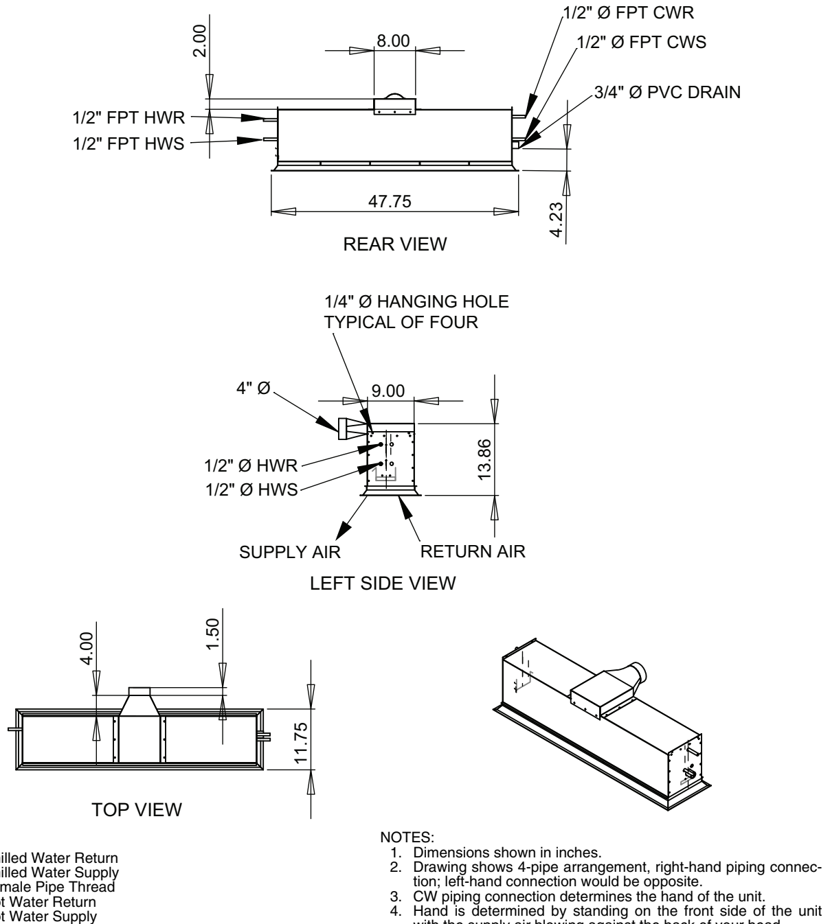
Fig. 11 — 36IBAN 1 x 4, 1-Way Blow, 4-Pipe RH Unit Dimensions
