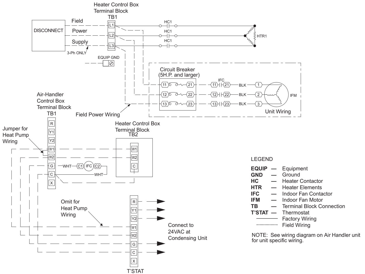
Fig. 7 — Electric Heat and Control Wiring (without UCB Board)
