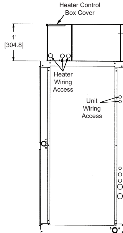
Right Side
