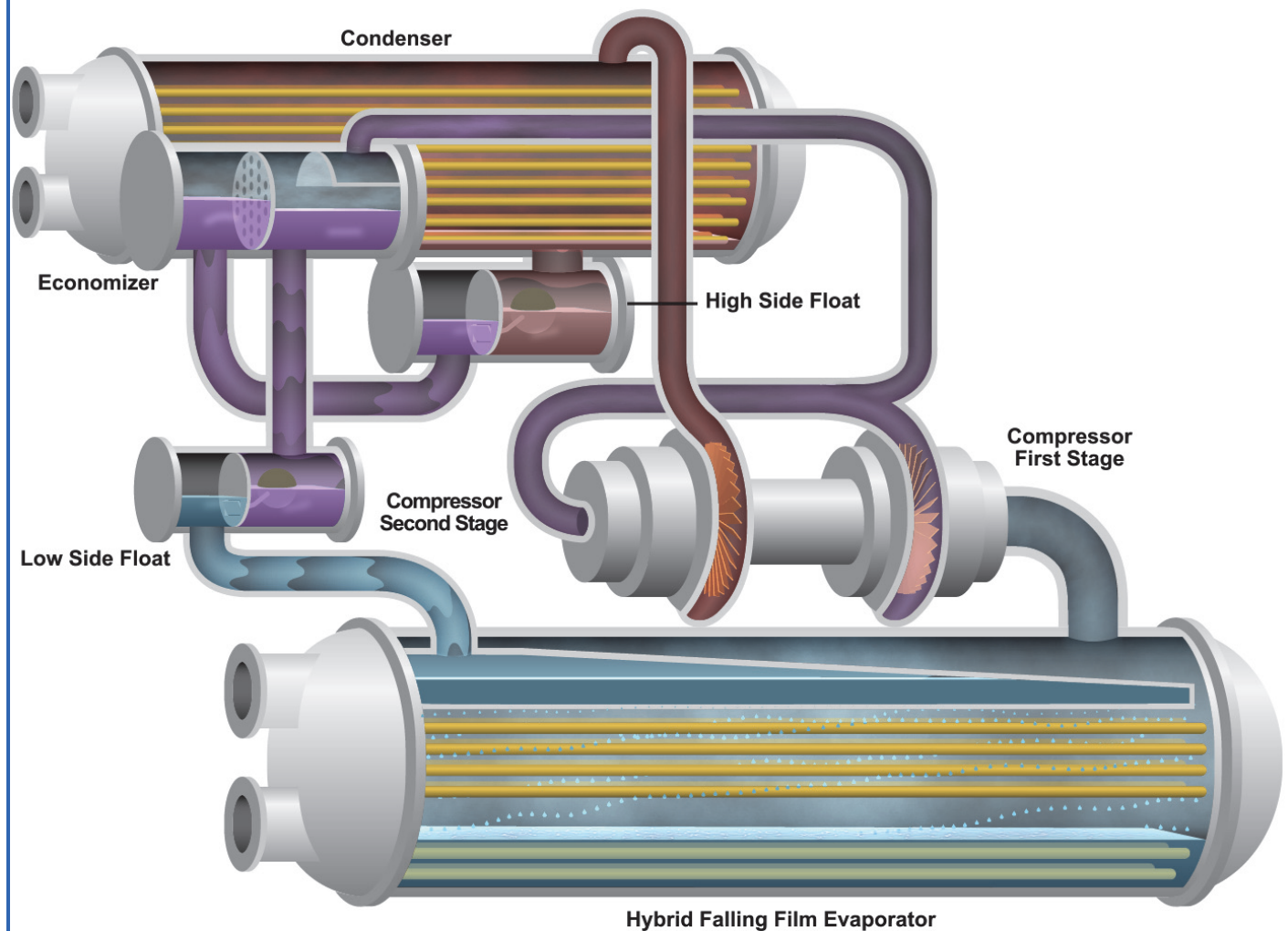
Refrigeration Cycle 19DV Two-Stage Compressor Frame
