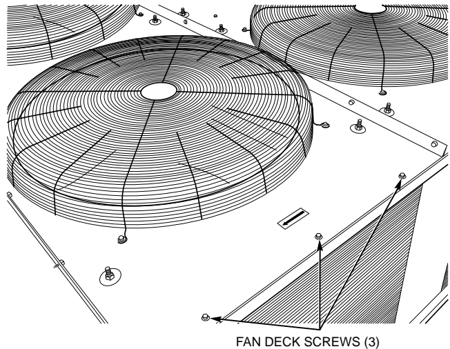
Fig. 2 — Fan Deck Screw Locations (Each Coil Section)
