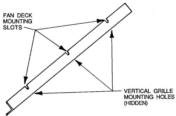
Fig. 3 — Grille Angle (Grille Mounting Bracket)
