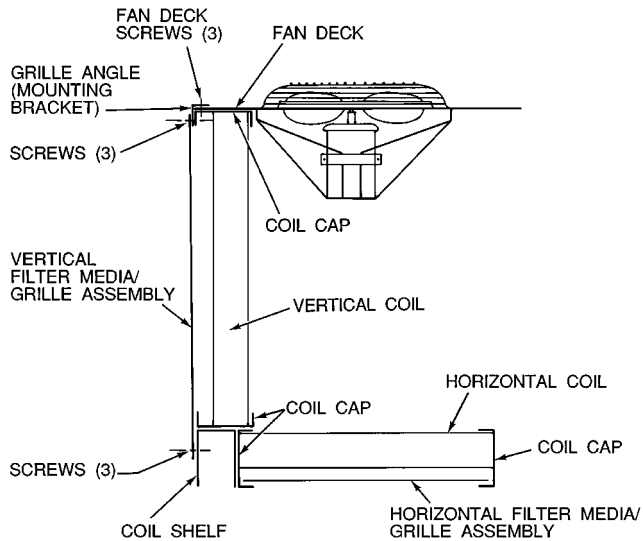
Fig. 4 — Filter Media/Grille Mounting Locations
