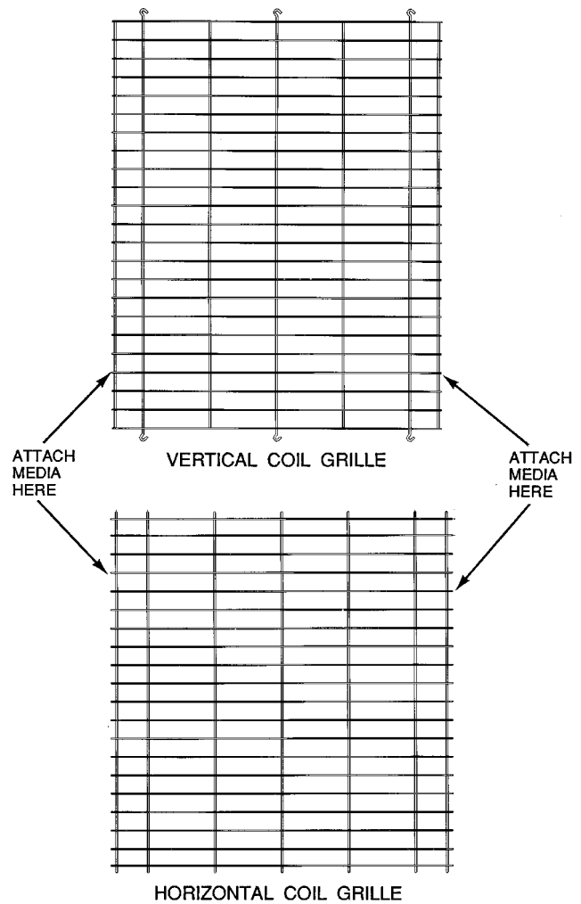
Fig. 1 — Filter Media Support Grilles
