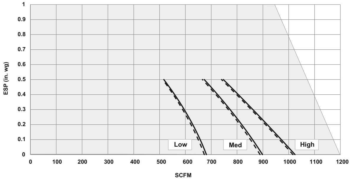
AIR DELIVERY (cont) 42S SERIES — UNIT SIZE 10
