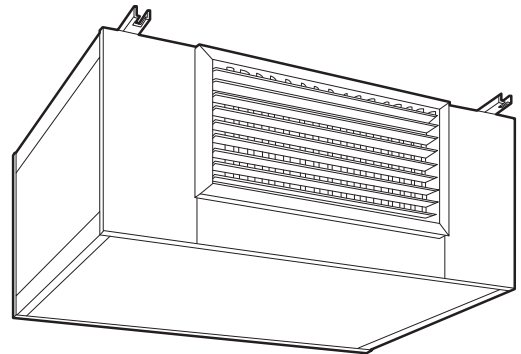
42DF Exposed-ceiling painted cabinet model with integral double-deflection discharge grille and a bar-type return-air grille for non-ducted applications (600-2000 cfm)
