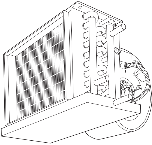
42DA Furred-in model for installation in the ceiling for high static applications. (600-2000 cfm)
