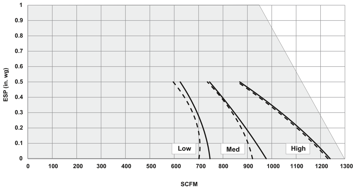
42S SERIES — UNIT SIZE 12
