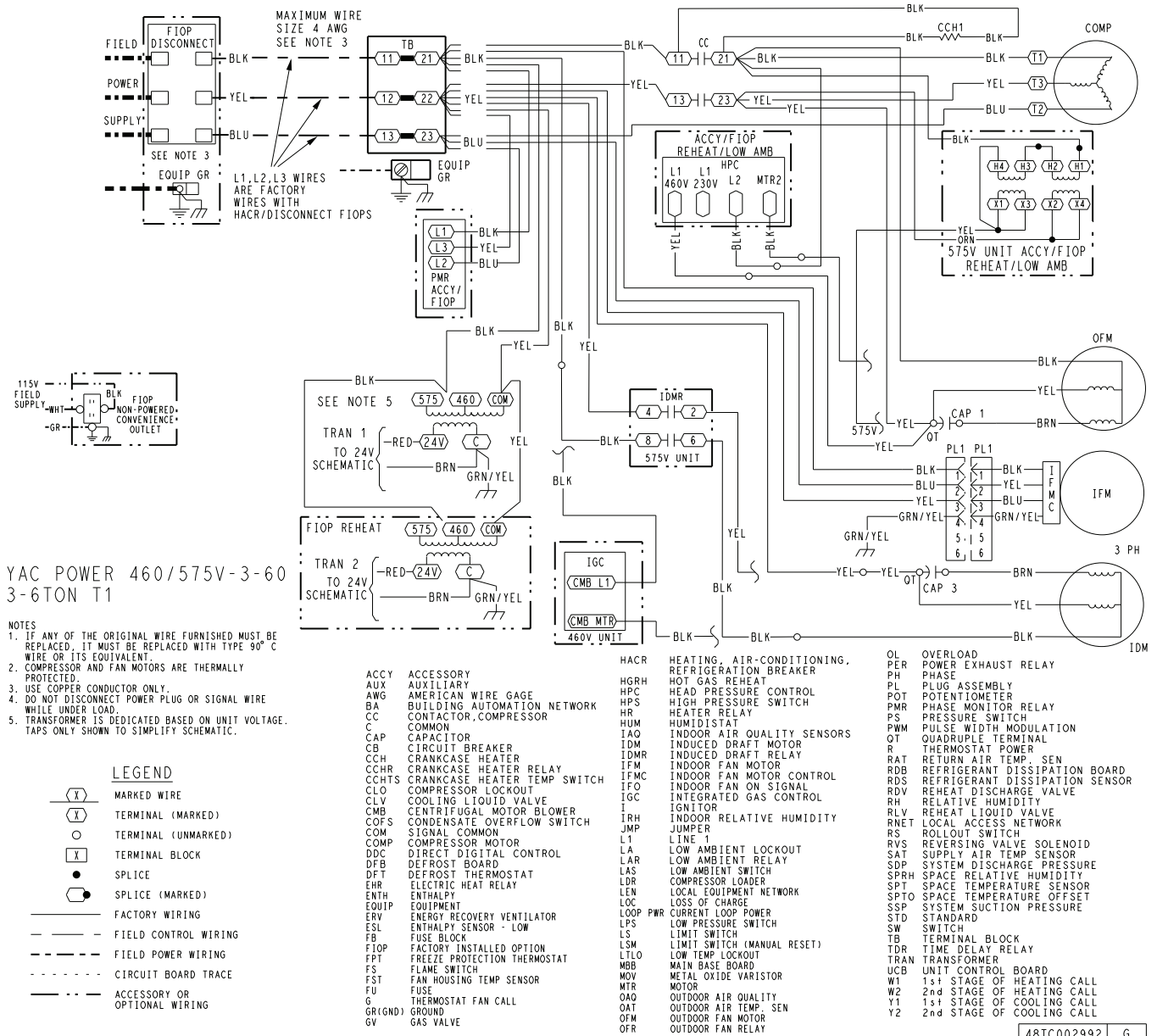
Typical 48FC 04-07 Power Wiring Diagram, 460-575/3/60 Unit Shown
