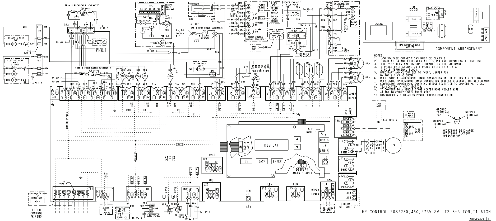
Fig. F — 50GCQ 04-06, All Voltages — Optional Factory-Installed SystemVu™ Controller
