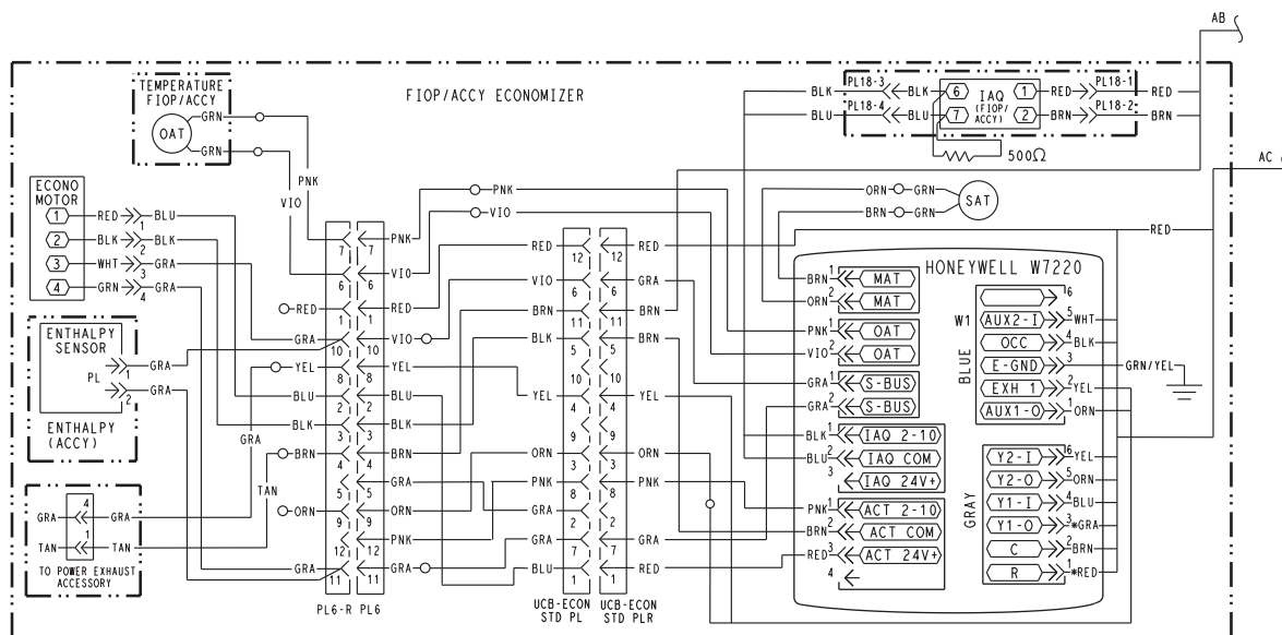
Fig. 67 — Typical EconoMi$er X (W7220 Controller) Wiring
