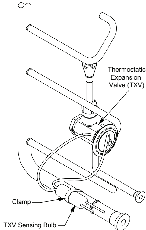
Fig. 20 — TXV Valve and Sensing Bulb Location
