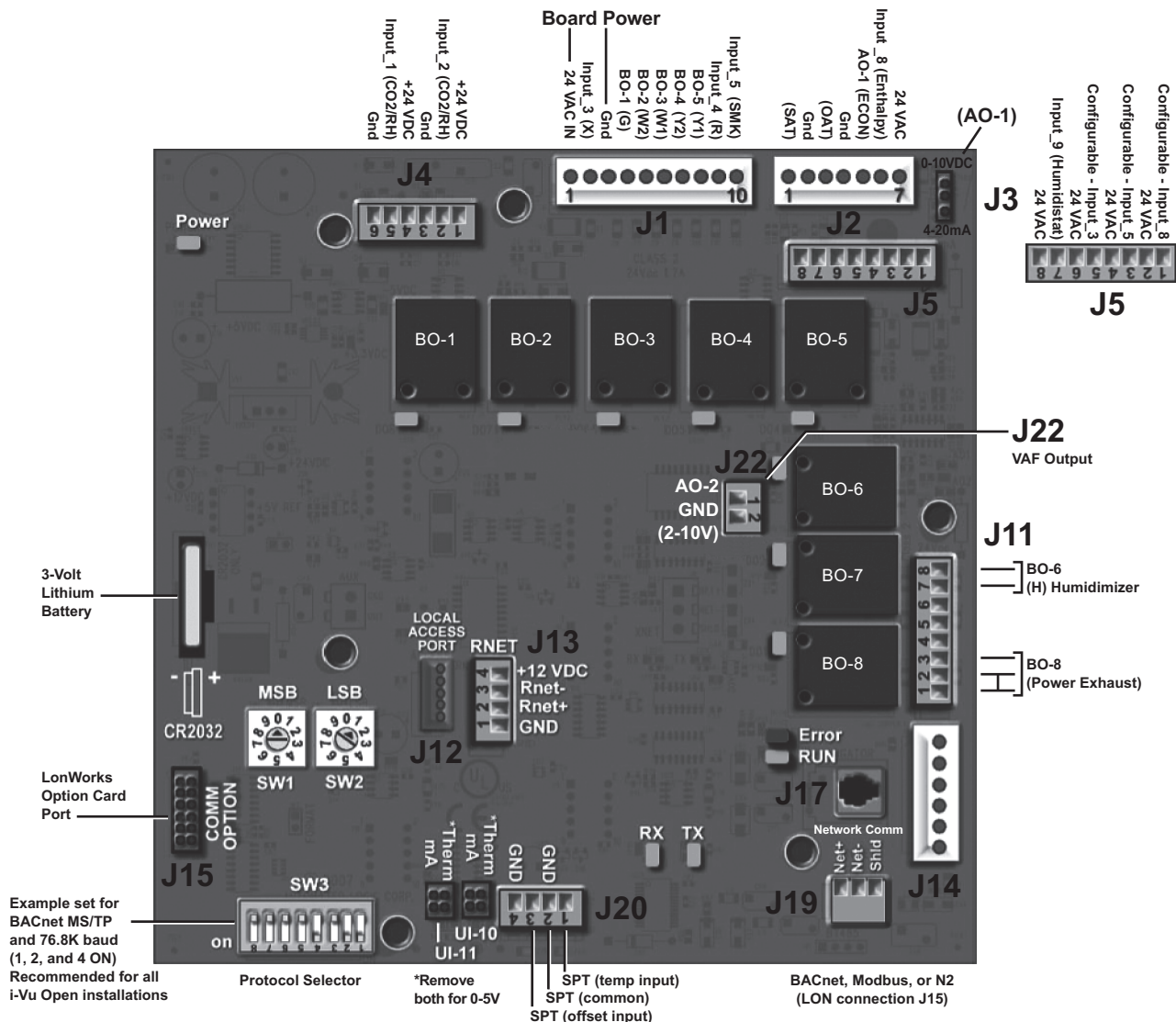
Fig. 51 — RTU Open Control Module
