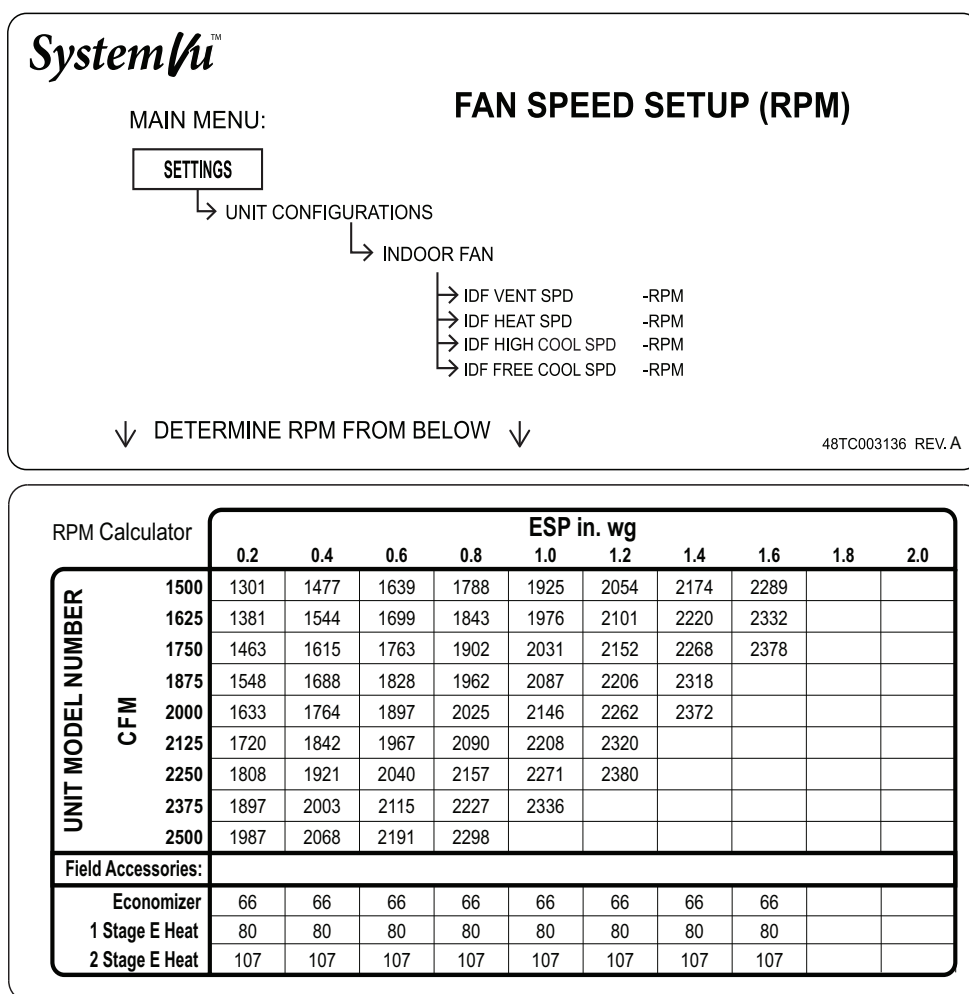
Fig. 9 — Example of Fan Speed Set Up Labels for SystemVu™ Controls
