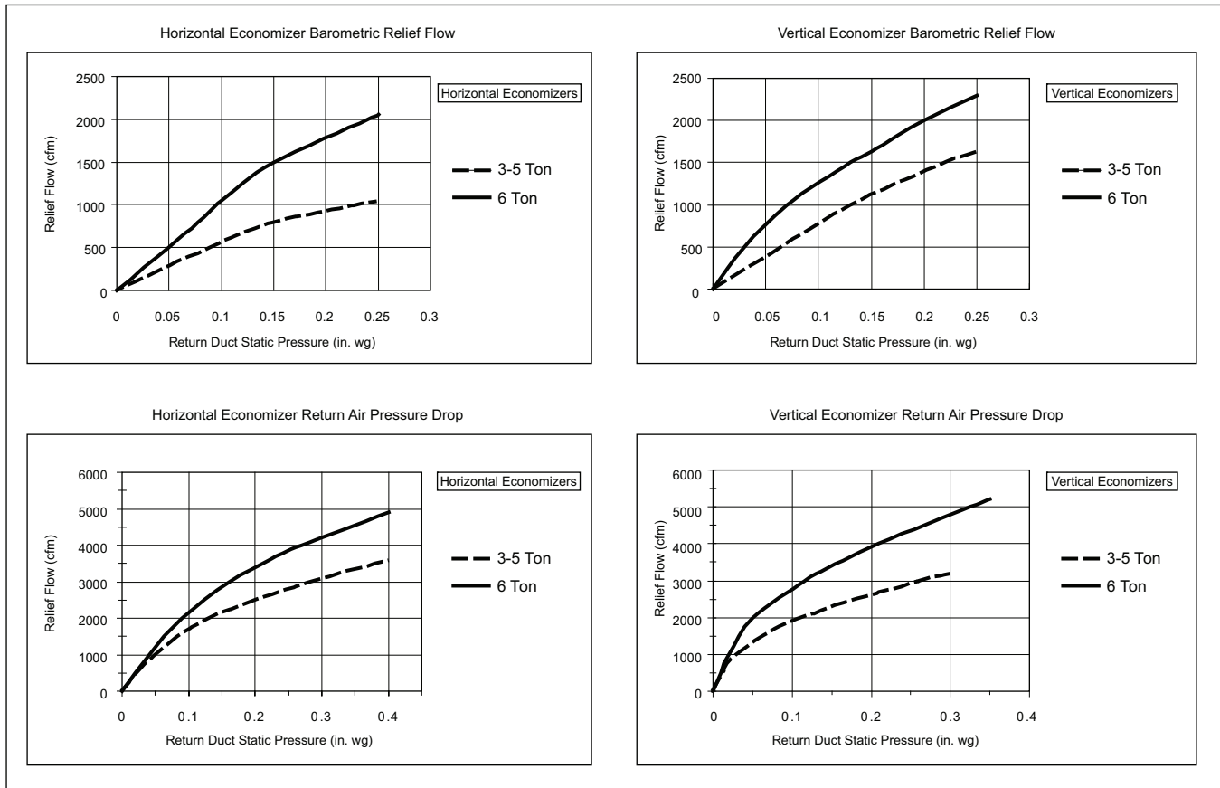
Fig. 61 — Outdoor-Air Damper Leakage
