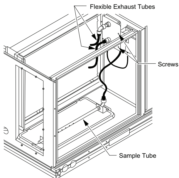
Fig. 44 — Return Air Smoke Detector Shipping Position
