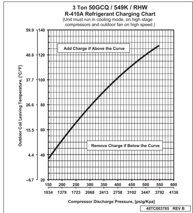
Fig. 22 — Cooling Charging Chart — 3 Ton
