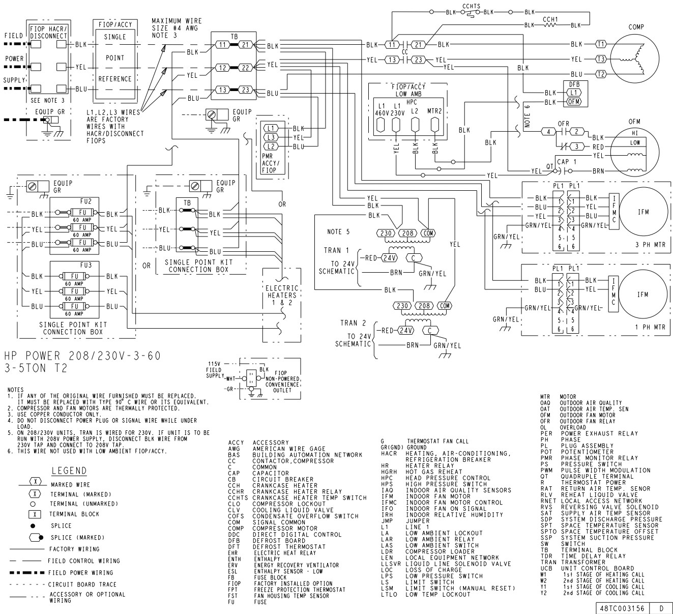
Fig. H — 50GCQ 04-06 Power Wiring Diagram — 208/230-3-60 Units
