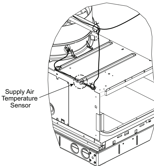
Fig. 59 — Supply Air Sensor Location
