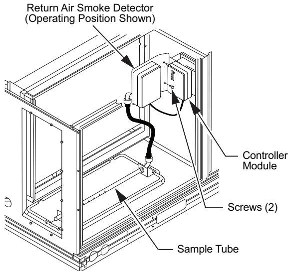
Fig. 45 — Return Air Smoke Detector Operating Position
