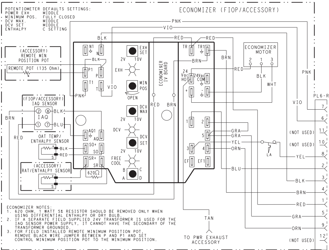
Fig. 56 — EconoMi$er IV Functional View
