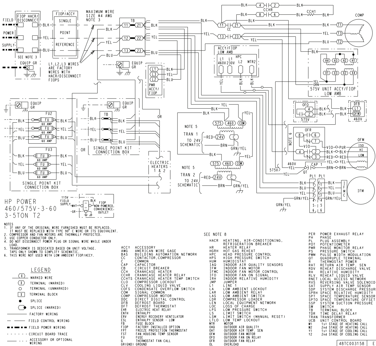
Fig. I — 50GCQ 04-06 Power Wiring Diagram — 460/575-3-60 Units
