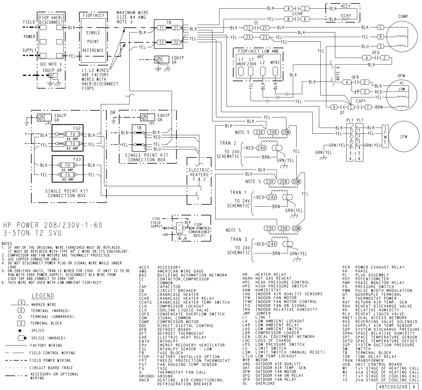
Fig. J — 50GCQ 04-06 SystemVu™ Power Wiring Diagram — 208/230-1-60 Units
