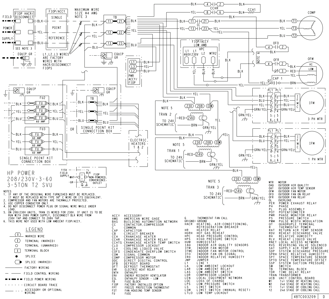
Fig. K — 50GCQ 04-06 SystemVu™ Power Wiring Diagram — 208/230-3-60 Units
