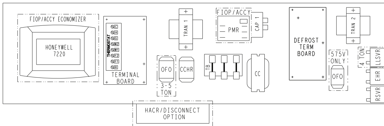
Fig. 31 — Defrost Control Board Location — 50GCQ*04-06 Electro-Mechanical Units
