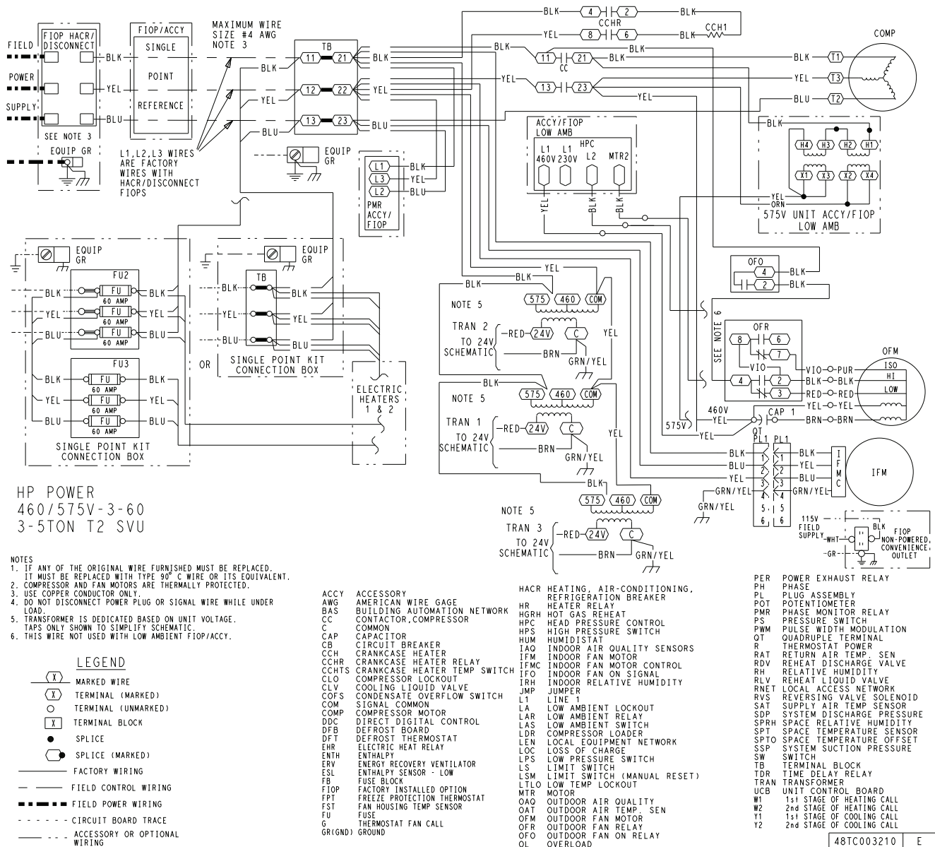
Fig. L — 50GCQ 04-06 SystemVu™ Power Wiring Diagram — 460/575-3-60 Units
