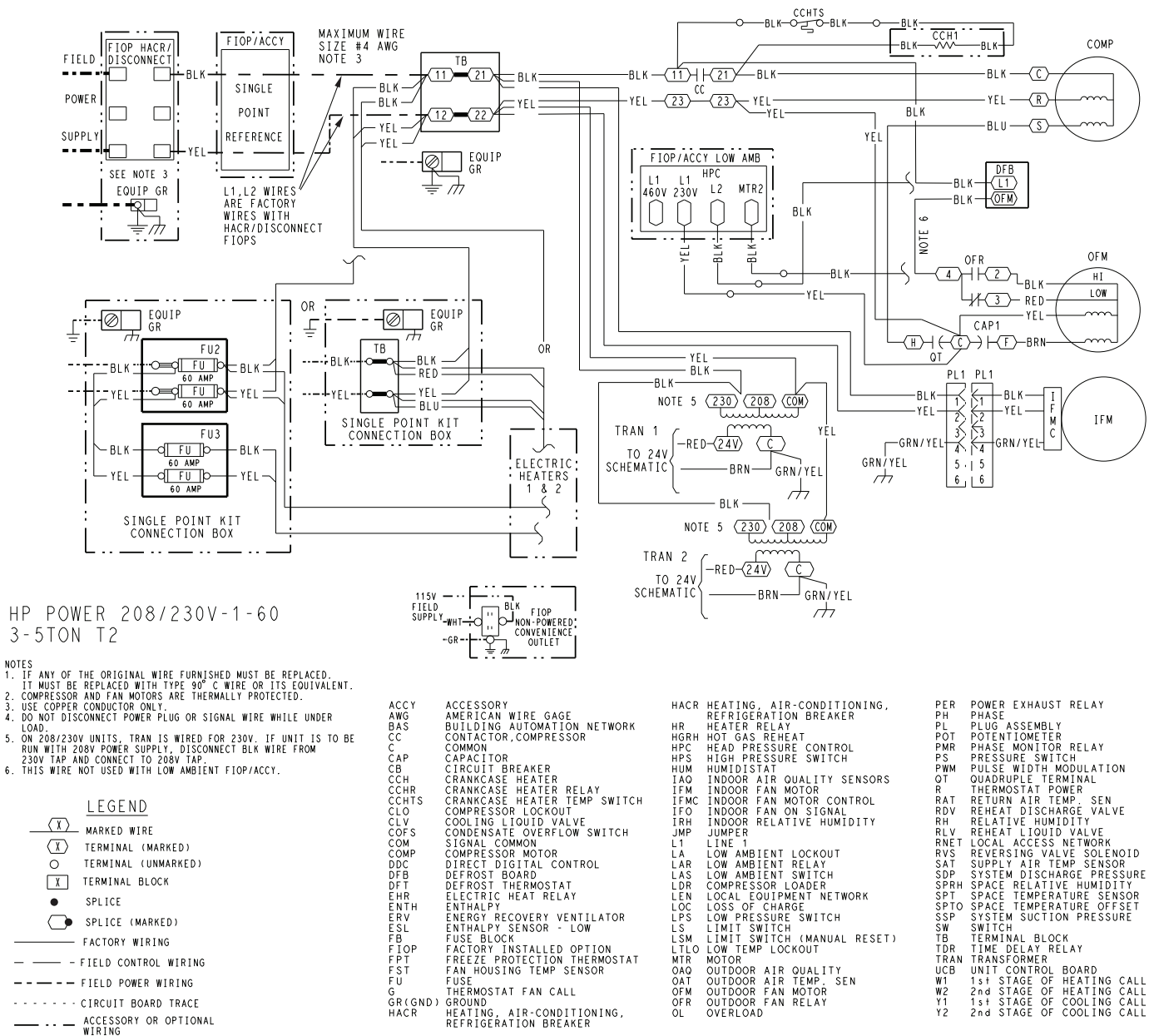
Fig. G — 50GCQ 04-06 Power Wiring Diagram — 208/230-1-60 Units
