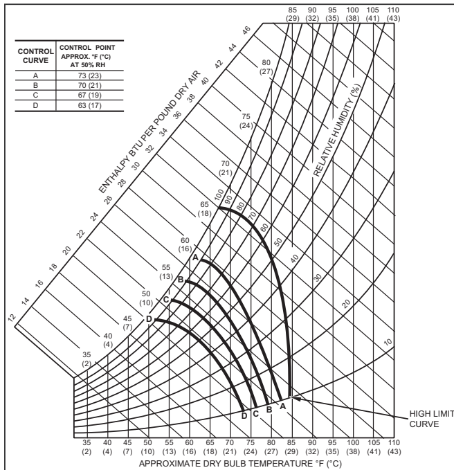
Fig. 64 — Enthalpy Changeover Set Points
