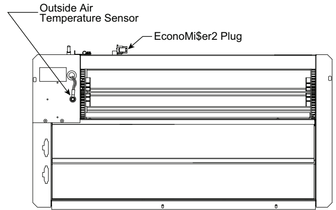
Fig. 54 — EconoMiSer 2 Component Locations
