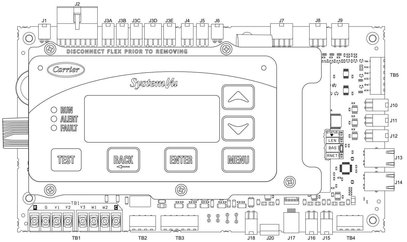
Fig. 50 — SystemVu Control
