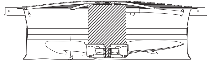
Fig. 25 — Condenser-Fan Adjustment
