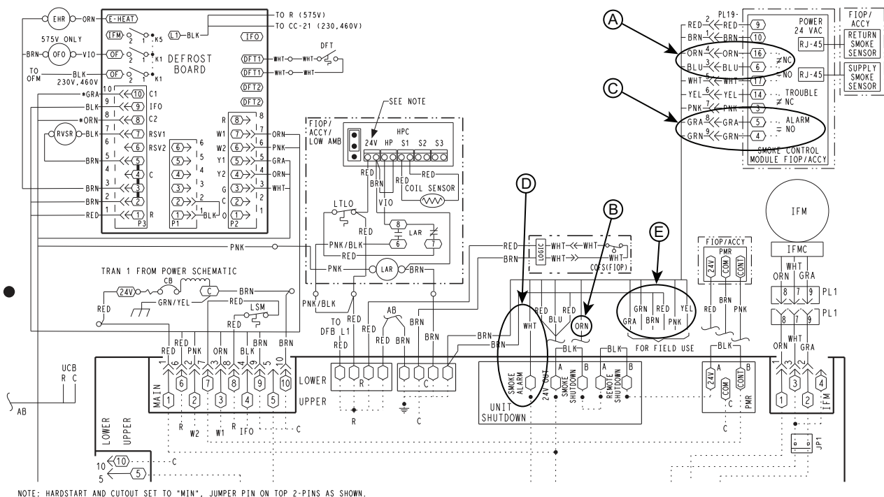
Fig. 46 — Typical Smoke Detector System Wiring
