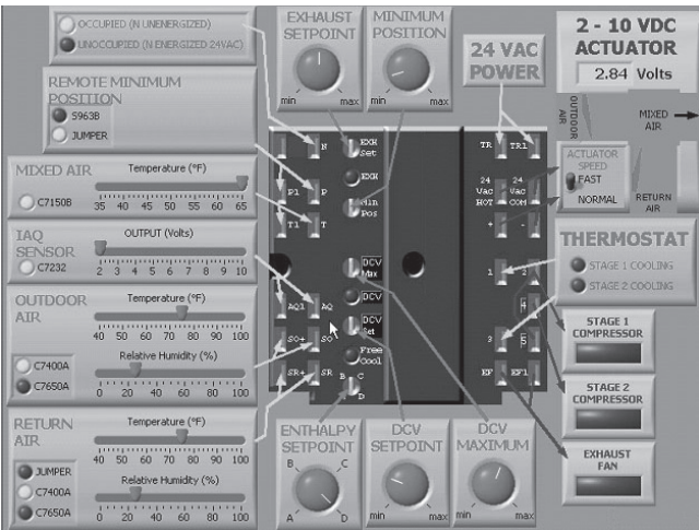
Fig. 56 — EconoMi$er IV Functional View
