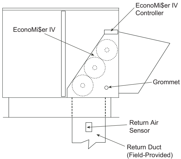
Fig. 62 — Return Air Temperature or Enthalpy Sensor Mounting Location
