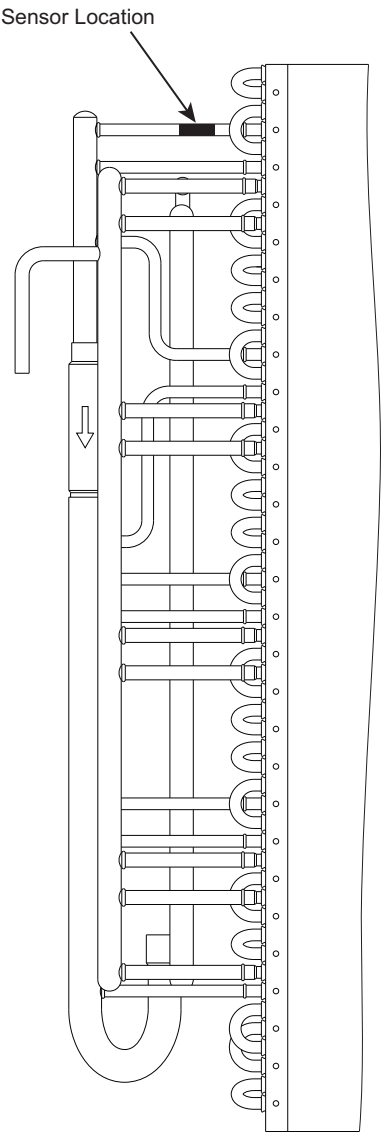
Fig. M — 50GCQ 04 Outdoor Circuiting
