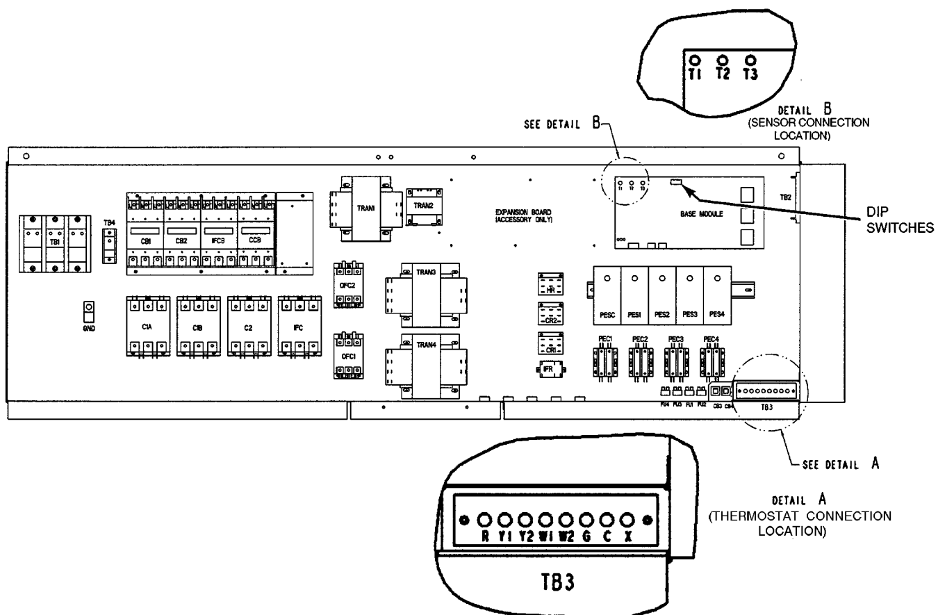
Fig. 15 — Control Box Diagram (Size 044)
