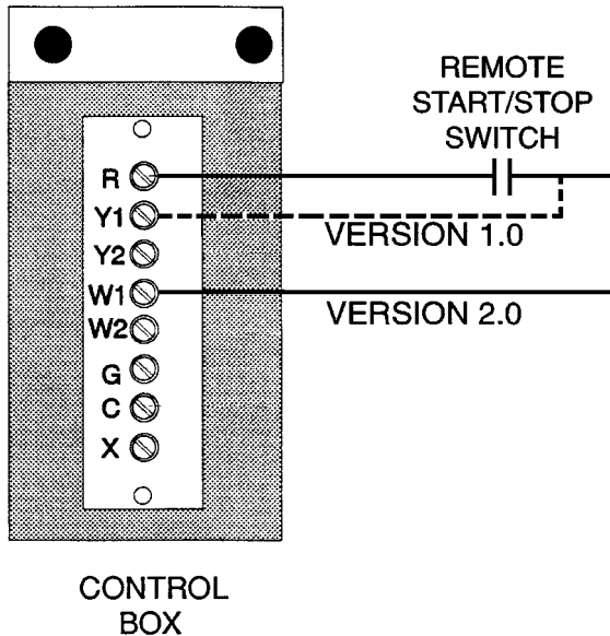
Fig. 11 — Field Control Remote Start/Stop (CV or VAV Units)
