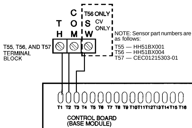
Fig. 17 — Field Control Temperature Sensor Wiring
