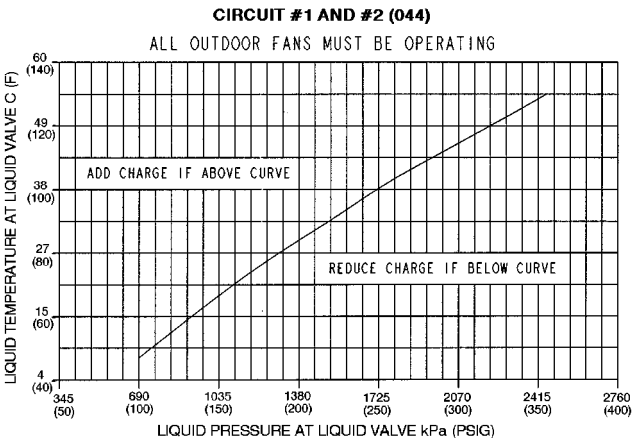
Fig. 42 — Cooling Charging Chart, Size 044
