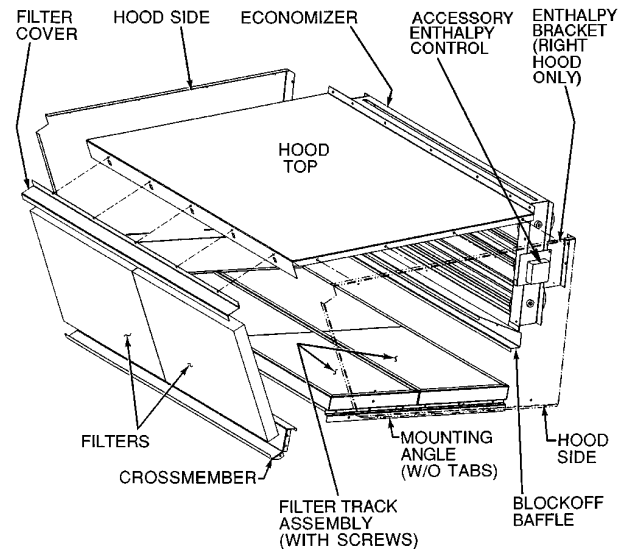
Fig. 19 — Economizer Hood Assembly (Right-Side Economizer Hood Shown)
