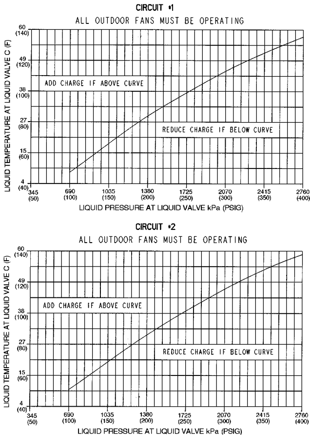
Fig. 41 — Cooling Charging Chart, Sizes 024-034
