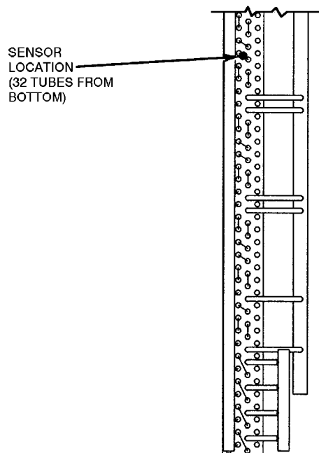
Fig. 33B — Motormaster III Sensor Location (Size 044)
