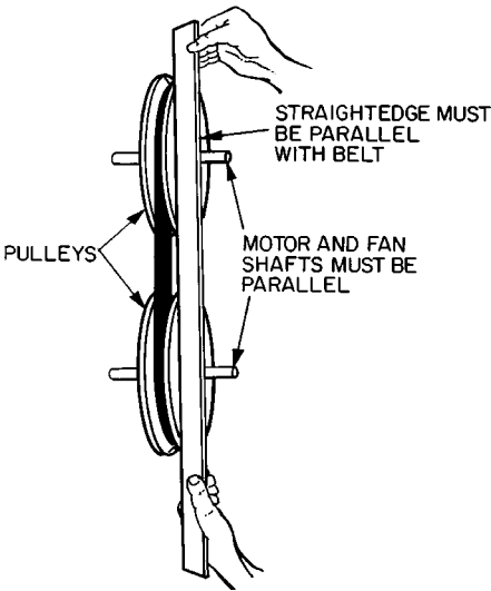
Fig. 38 — Evaporator-Fan Pulley Alignment and Adjustment
