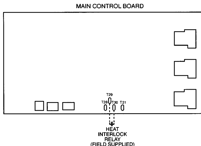
Fig. 35 — Heat Interlock Relay Wiring
