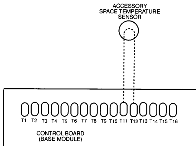
Fig. 36 — Space Temperature Sensor Wiring
