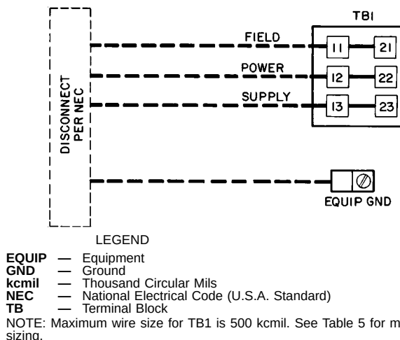
Fig. 13 — Field Power Wiring Connections
