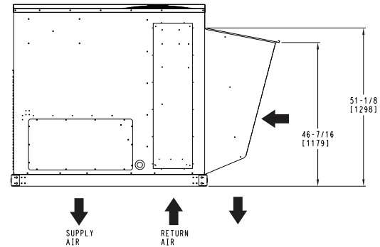
HORIZONTAL ECONOMIZER
