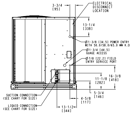
LEFT SIDE VIEW (FOR 38AXZ SYSTEMS)
