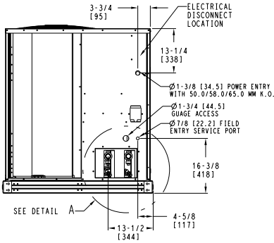
LEFT SIDE VIEW (FOR 38AXD/38AXQ SYSTEMS)
