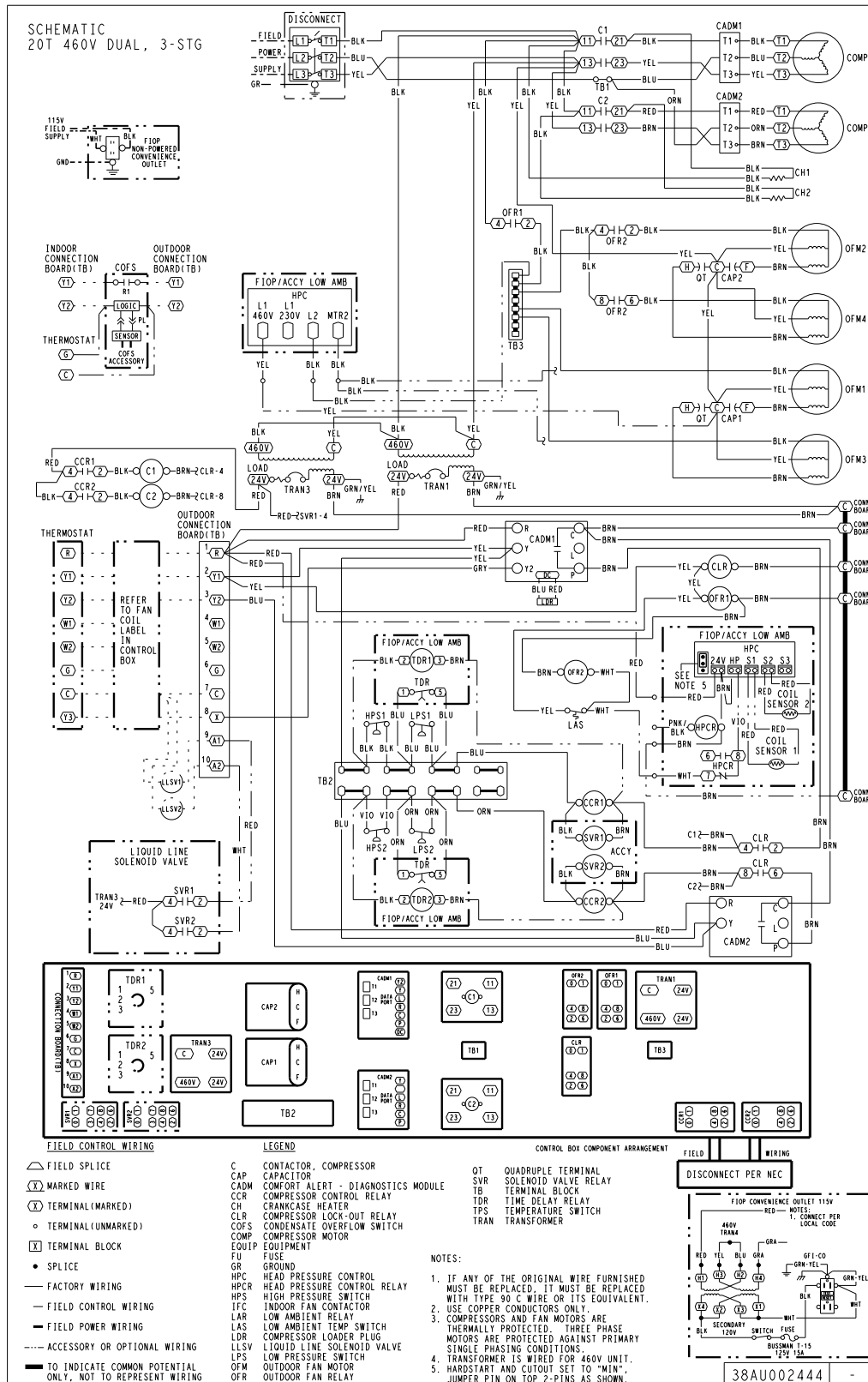
Typical Dual Circuit/Three Stage Wiring Diagram, 20 Ton (460-3-60 Unit Shown)
