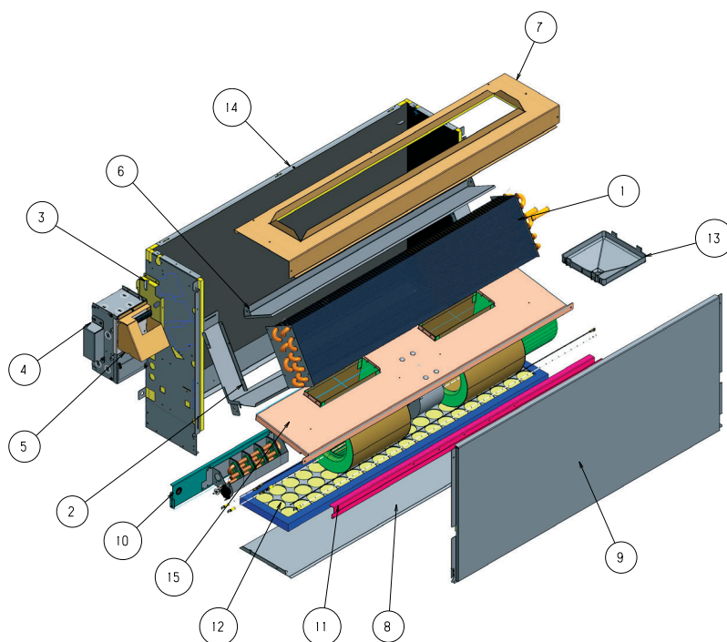
Fig. 39 — 42VAD Vertical Floor Top Supply With Optional Electric Heat (Exploded View)
