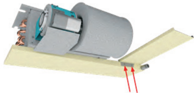
Fig. 60 — Left-Hand Extension Drip Lip
