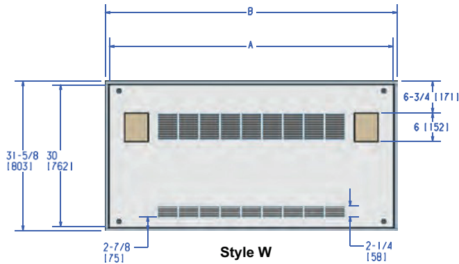
Fig. 68 — Style W Framed Wall Panel
