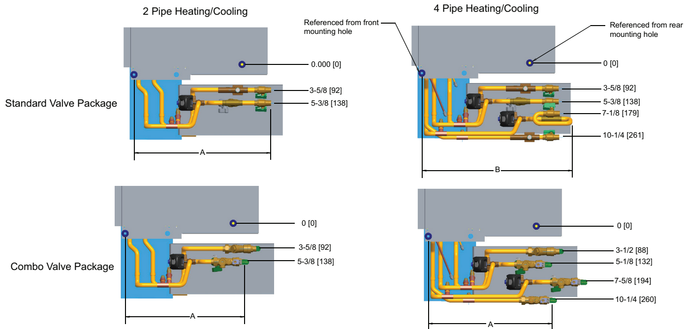
Partial Top View of 42CA/CE Units
