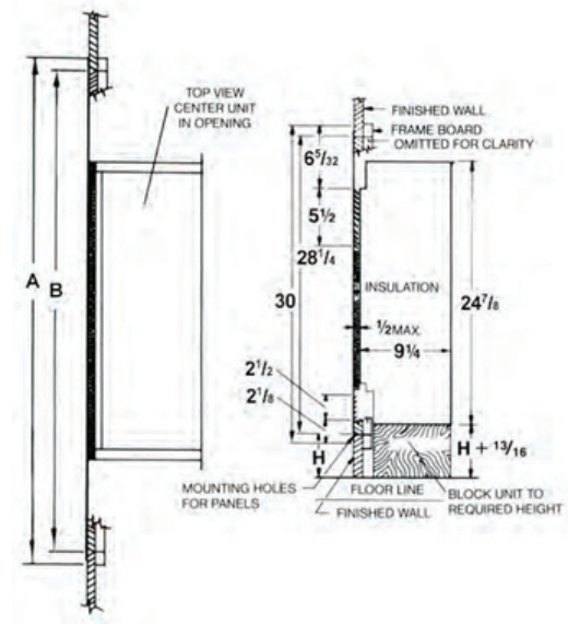
Fig. 70 — Style W Framed Wall Panel Install Diagram
