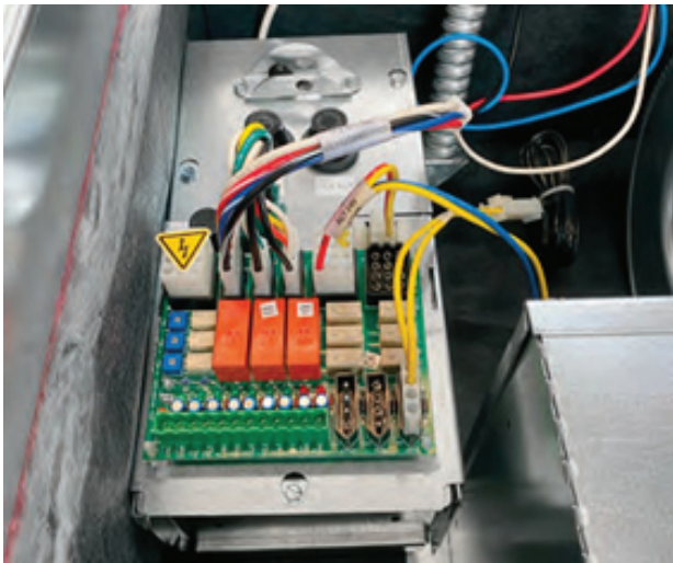
Fig. 83 — Unit-Mounted Control Box Access
