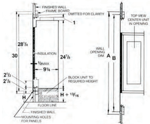
Fig. 71 — Style Z Framed Wall Panel Install Diagram
