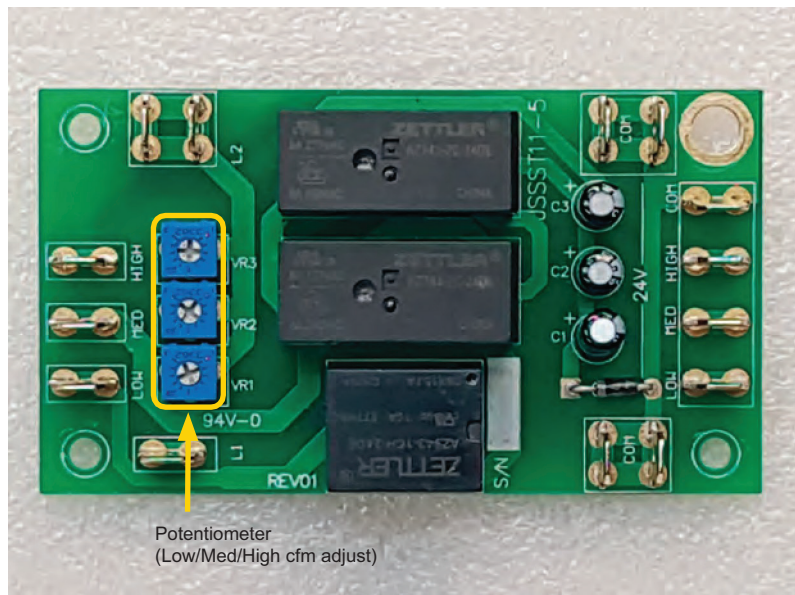
Fig. J — 3-Speed Pot Board
