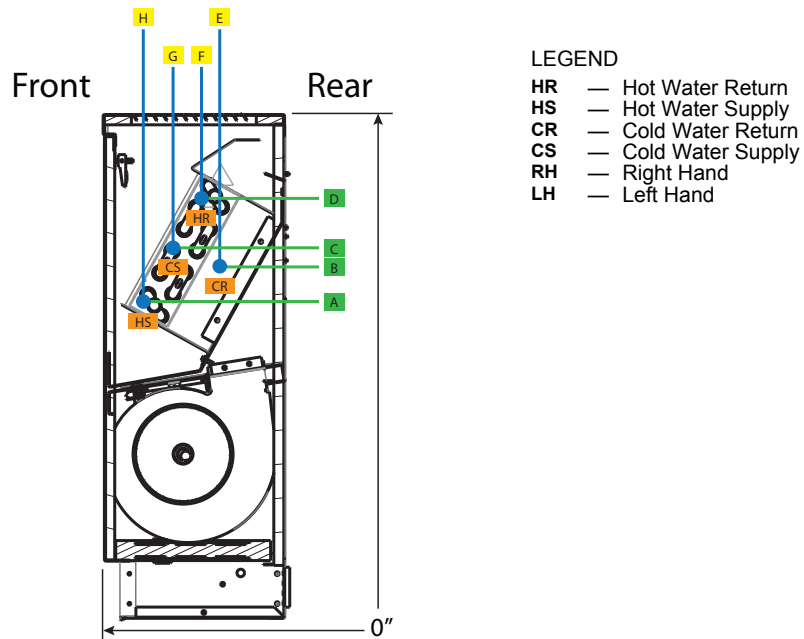
42V*D Hydronic Cooling and Heating Coil Dimensions a,b,c,d
