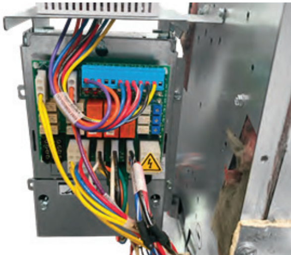
Fig. 83 — Unit-Mounted Control Box Access
