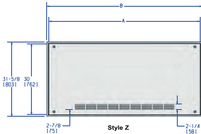
Fig. 69 — Style Z Framed Wall Panel
