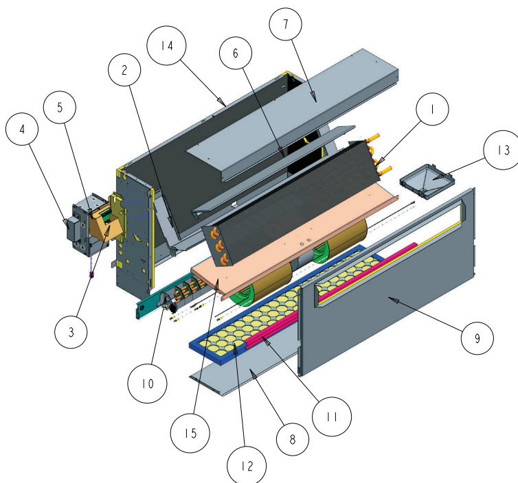
Fig. 41 — 42VAD Vertical Hideaway Front Supply With Optional Electric Heat (Exploded View)
