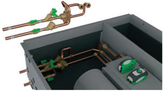
Fig. 59 — General Valve Package Assembly (CG Unit Shown)
