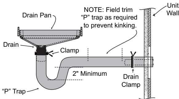
Fig. 77 — “P” Trap Minimum Configuration
