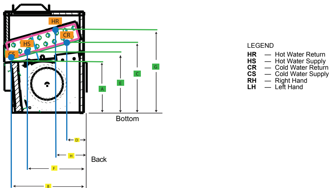
42VCA/VEA Hydronic Cooling and Heating Coil Dimensions a,b,c,d
