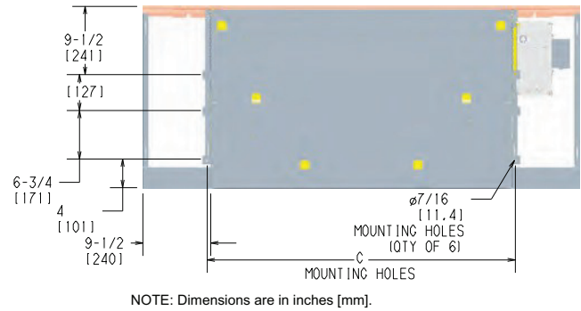
Fig. 67 — Wall Mount Hanger Hole Locations — 42VBD/VFD
