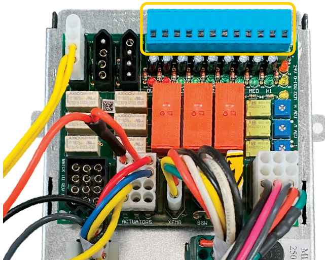
Fig. E — Thermostat Control Board (By Others or Remote Mounted)
