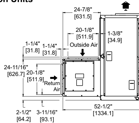
RIGHT SIDE
