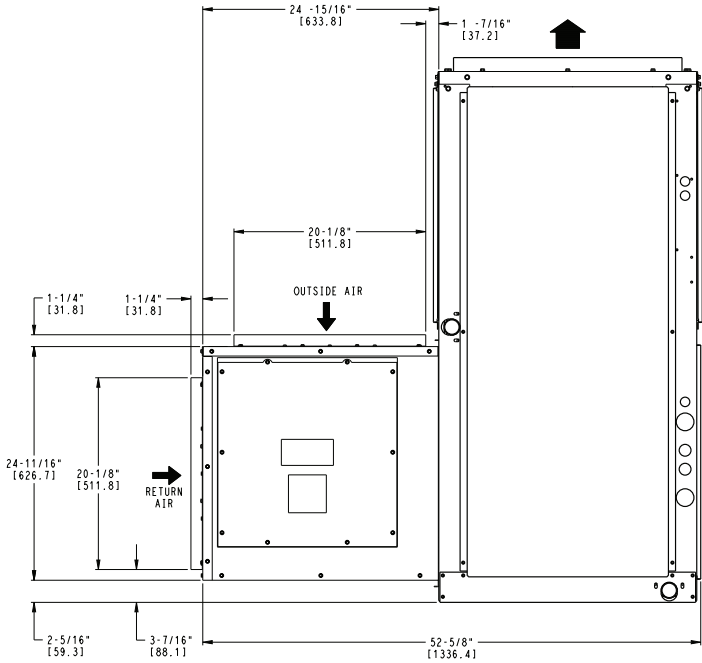
RIGHT SIDE
