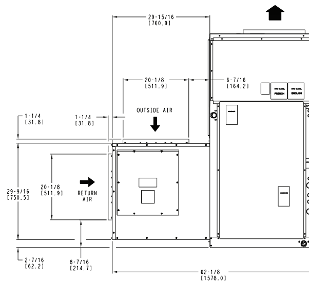
RIGHT SIDE
