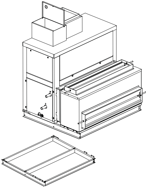
Top/Front Inlet Mixing Box
