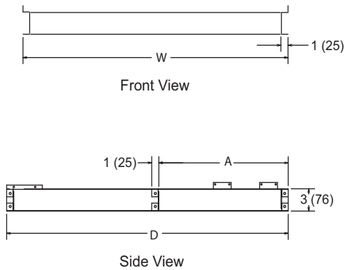
Base Rail Details
