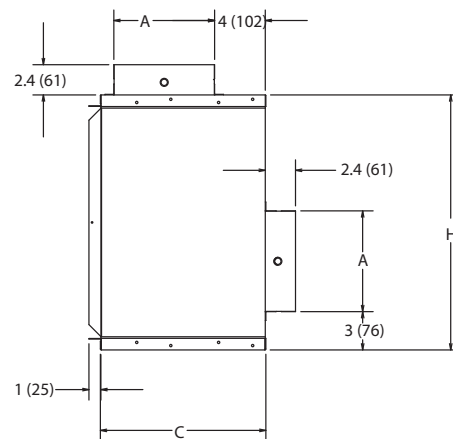
Top/Rear Inlet - DHA Top/Front Inlet - DVA
