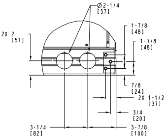
DETAIL C AT 2 PLCS
