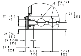
DETAIL B AT 2 PLCS
