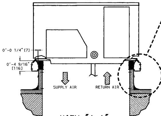
VIEW "A-A"
