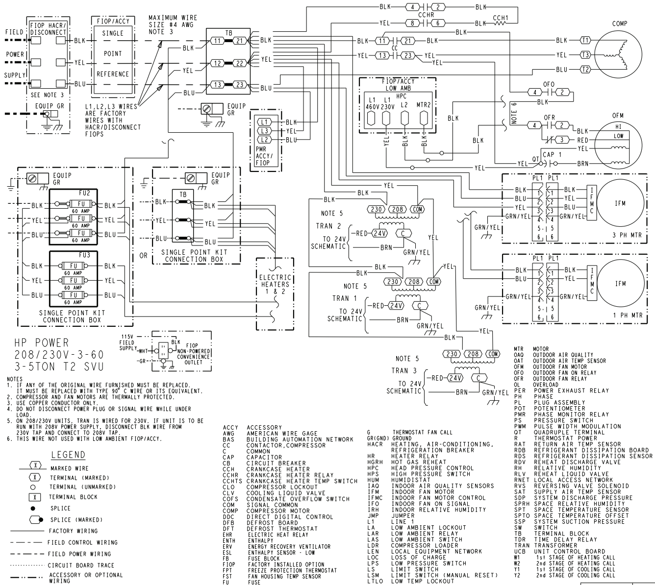
Typical 50GEQ 04-06 Power Wiring Diagram, SystemVu, 208/230-3-60 Shown
