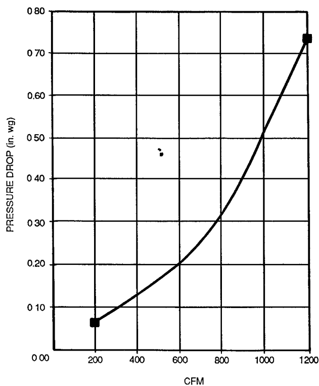
PARABLADE ECONOMIZER BAROMETRIC RELIEF DAMPER CHARACTERISTICS — 50TJ008-014
