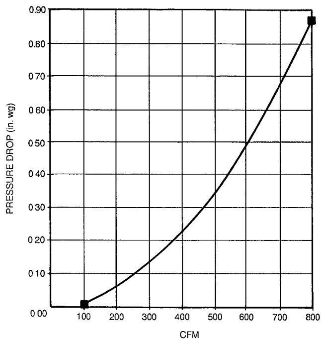
PARABLADE ECONOMIZER BAROMETRIC RELIEF DAMPER CHARACTERISTICS — 50TJ004-007
