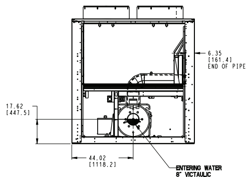
1 PASS EVAPORATOR (“I” IN MODEL NUMBER POSITION 12)
