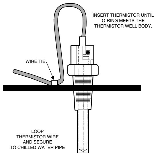
Fig. 50 — Dual Chiller Accessory Kit Leaving Water Thermistor and Well (Part No. 00EFN900044000A)
