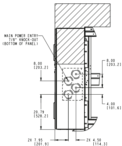
DETAIL B FROM SHEET #1 (TOP VIEW- KNOCK OUTS ON BOTTOM OF CONTROL BOX)
