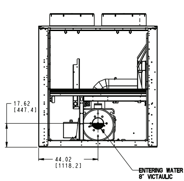
1 PASS EVAPORATOR ("I" IN MODEL NUMBER POSITION 12)
