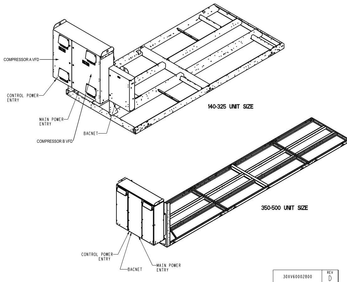
Fig. 48 — Field Control and Power Wiring (cont)
