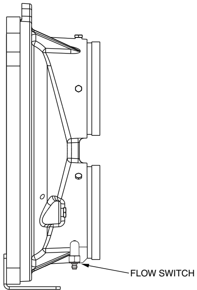
Fig. 38 — Flow Switch Location
