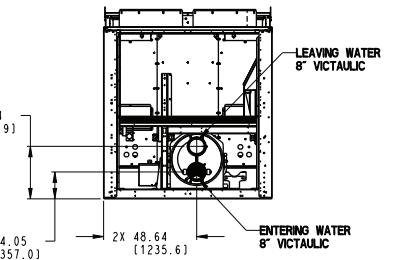
STANDARD PASS EVAPORATOR (“-” AND “0” IN MODEL NUMBER POSITION 12)
