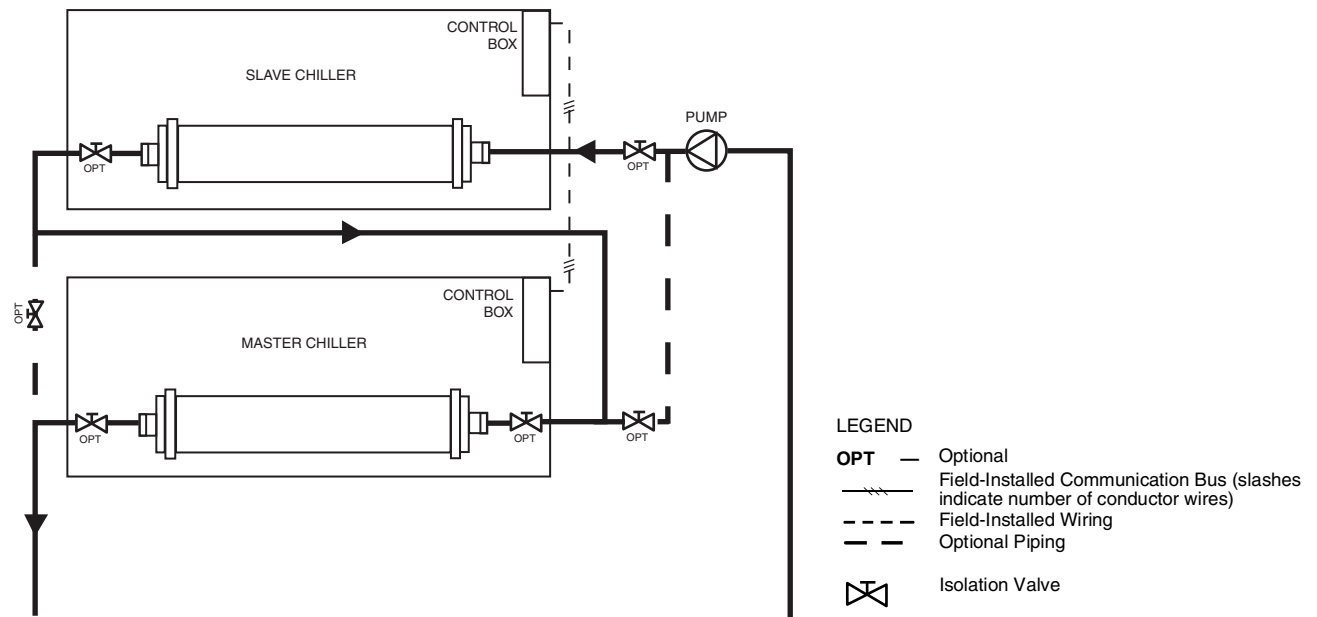
Fig. 43 — Series Dual Chiller Operation
