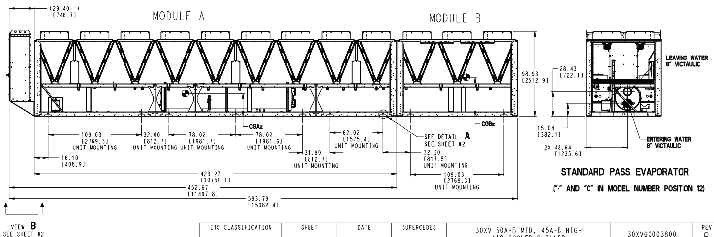
Fig. 24 — 30XV Split Unit 45A-B High, 50A-B Mid Tier Air-Cooled Chiller
