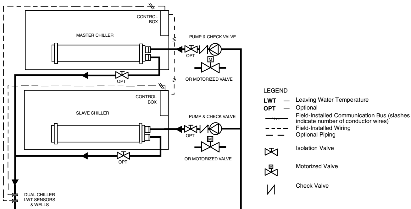
Fig. 42 — Parallel Dual Chiller Operation
