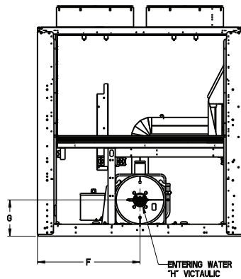
1 PASS EVAPORATOR (1" IN MODEL NUMBER POSITION 12)
