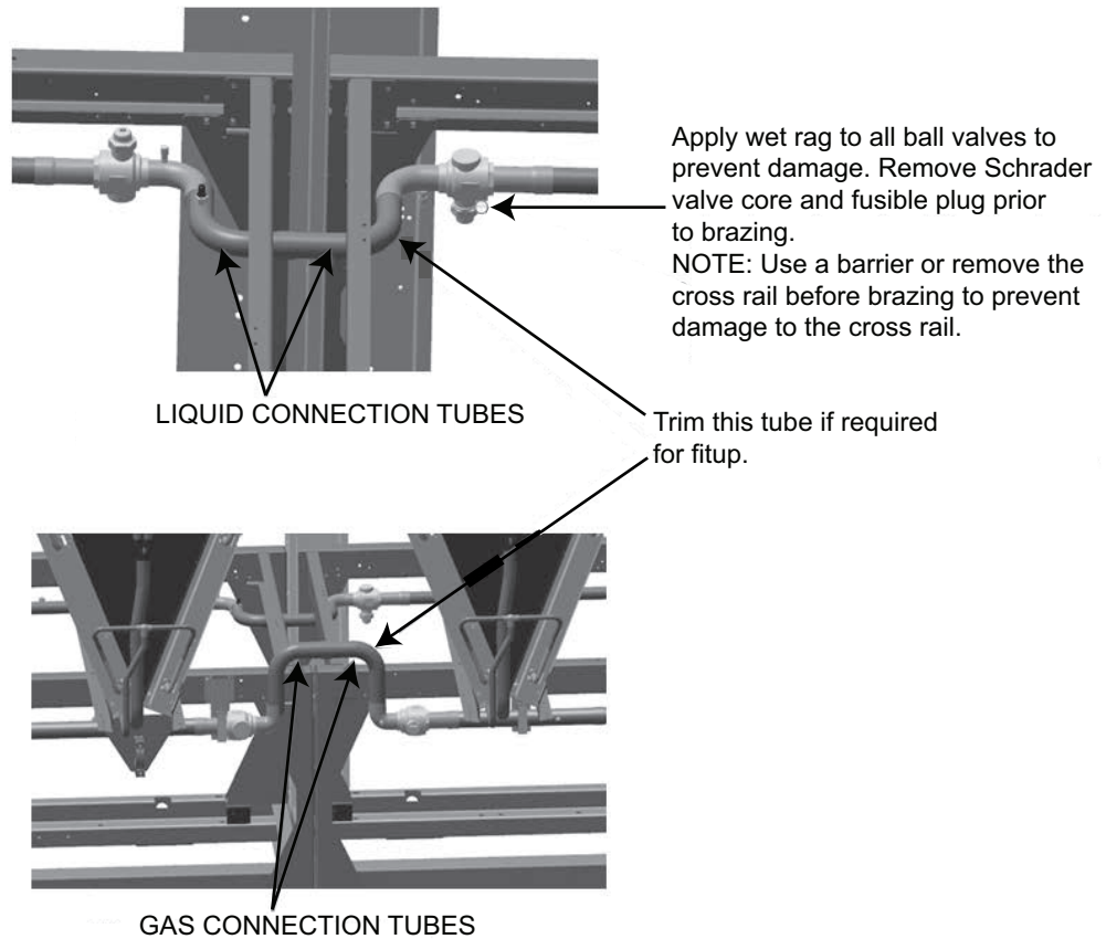
Fig. 32 — Brazing Gas and Liquid Lines
