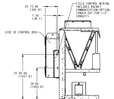
DETAIL A AT (10) PLCS FROM SHEET #1
