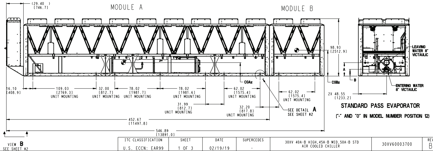
Fig. 23 — 30XV Split Unit 40A-B High, 45A-B Mid, 50A-B Standard Tier Air-Cooled Chiller
