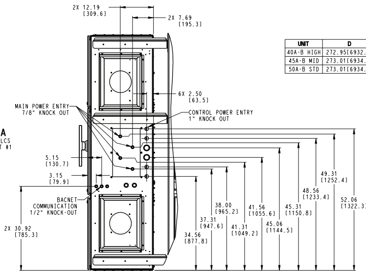
VIEW B FROM SHEET #1
