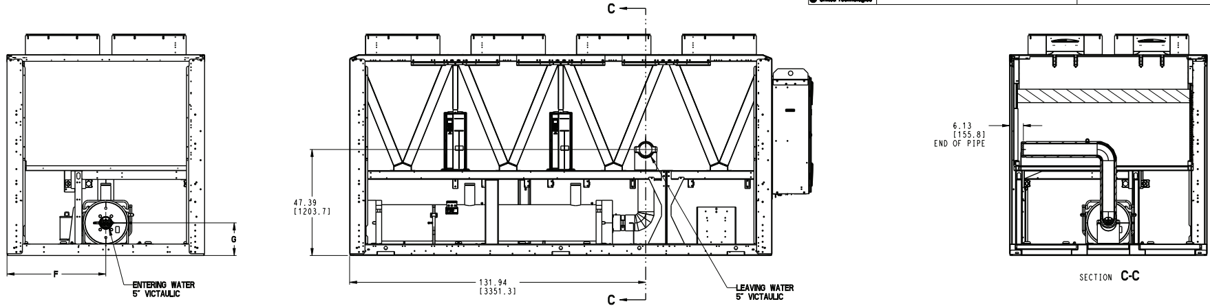
1 PASS EVAPORATOR (“I” IN MODEL NUMBER POSITION 12)
