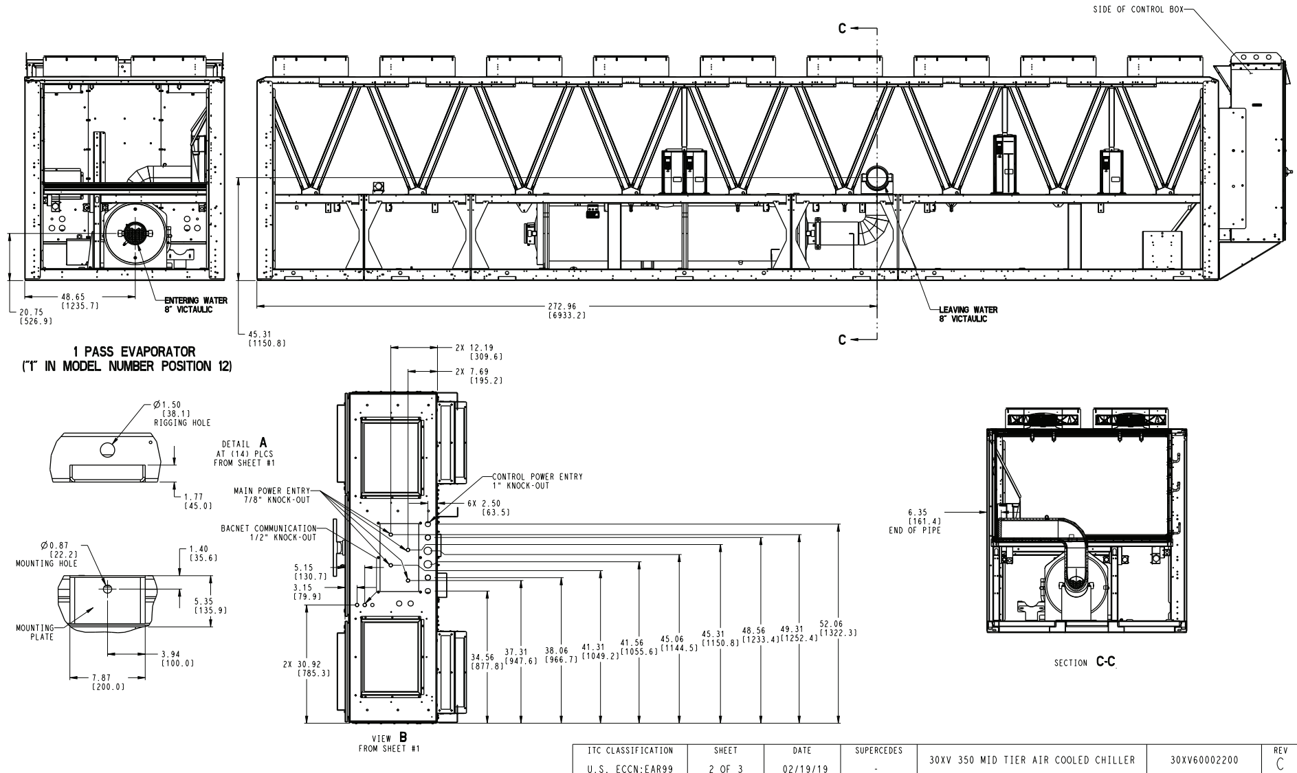
Fig. 17 — 30XV 350 Mid Tier Air-Cooled Chiller (cont)
