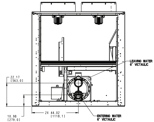
BRINE EVAPORATOR (\"2\" IN MODEL NUMBER POSITION 12)
