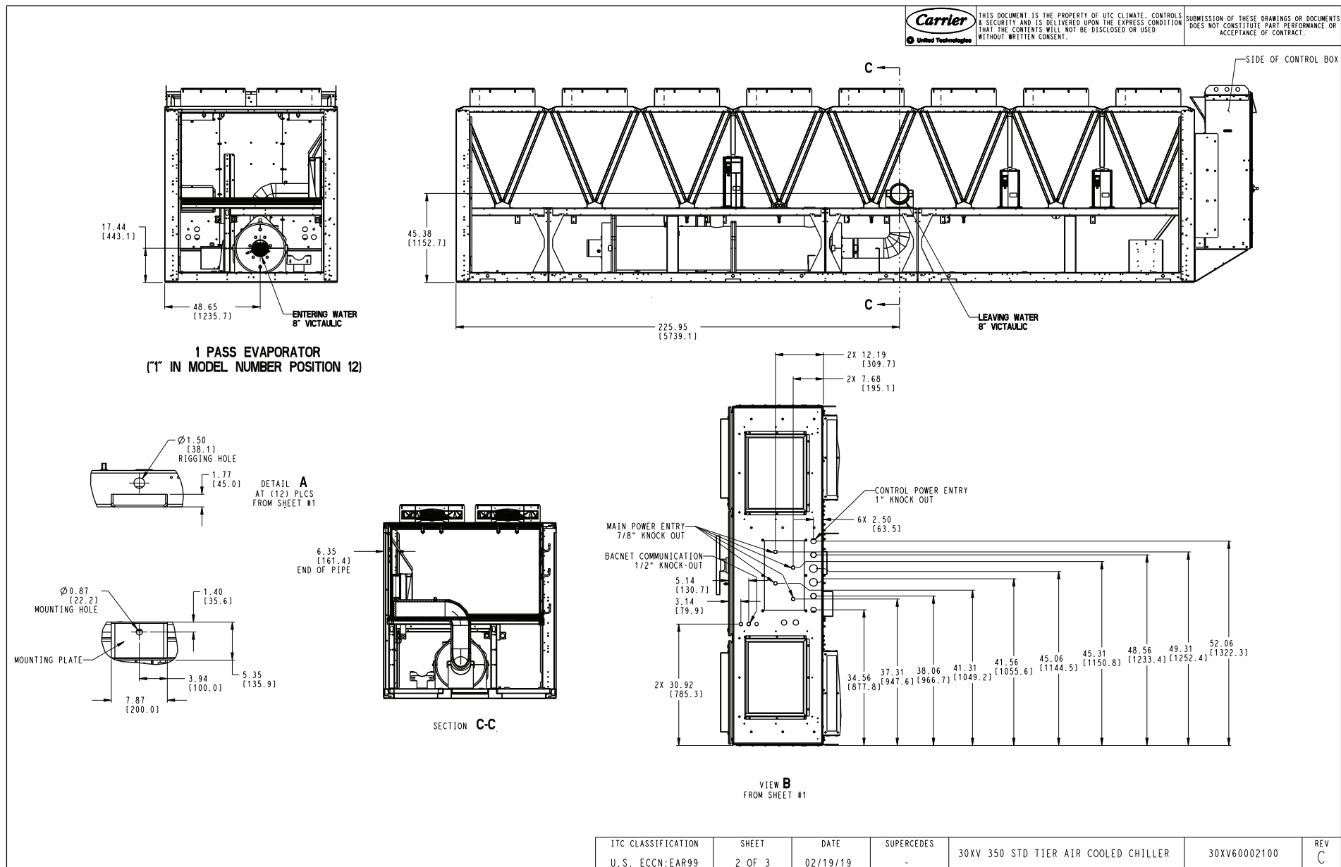
Fig. 16 — 30XV 350 Standard Tier Air-Cooled Chiller (cont)
