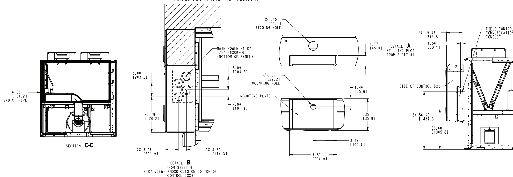
1 PASS EVAPORATOR (“I” IN MODEL NUMBER POSITION 12)
