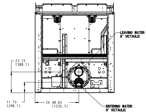
BRINE EVAPORATOR ("2" IN MODEL NUMBER POSITION 12)
