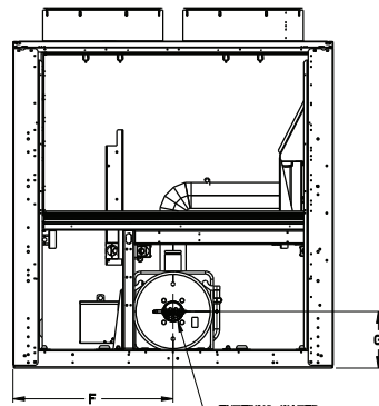
1 PASS EVAPORATOR (“T” IN MODEL NUMBER POSITION 12)
