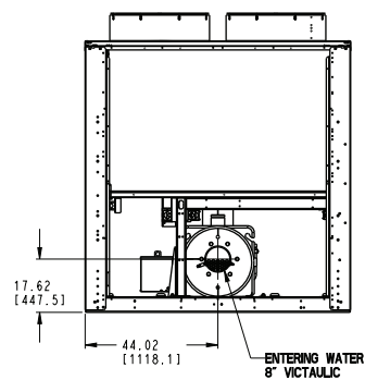
1 PASS EVAPORATOR ("I" IN MODEL NUMBER POSITION 12)
