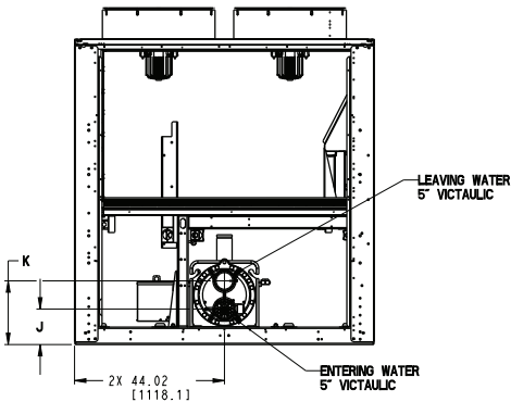
BRINE EVAPORATOR (2" IN MODEL NUMBER POSITION 12)
