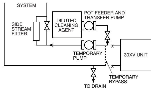
Fig. 47 — Cleaning Using a Side Stream Filter
