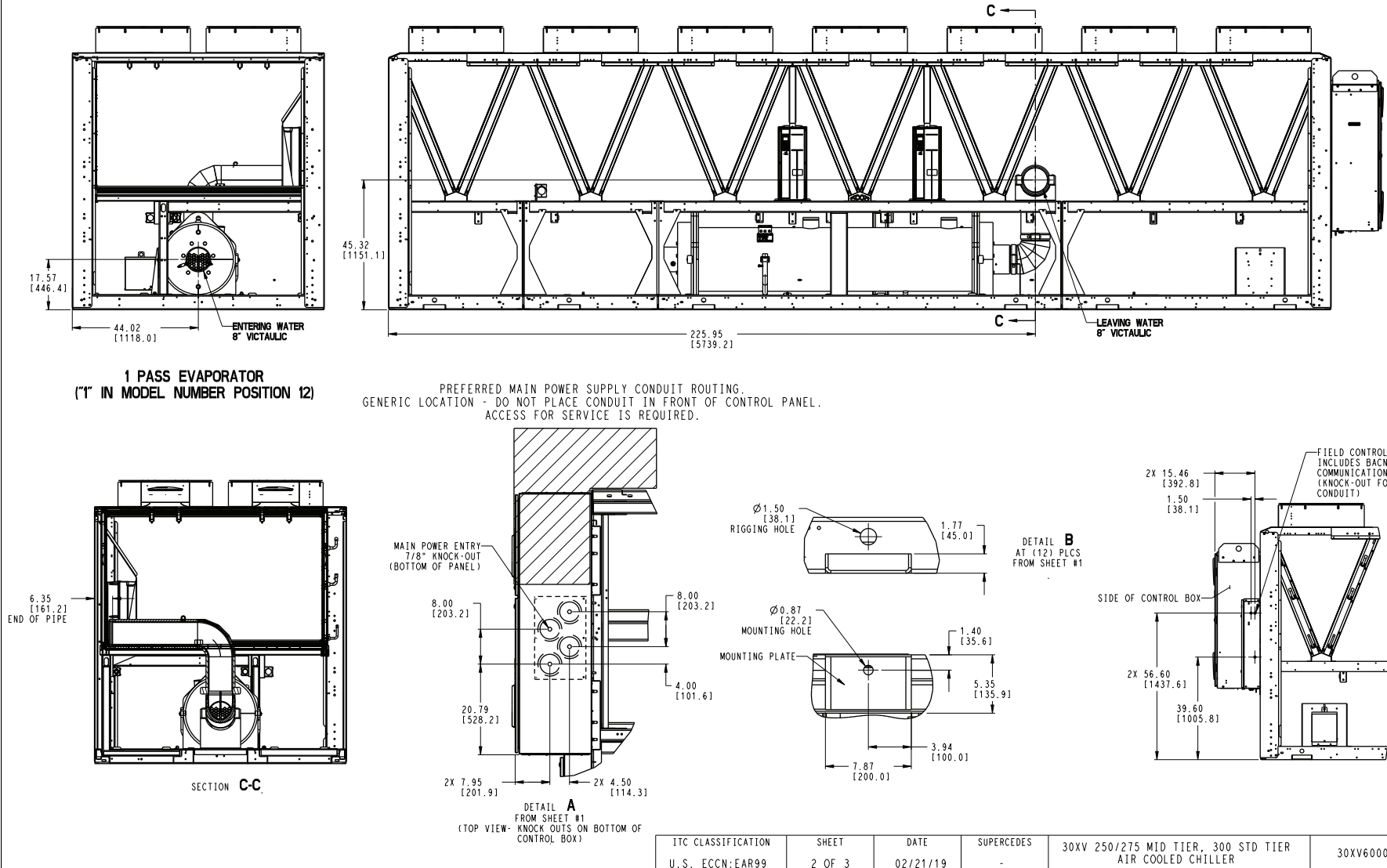
Fig. 12 — 30XV 250,275 Mid Tier; 300 Std Tier Air-Cooled Chiller (cont)
