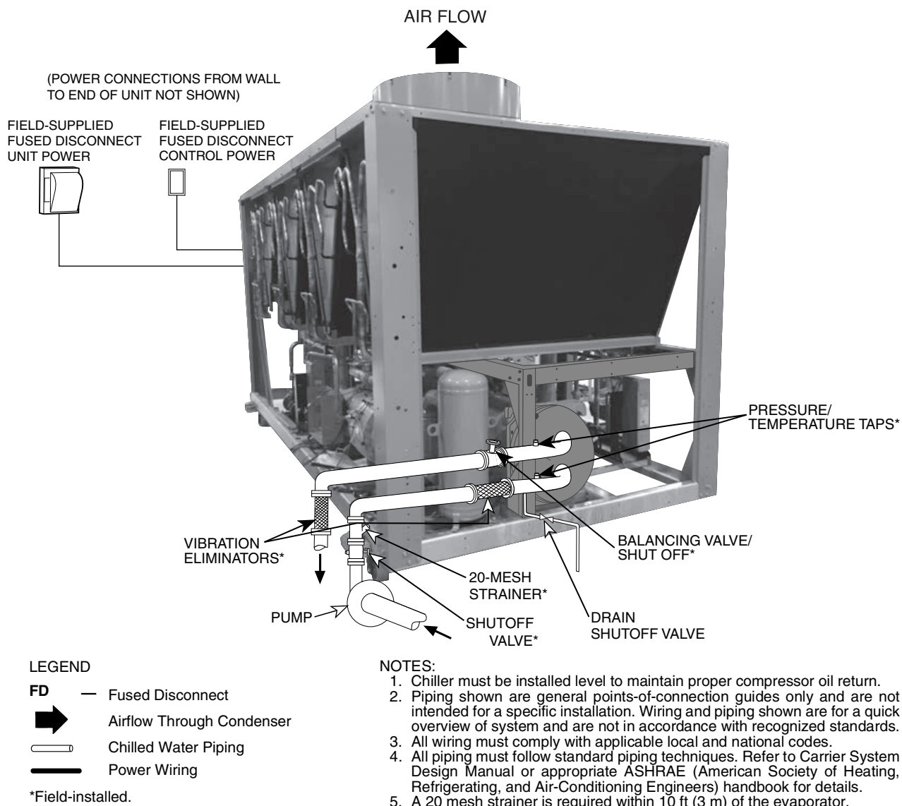
Fig. 37 — 30XV Typical Piping and Wiring
