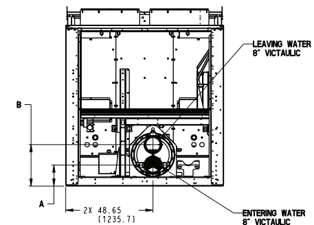
BRINE EVAPORATOR (2" IN MODEL NUMBER POSITION 12)
