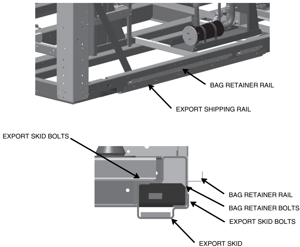
Fig. 26 — Export Shipping Rails
