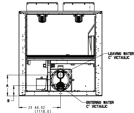
BRINE EVAPORATOR ("2" IN MODEL NUMBER POSITION 12)
