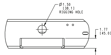
DETAIL A AT (B) PLCS FROM SHEET #1
