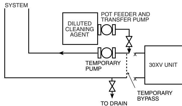
Fig. 46 — Typical Set Up for Cleaning Process
