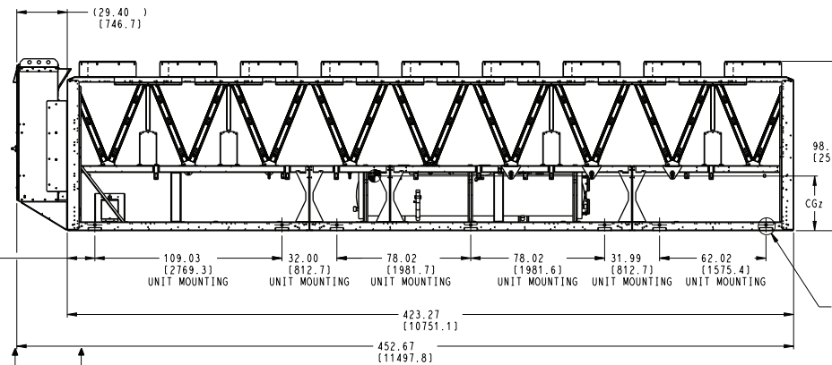
VIEW B SEE SHEET #2
