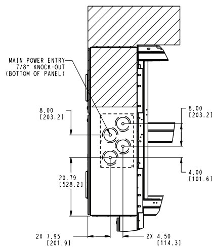
DETAIL B FROM SHEET #1 (TOP VIEW- KNOCK-OUTS ON BOTTOM OF CONTROL BOX)
