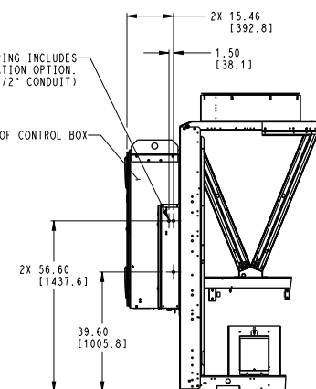
DETAIL A AT (10) PLCS FROM SHEET #1
