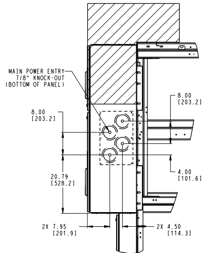
DETAIL A FROM SHEET #1 (TOP VIEW- KNOCK OUTS ON BOTTOM OF CONTROL BOX)
