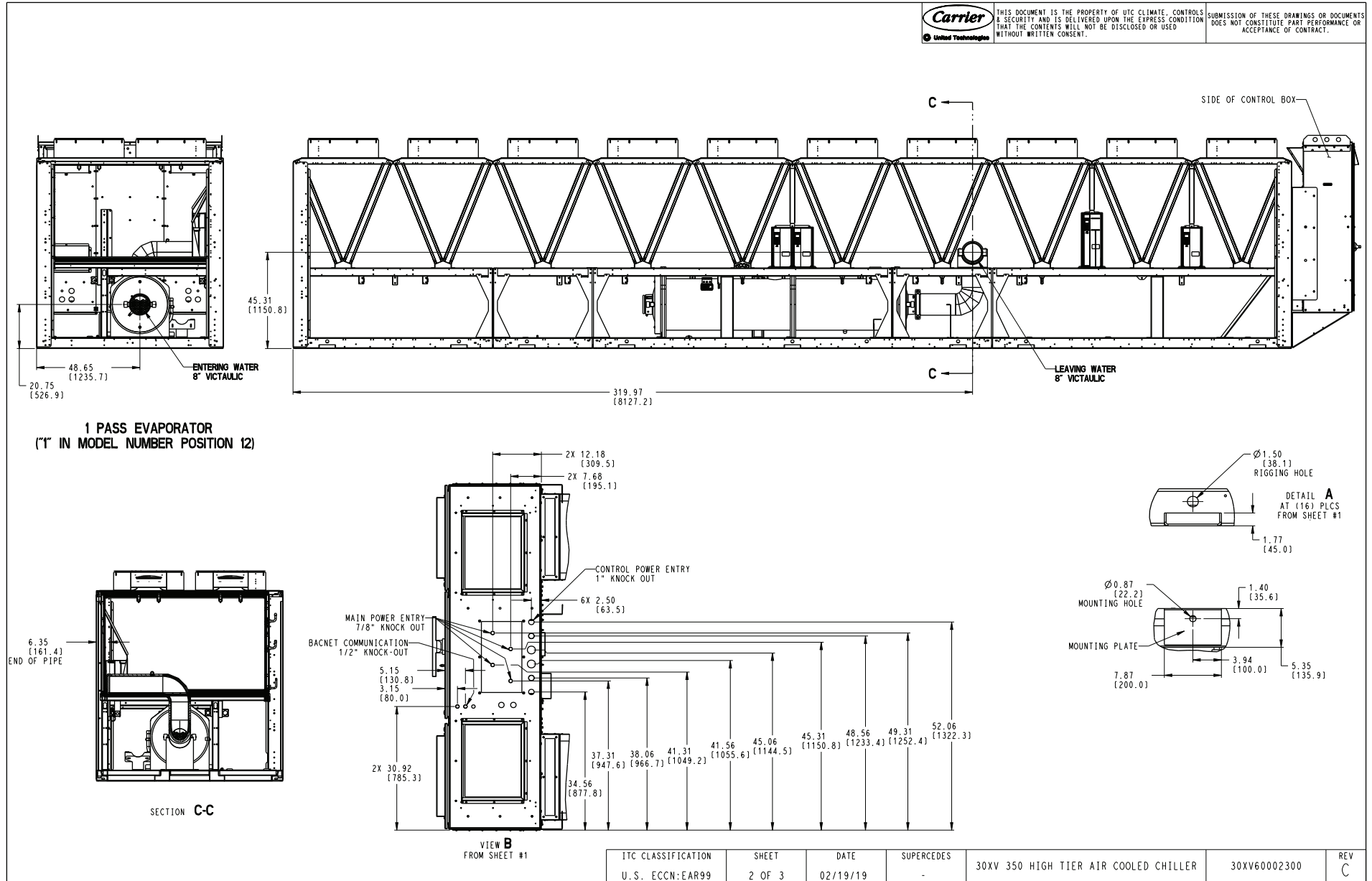
Fig. 18 — 30XV 350 High Tier Air-Cooled Chiller (cont)
