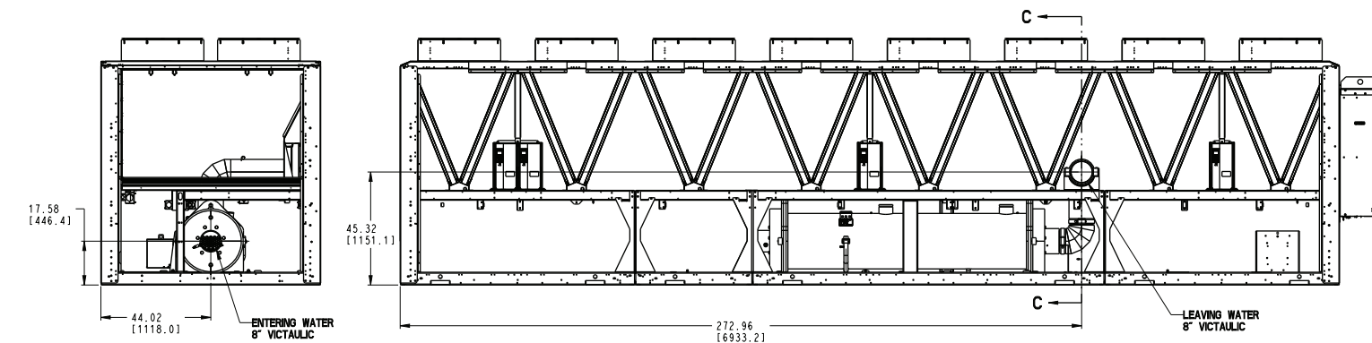
1 PASS EVAPORATOR (“I” IN MODEL NUMBER POSITION 12)
