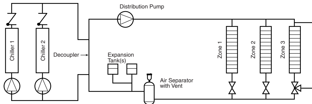
Fig. 40 — Typical Air Separator and Expansion Tank Location on Primary-Secondary Systems
