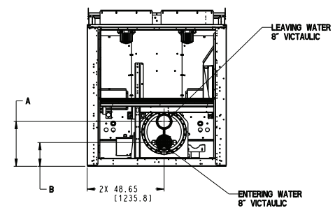
BRINE EVAPORATOR (2" IN MODEL NUMBER POSITION 12)
