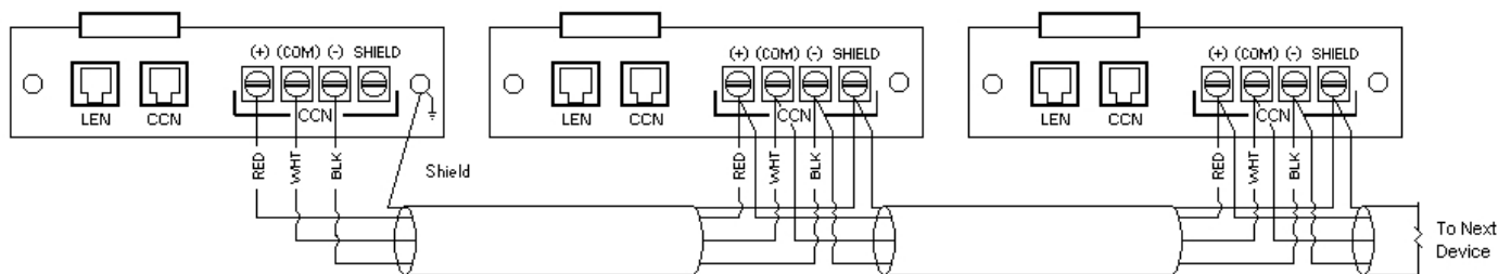
Fig. 3 — Typical CCN Bus Wiring
