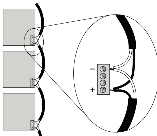
Fig. 4 — Typical BACnet MS/TP Bus Wiring
