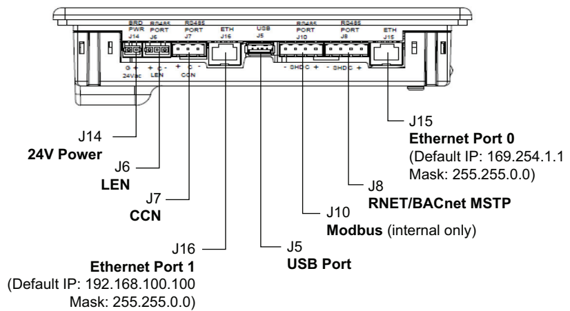
Fig. 2 — Carrier SmartVu™ Touchscreen Display Interface and Connections
