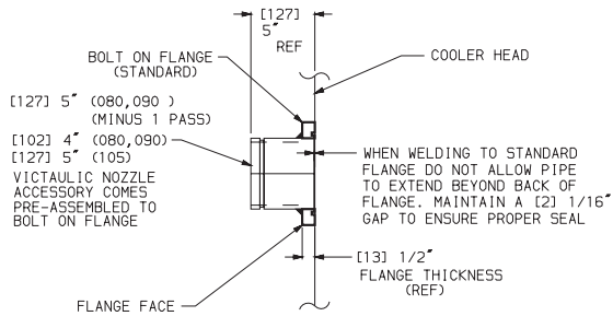
DETAIL "A" NOZZLE CONNECTIONS
