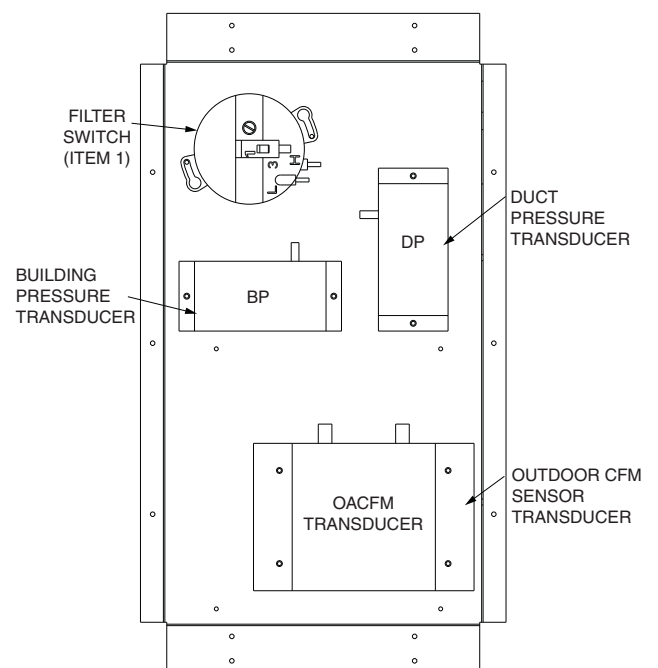
Fig. 7 — Auxiliary Control Box (48/50P030-050 and 48/50Z030-050)
