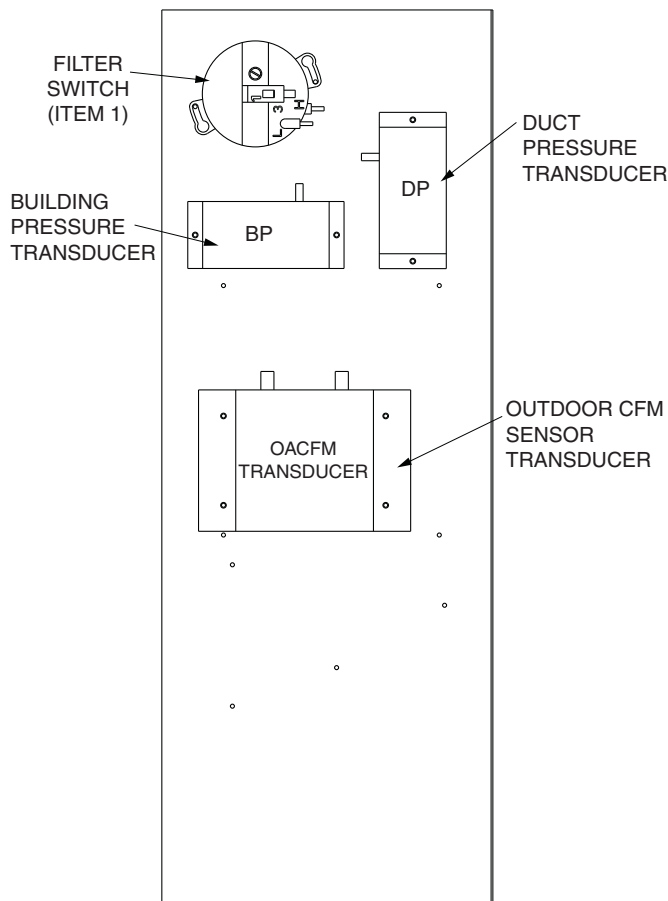
Fig. 8 — Auxiliary Control Box (48/50P055-100 and 48/50Z055-105)
